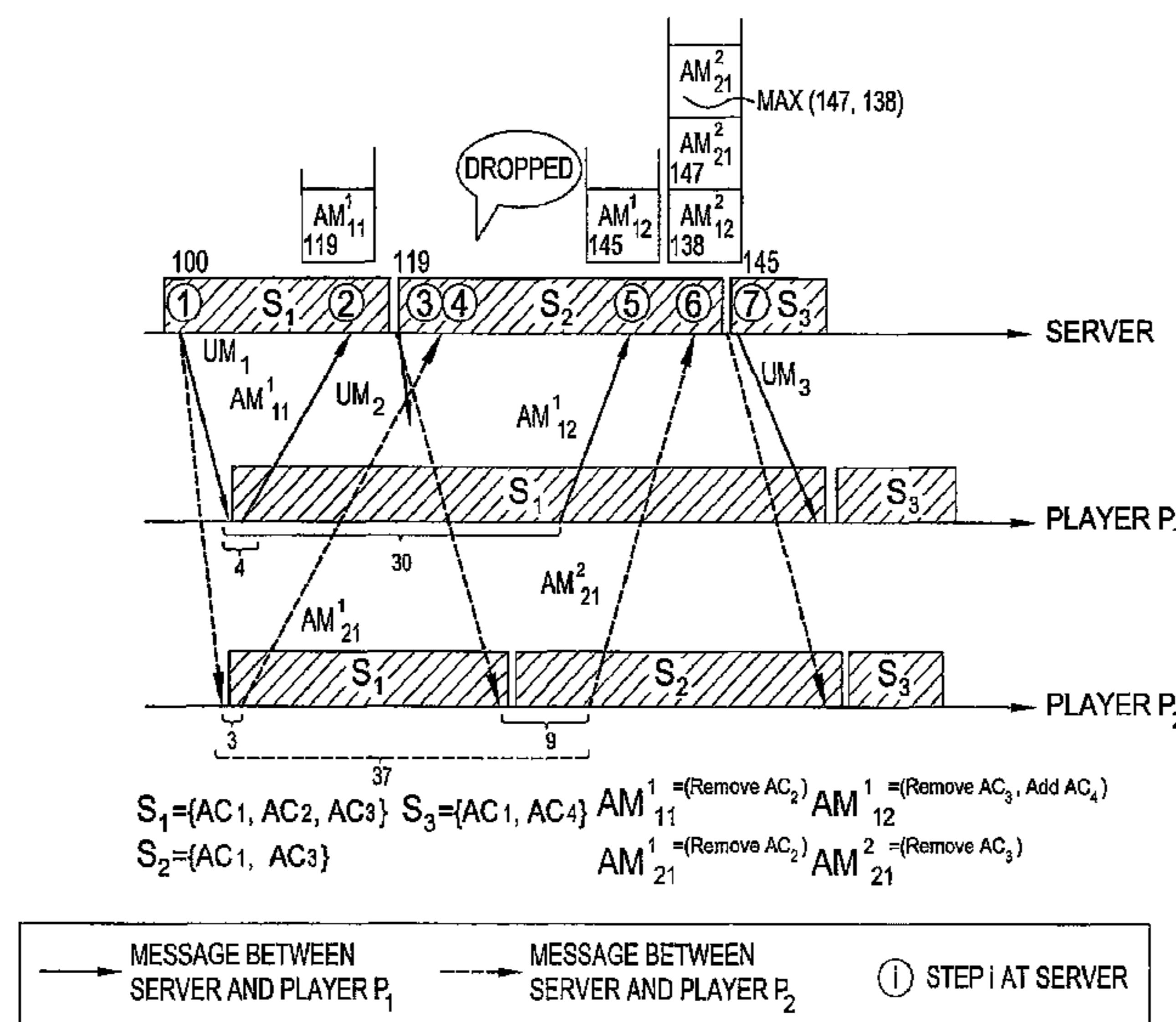
EXAMPLE SHOWING THE FAIR-ORDER MESSAGE DELIVERY ALGORITHM.
