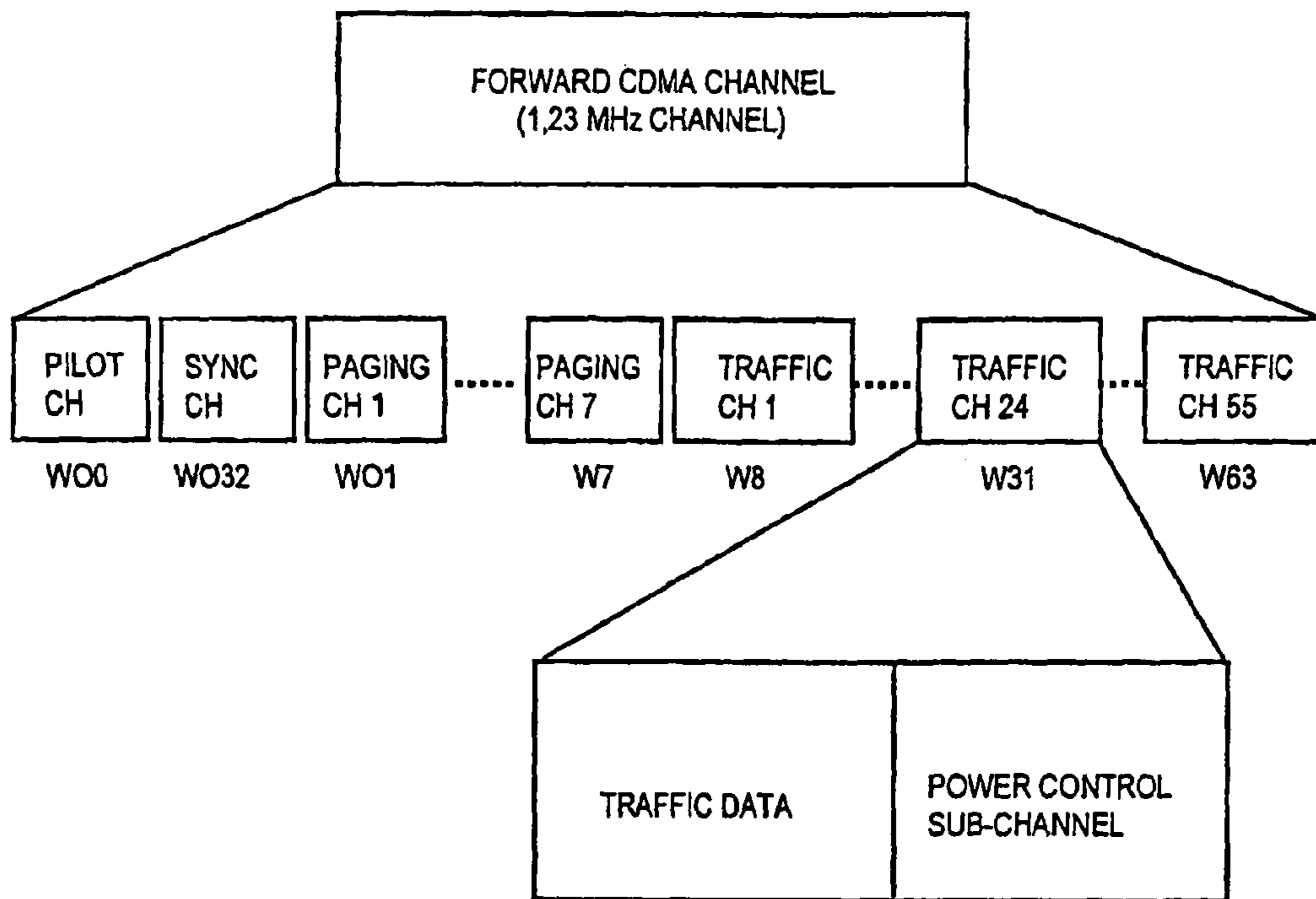
Fig. 1 PRIOR ART
