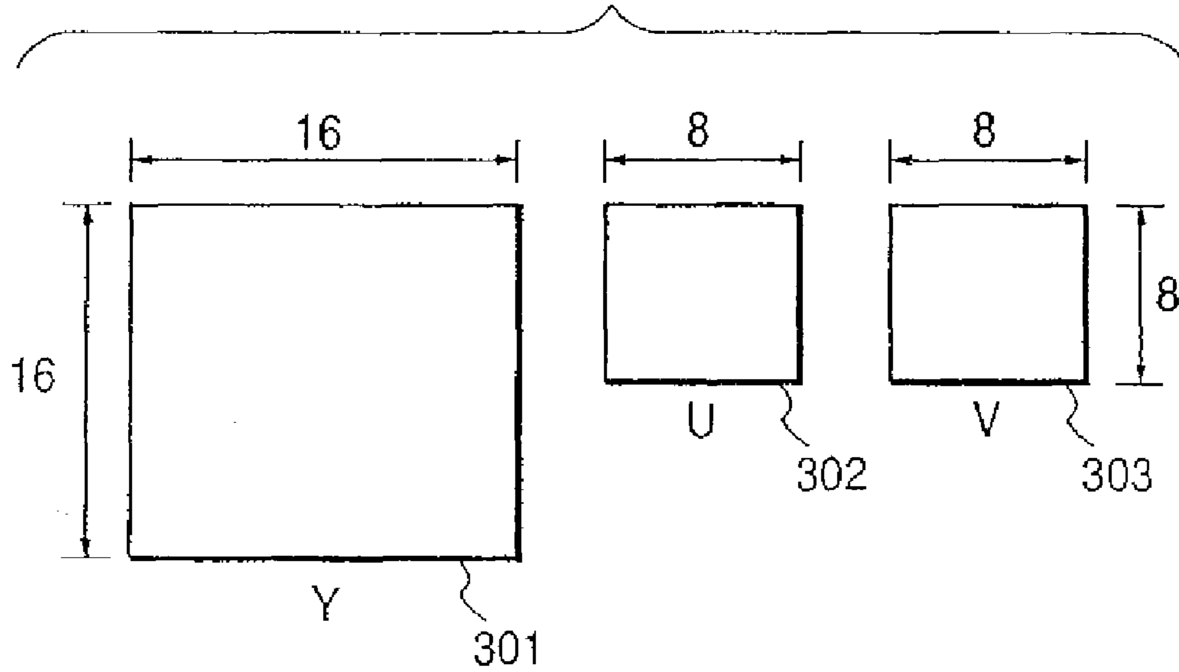
FIG. 3 (PRIOR ART)
