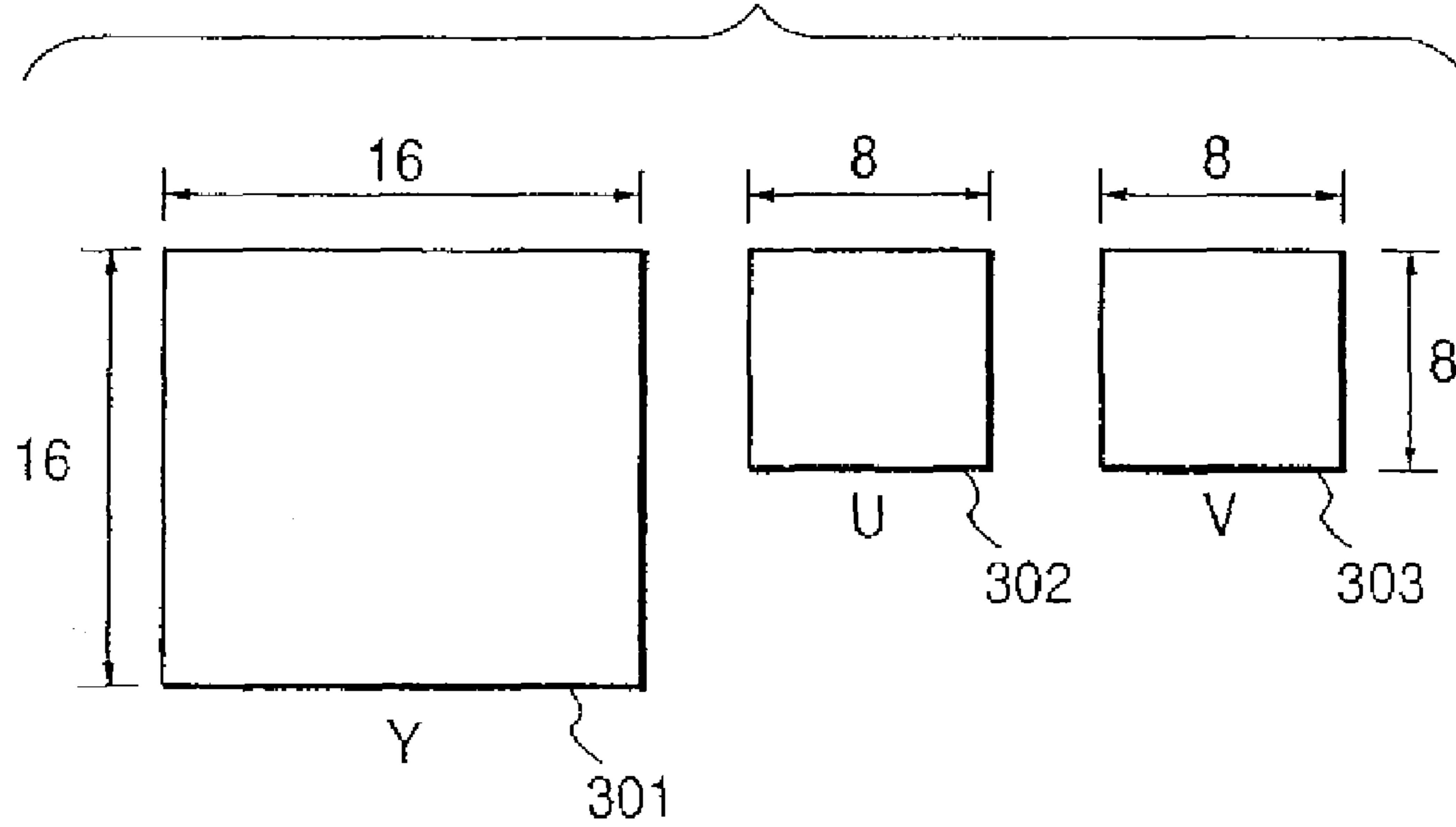
FIG. 3 (PRIOR ART)
