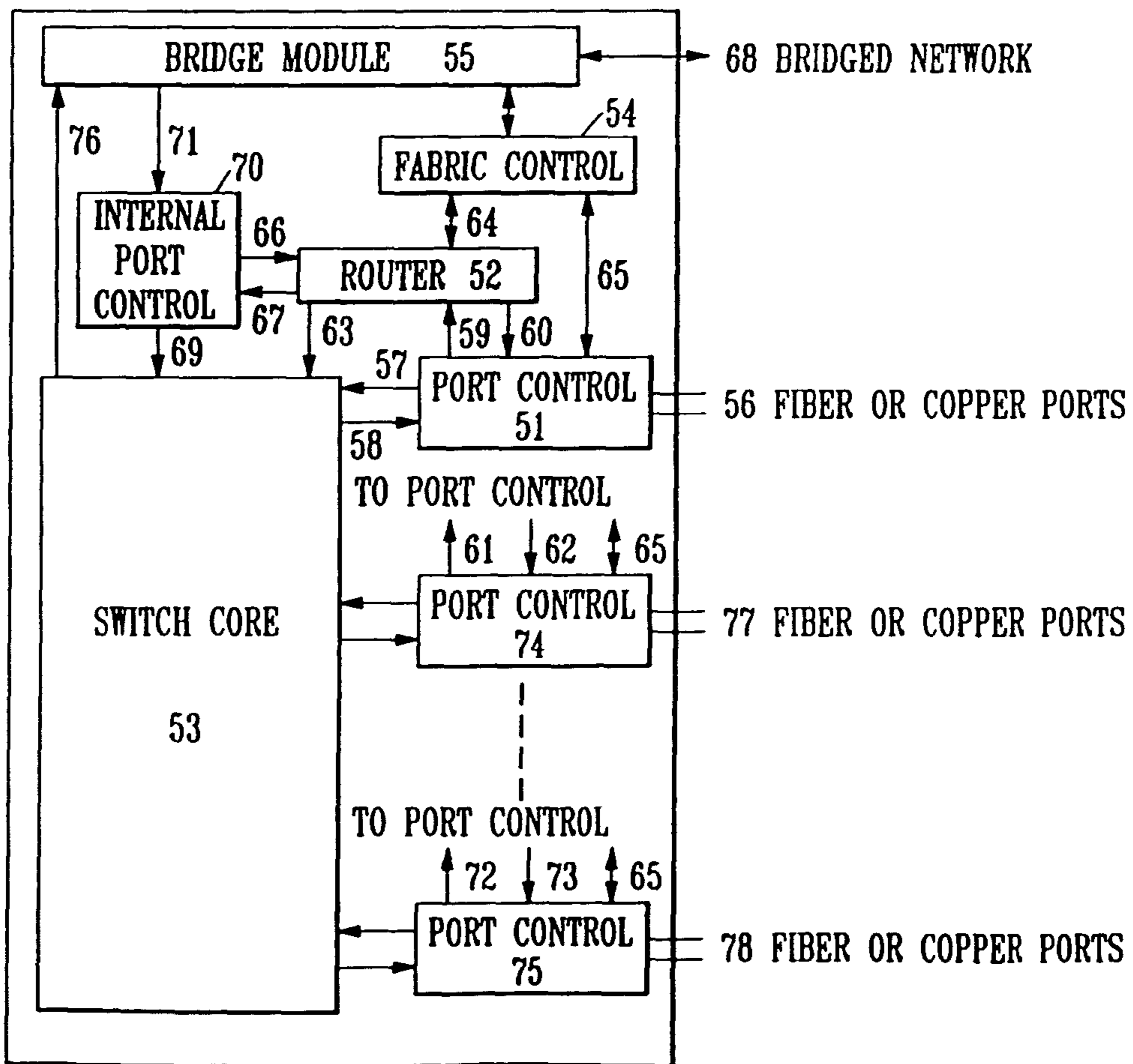
FIBRE CHANNEL FABRIC BLOCK DIAGRAM
