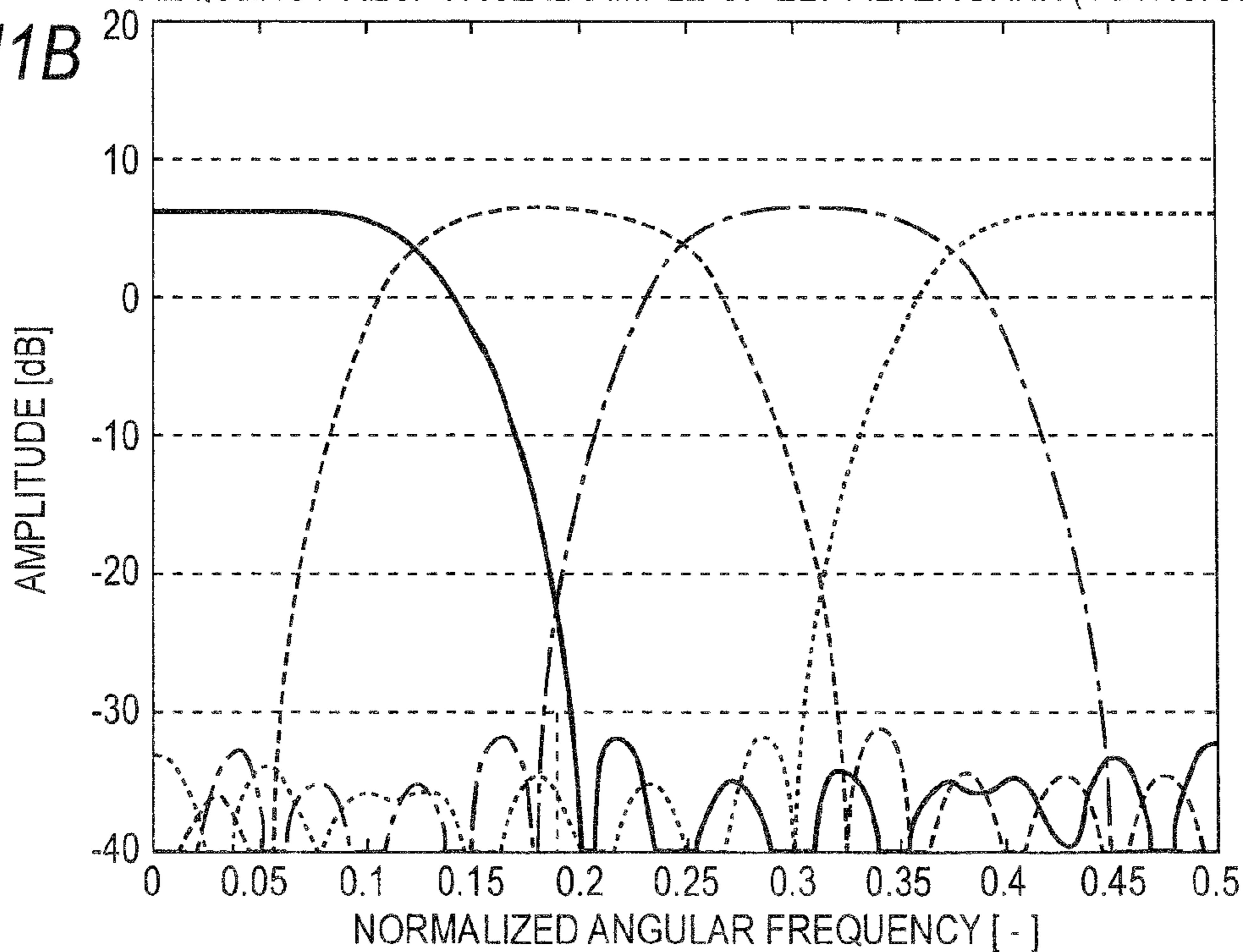
FREQUENCY RESPONSE EXAMPLE OF ELT FILTER BANK (4 DIVISION)
