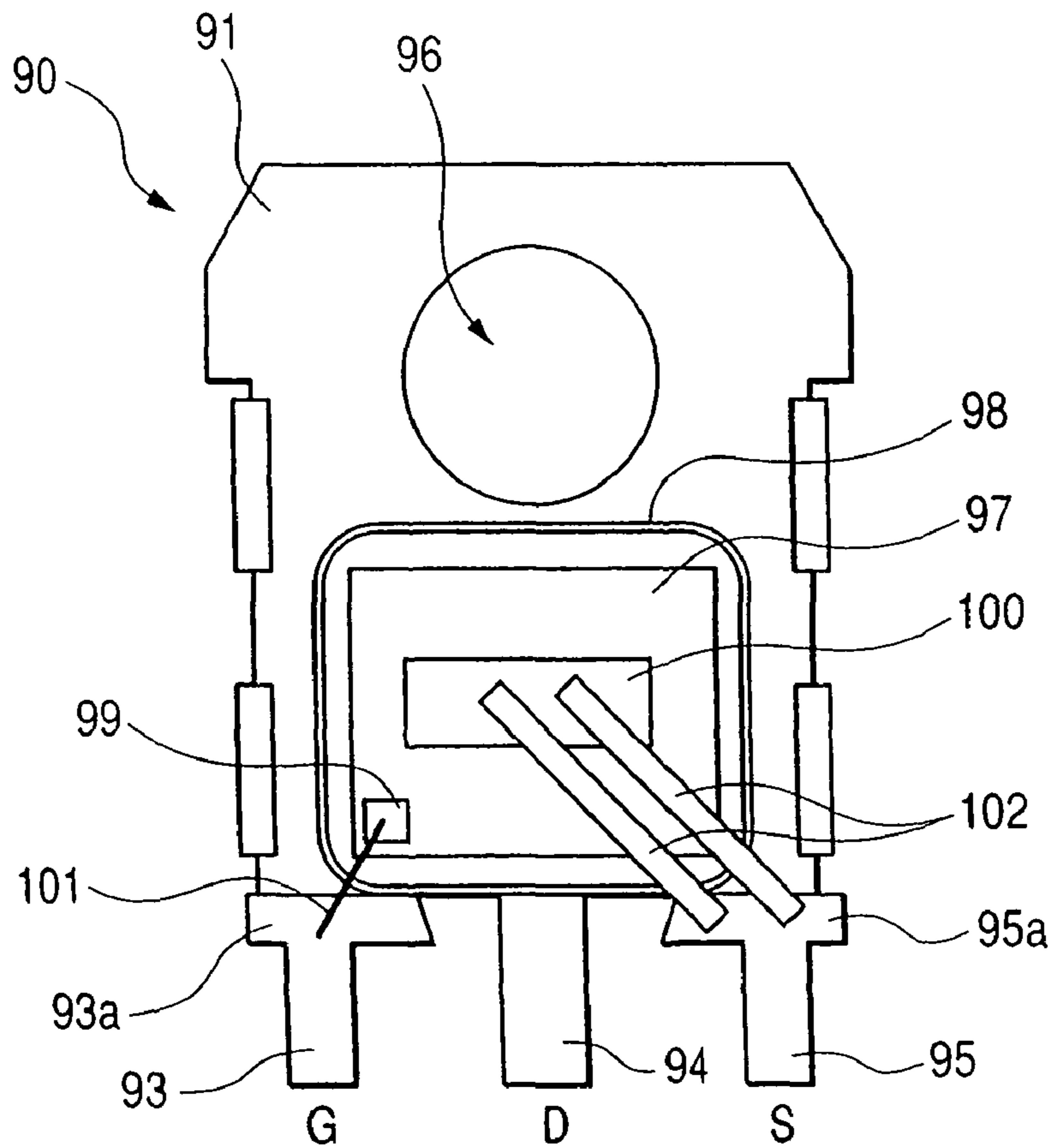
RELATED ART FIG. 25
