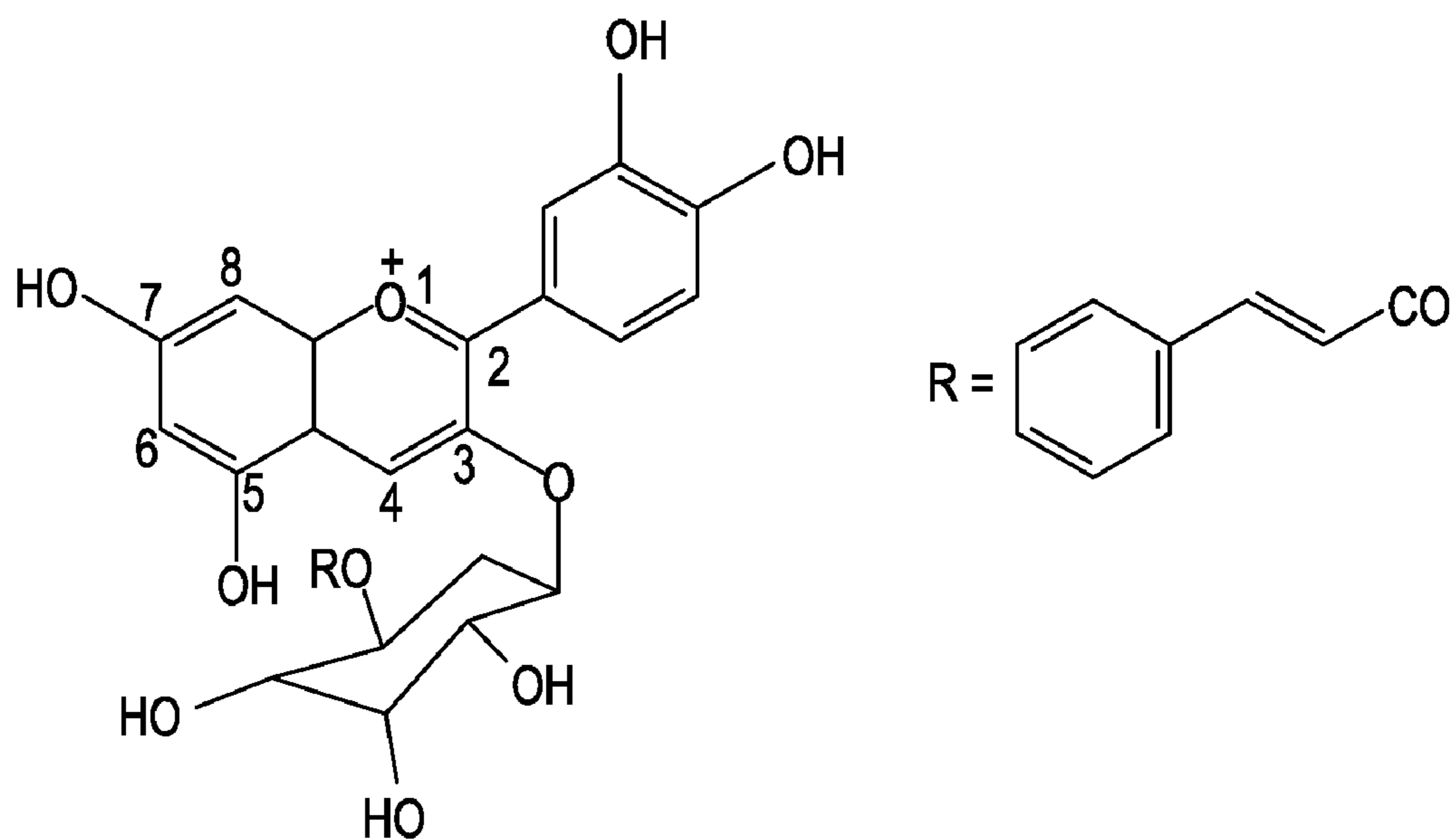
II: CYANIDIN -3- GLUCOSIDE-COUMARATE
