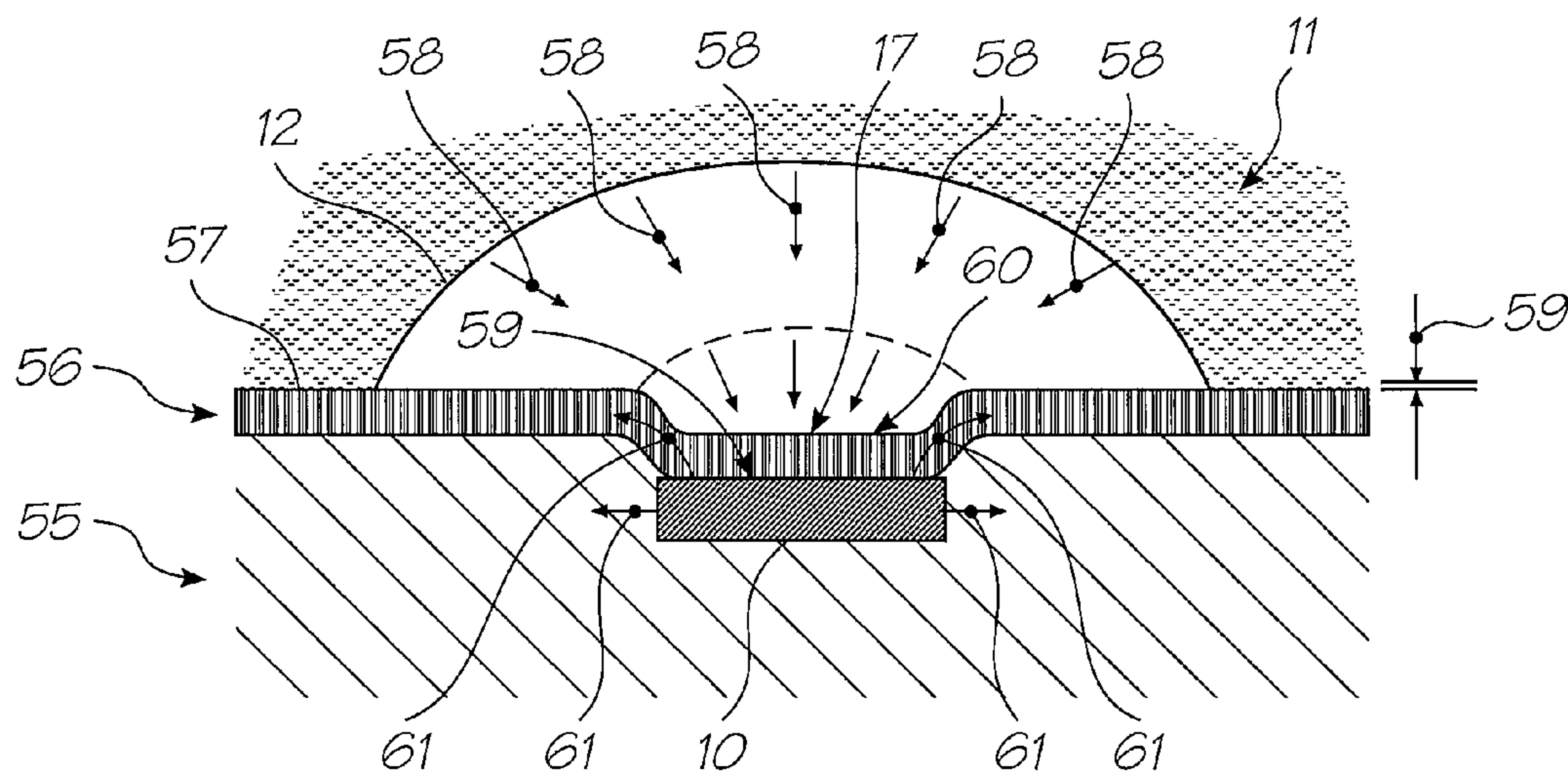
FIG. 57 (PRIOR ART)
