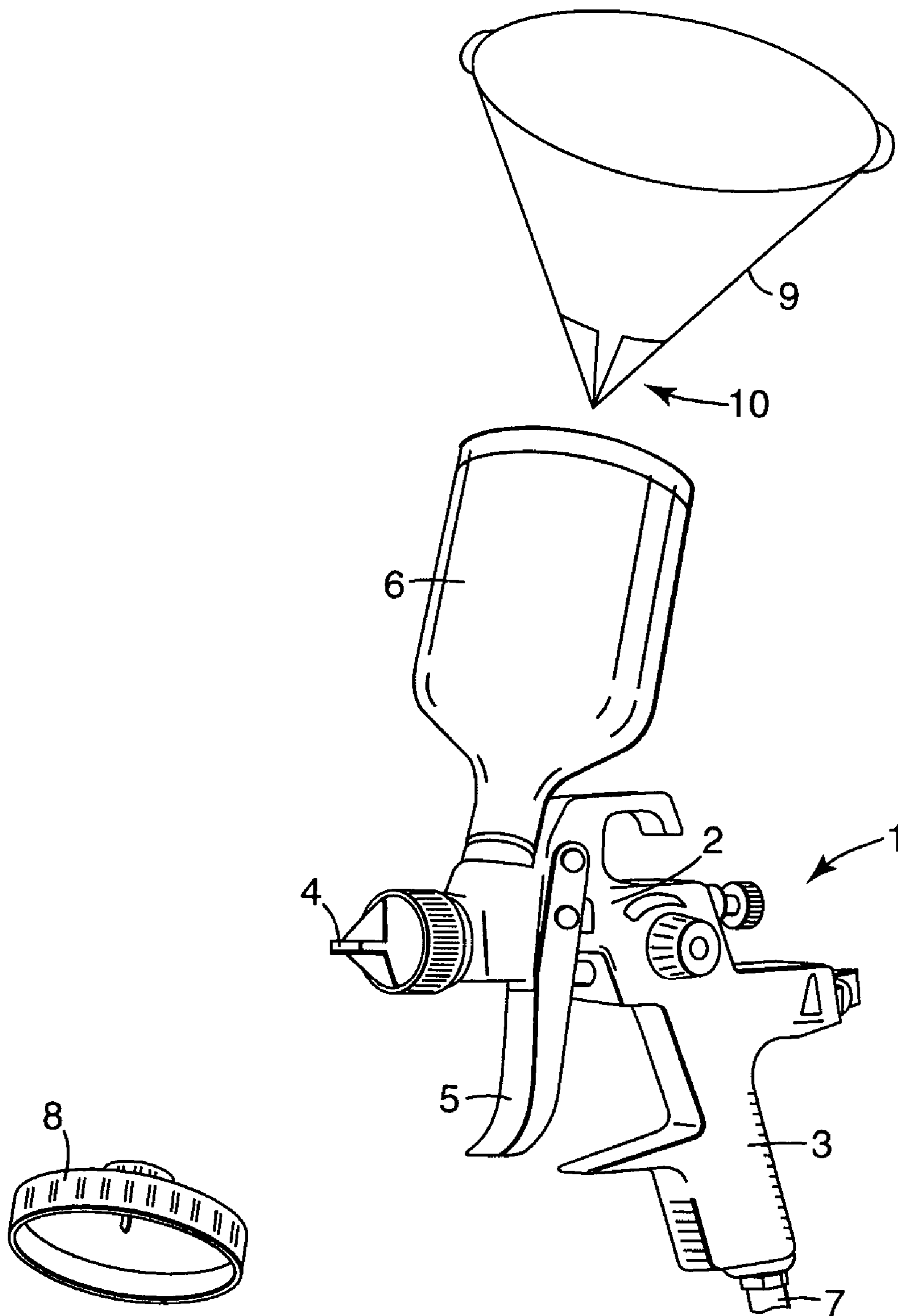
Fig. 1 PRIOR ART
