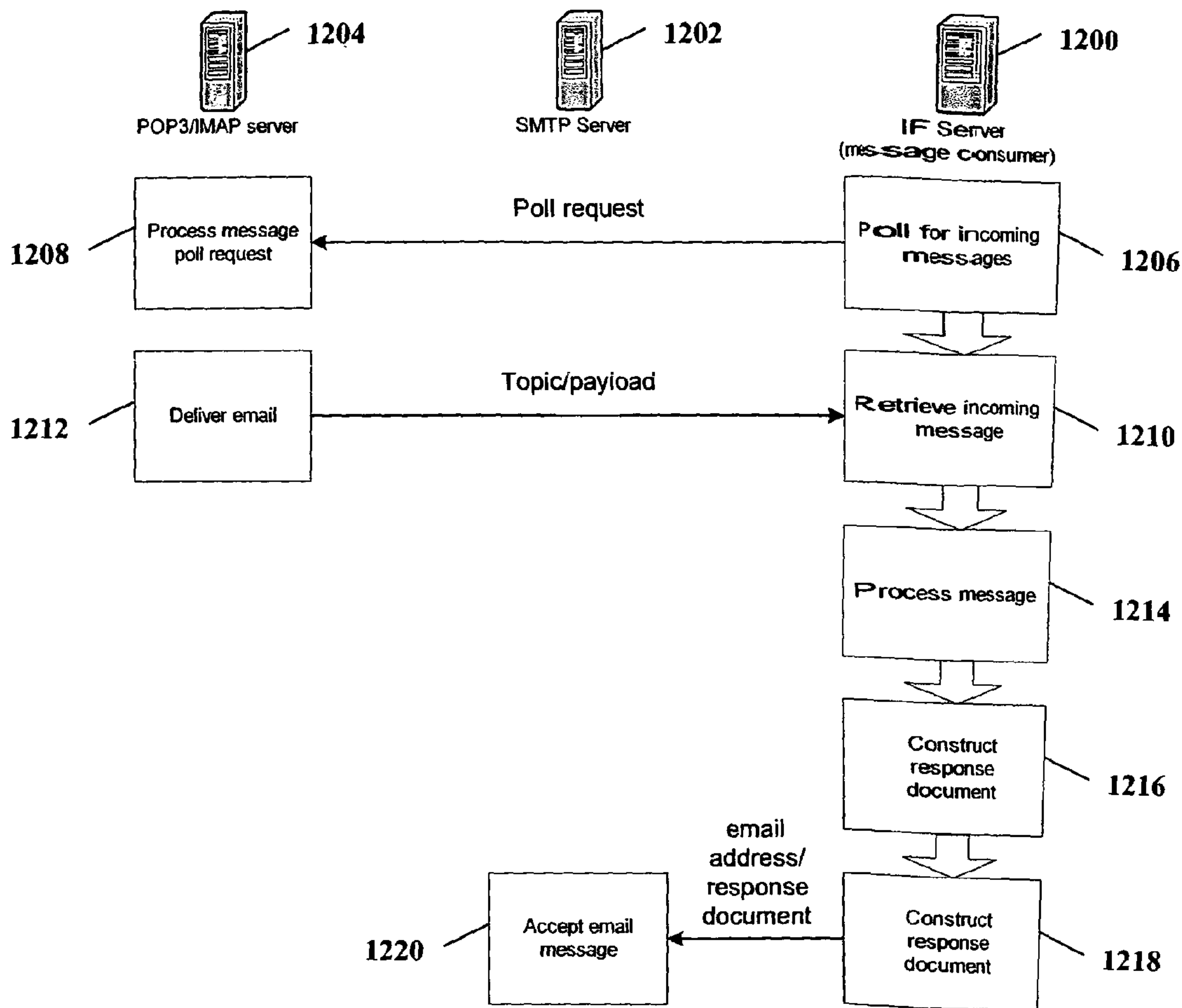
IF Server to SMTP/POP3/ IMAP Server object activation (bi-directional)
