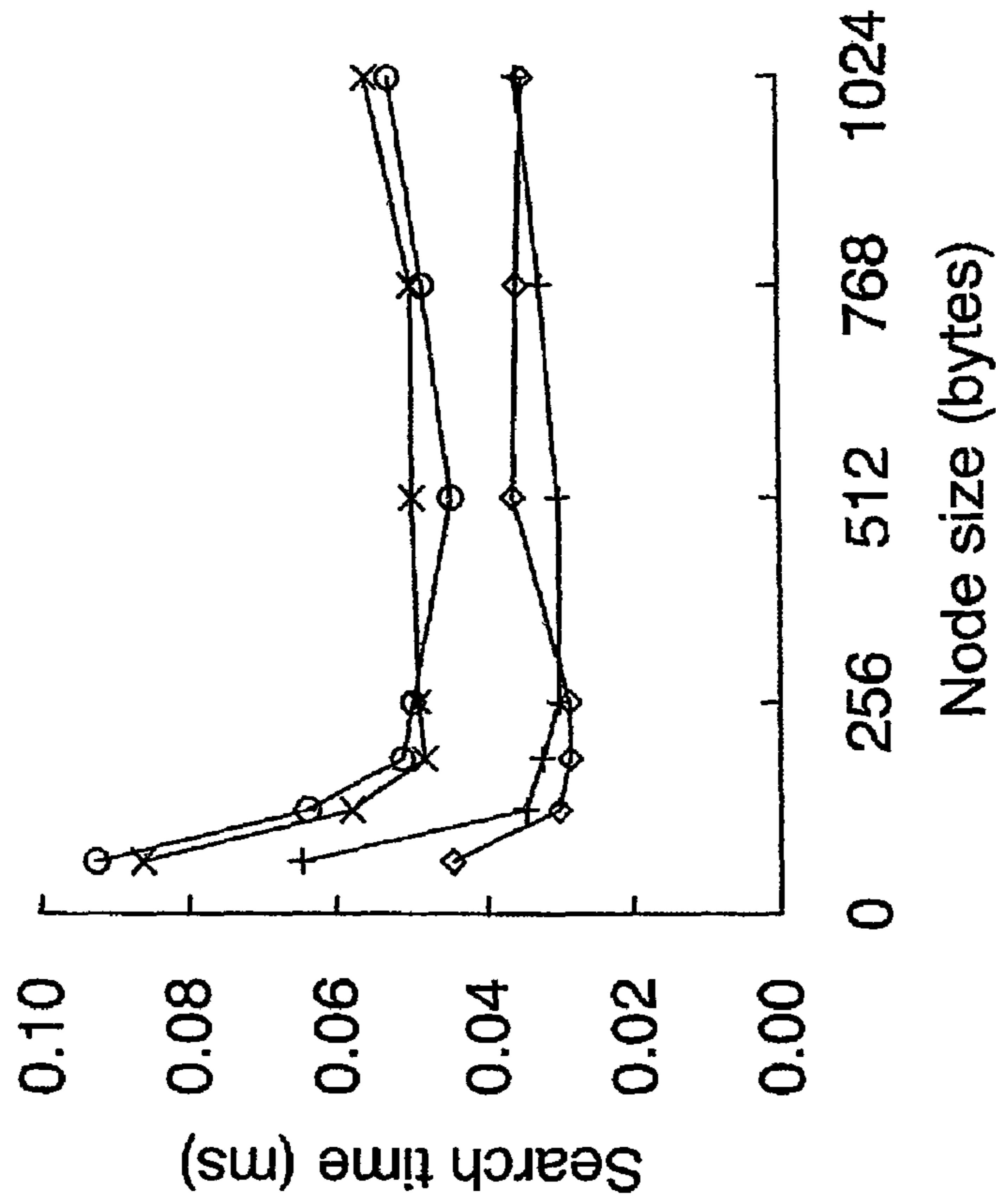
(a) Selectivity = 0.01%
