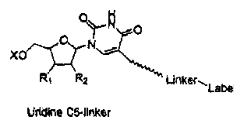
Uridine C5-linker
