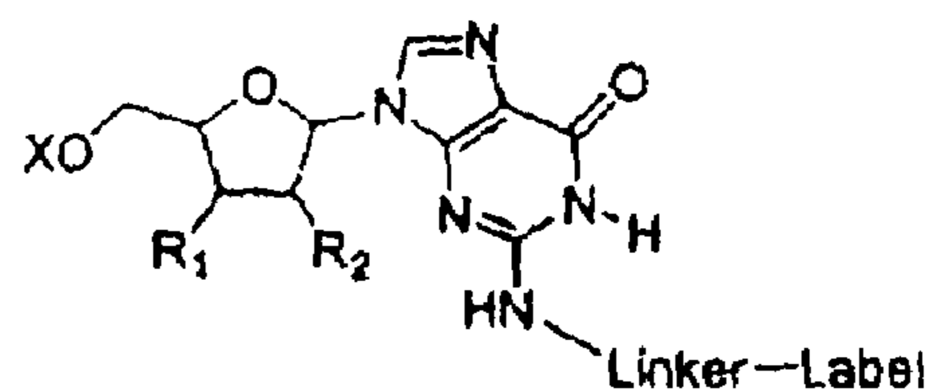
Guanosine N2-linker
