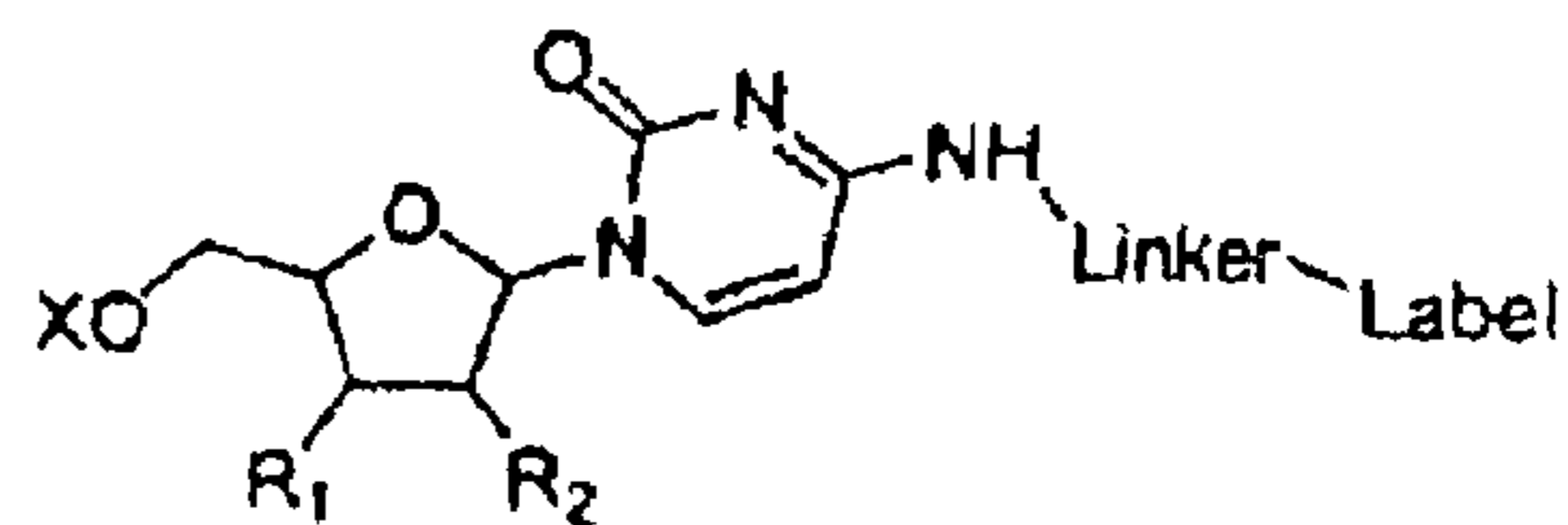
Cytidine N4-linker
