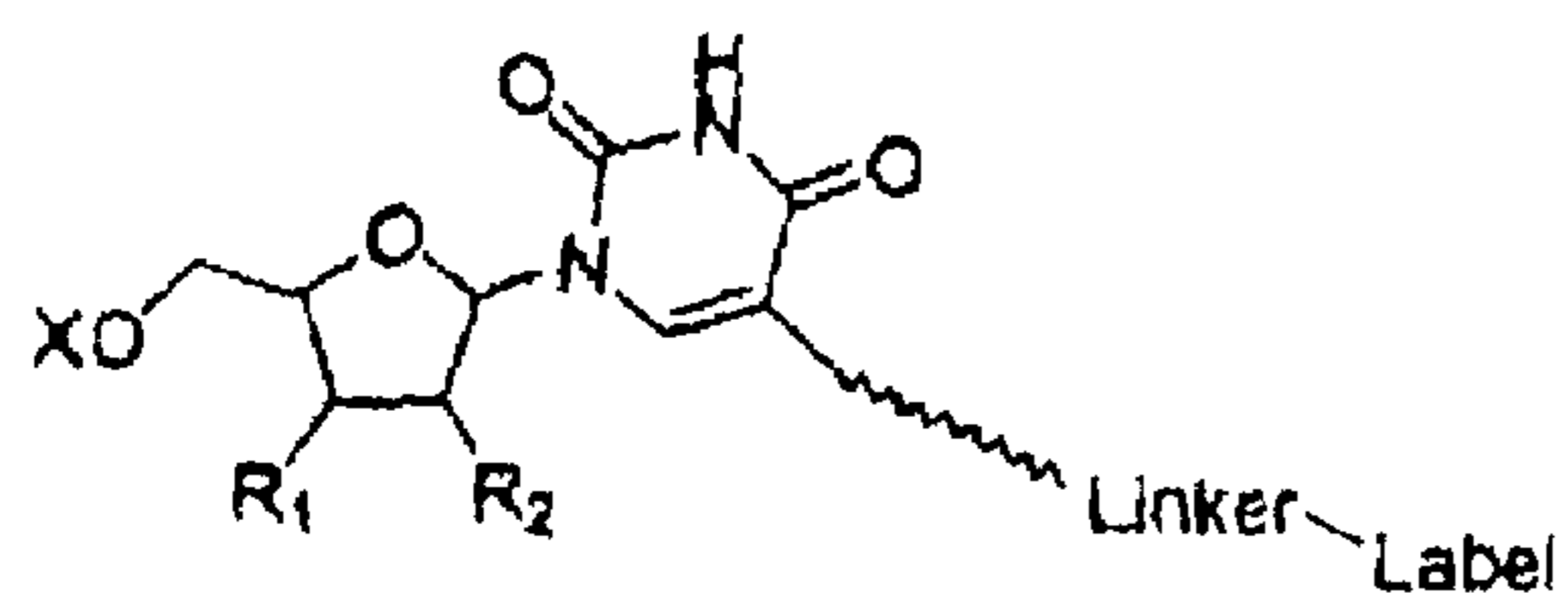
Uridine C5-linker
