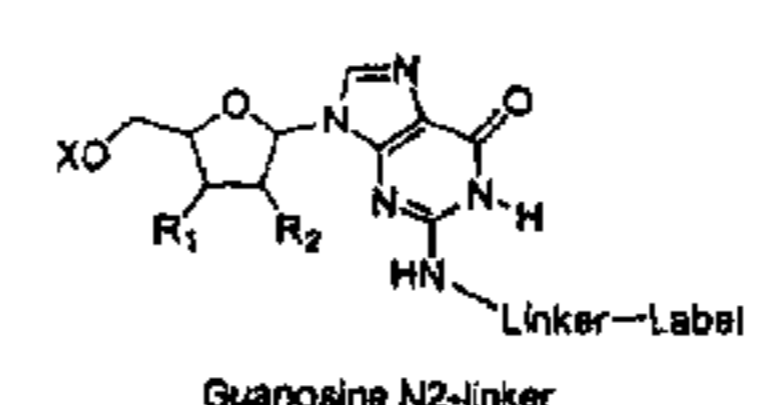
Guanosine N2-linker
