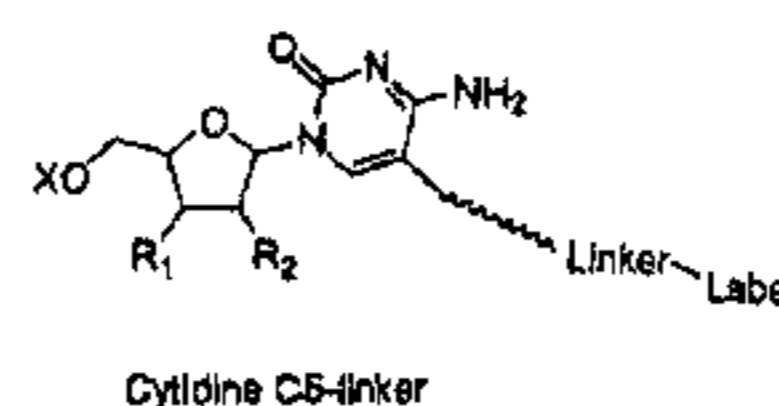
Cytidine C5-linker
