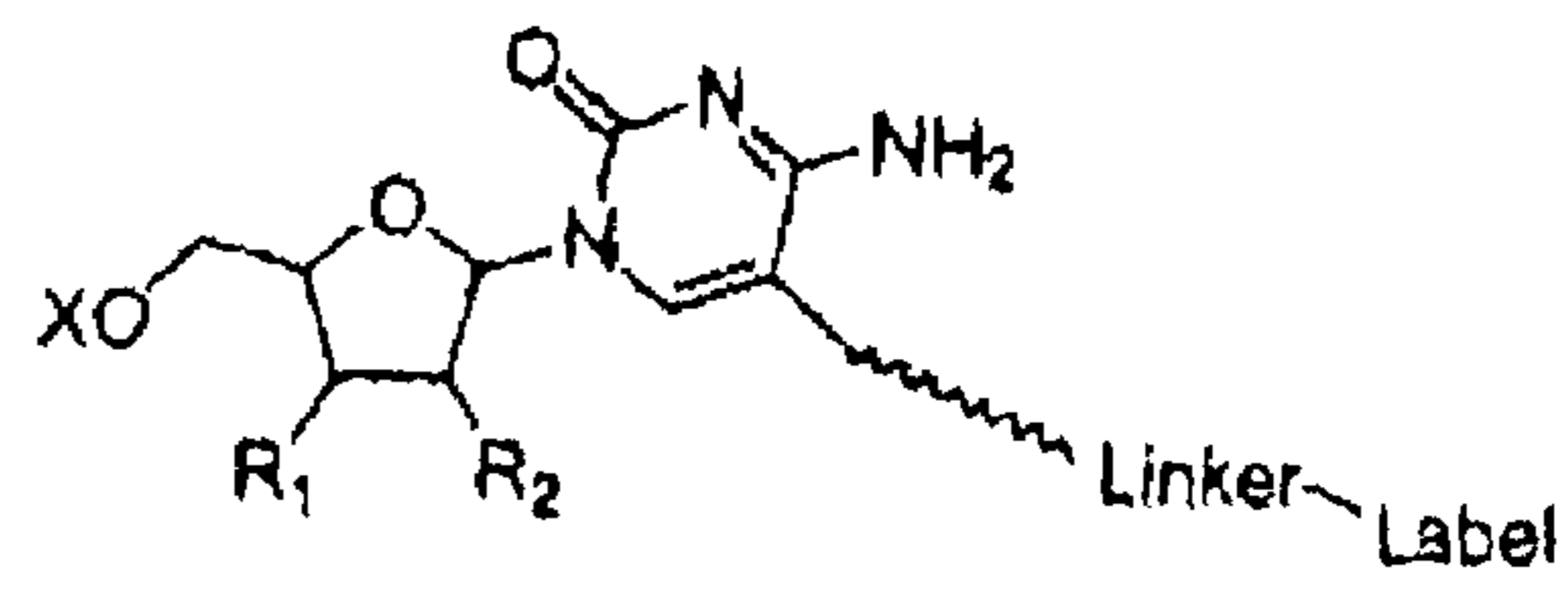
Cytidine C5-linker
