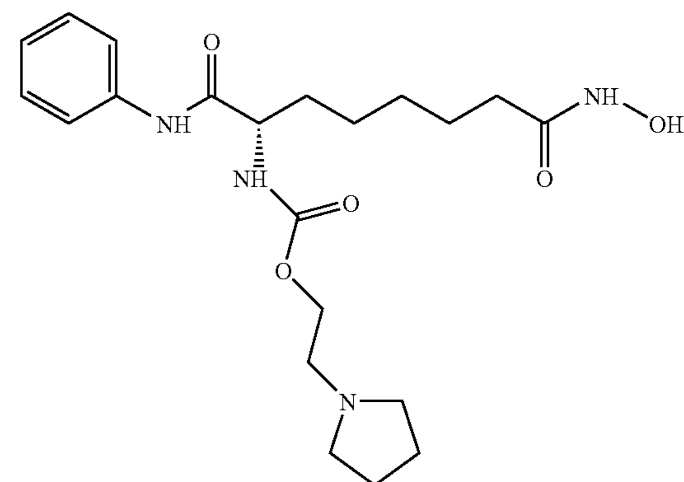
(6-Hydroxycarbamoyl-1-phenylcarbamoyl-hexyl)- carbamic Acid 2-pyrrolidin-1-yl-ethyl Ester
