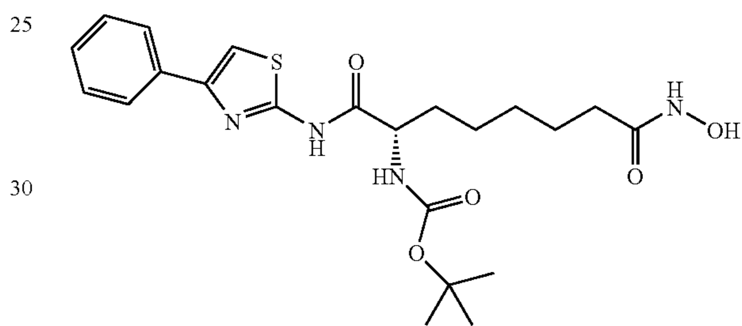
[6-Hydroxycarbamoyl-1-(4-phenyl-thiazol-2-ylcarbamoyl)-hexyl]-carbamic Acid tert-butyl Ester
