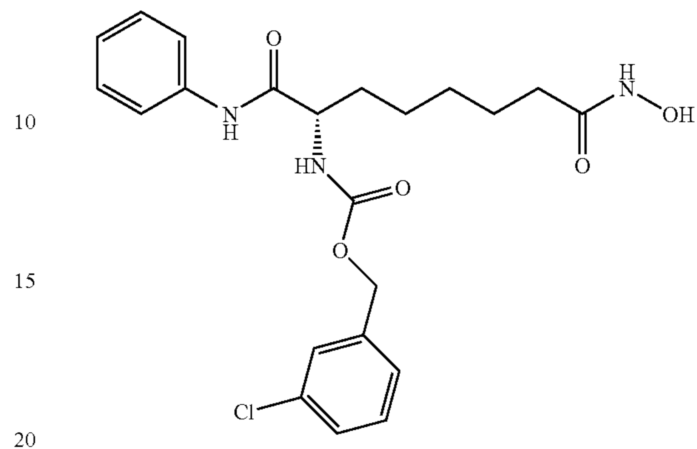
(6-Hydroxycarbamoyl-1-phenylcarbamoyl-hexyl)- carbamic Acid 3-chloro-benzyl Ester
