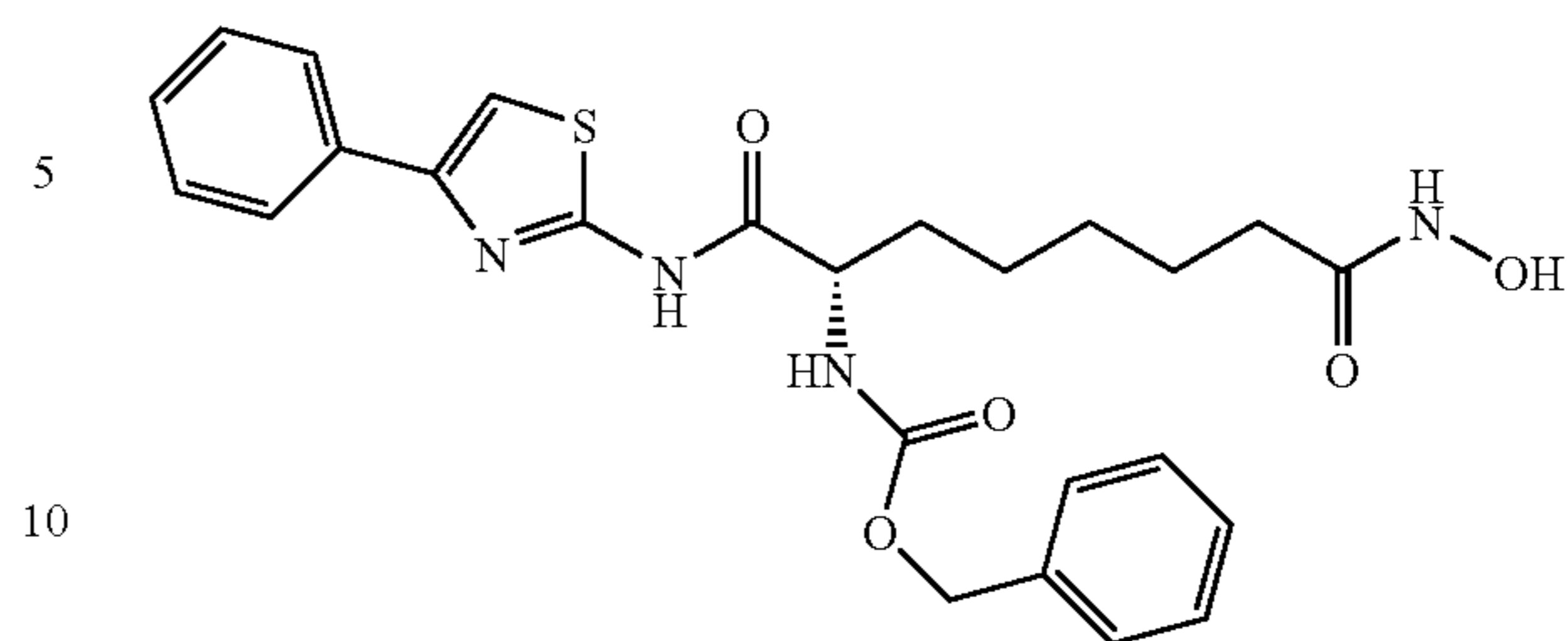
[6-Hydroxycarbamoyl-1-(4-phenyl-thiazol-2-ylcarbamoyl)-hexyl]-carbamic Acid Benzyl Ester
