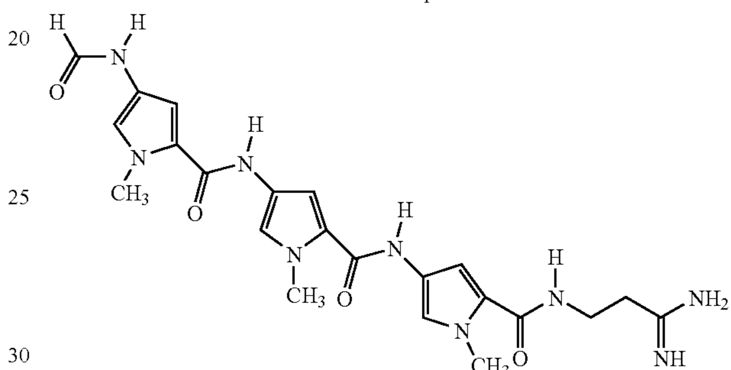
Lexitropsin
