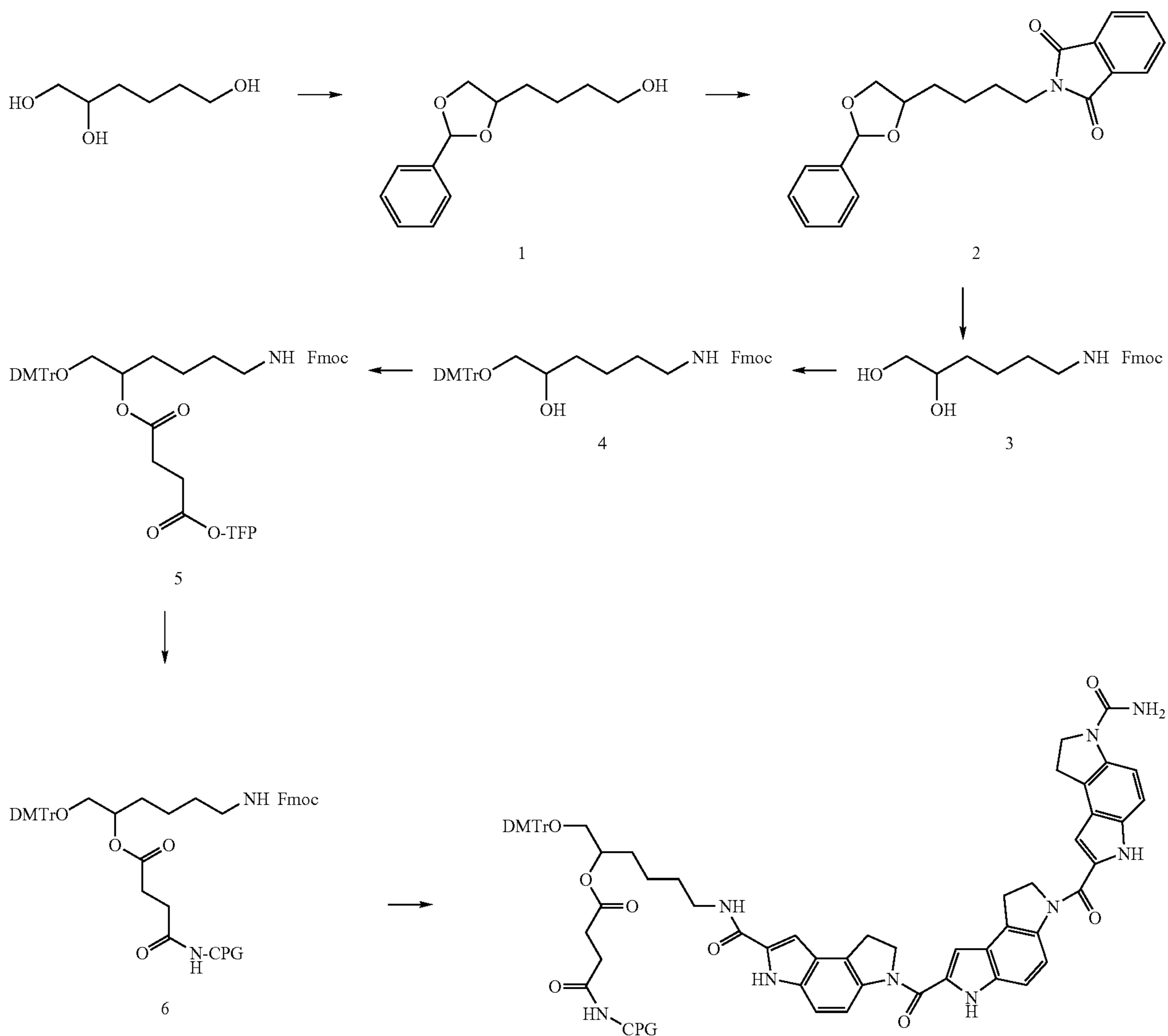
Scheme 6: Preparation of \text{CDPI}_3 -CPG support (below)
