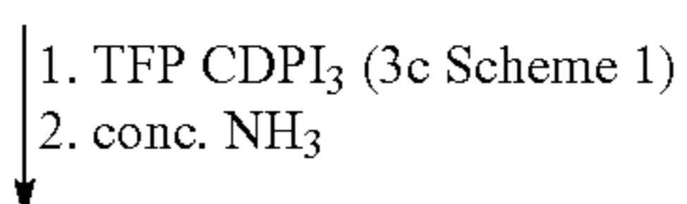
Reaction Scheme 4
