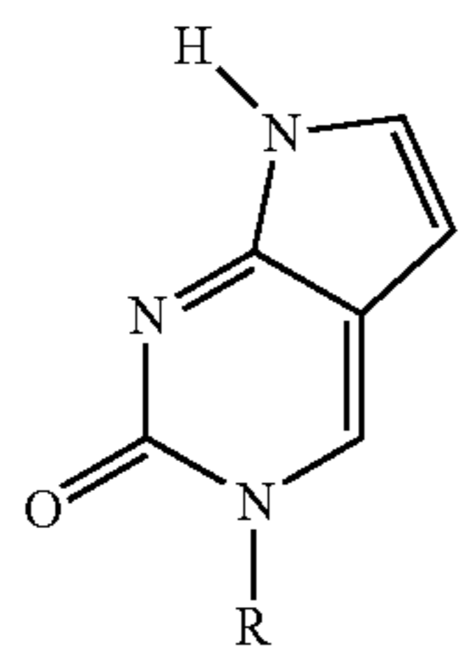
5-N 4 ethencytosine 2-deoxyribosides
