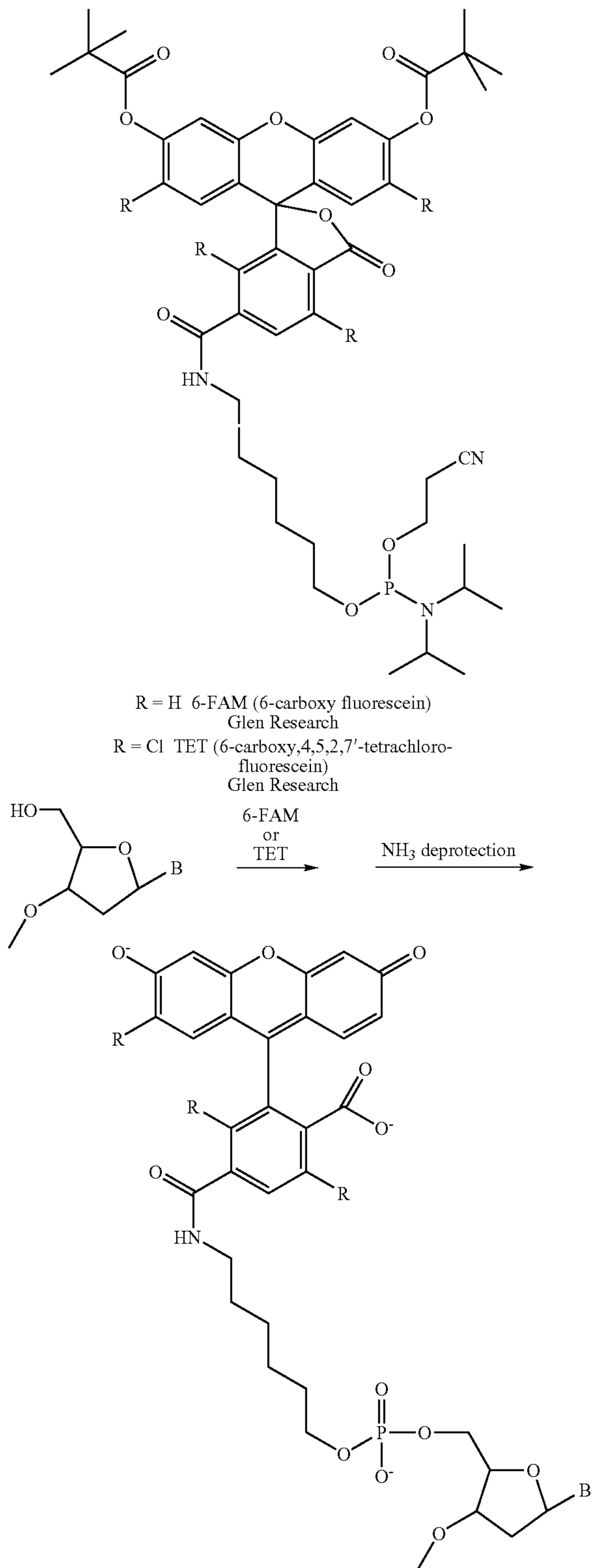
Scheme 8: Introduction of fluorophores at the 5'-end using 6-FAM and TET phosphoramidates (below)
