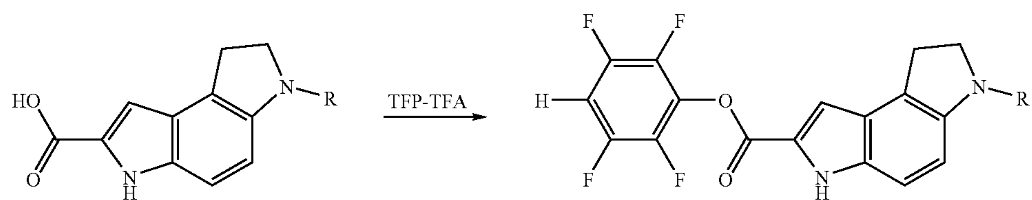
Reaction Scheme 1
