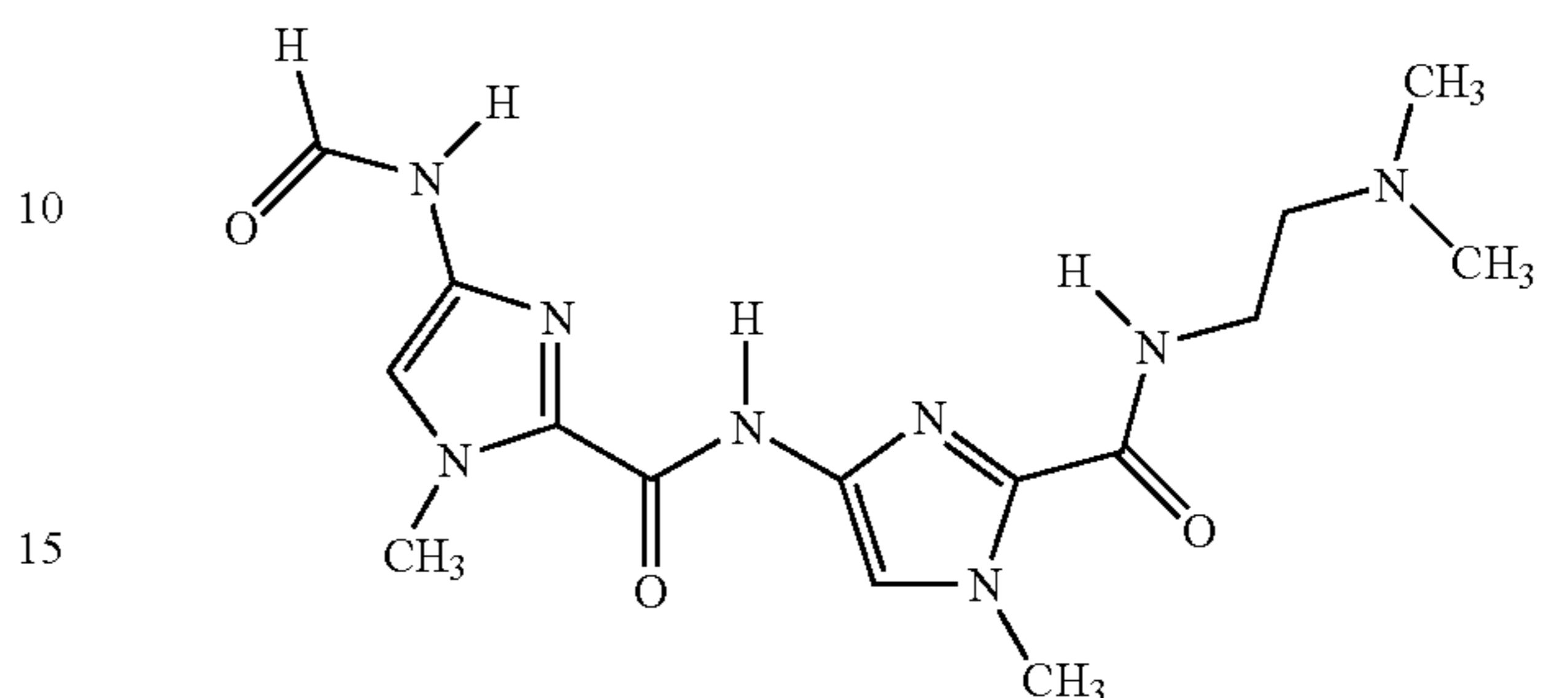
Lexitropsin
