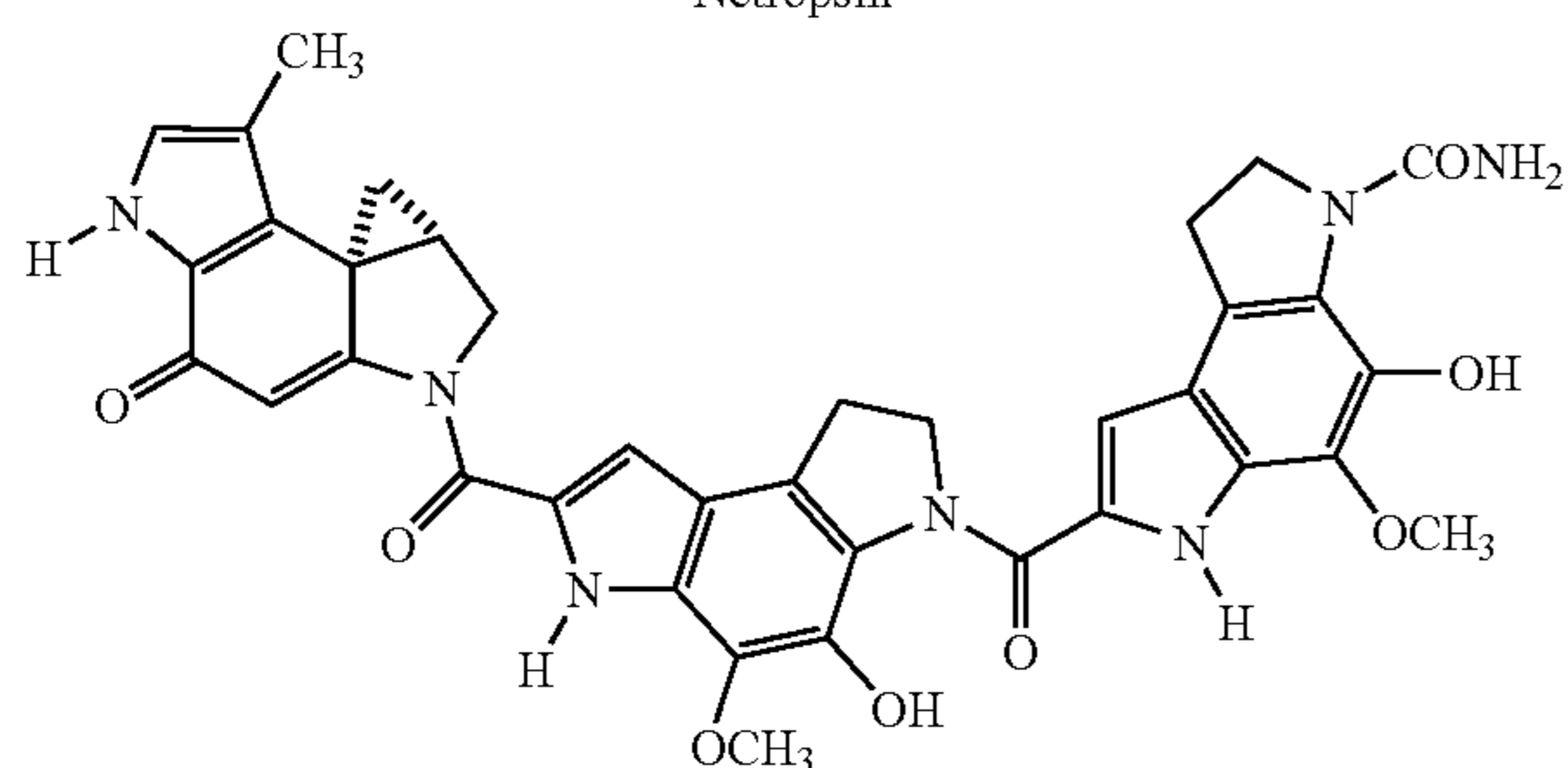
CC-1065
