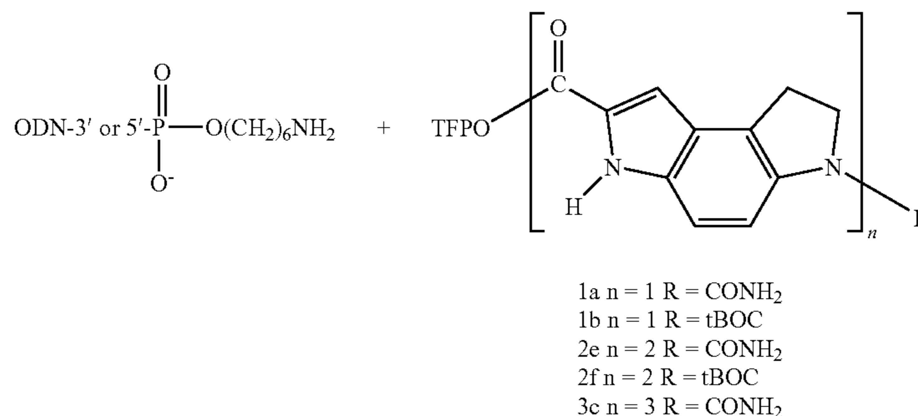
Reaction Scheme 3
