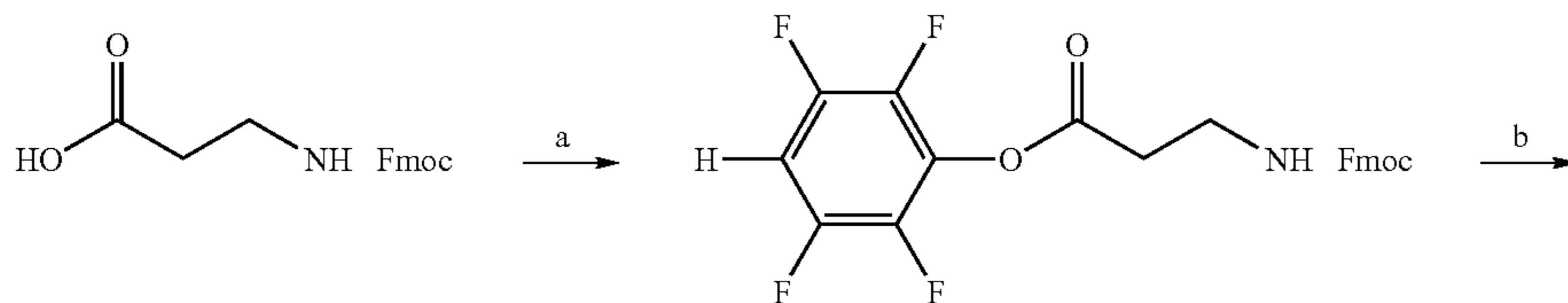
Reaction Scheme 5
