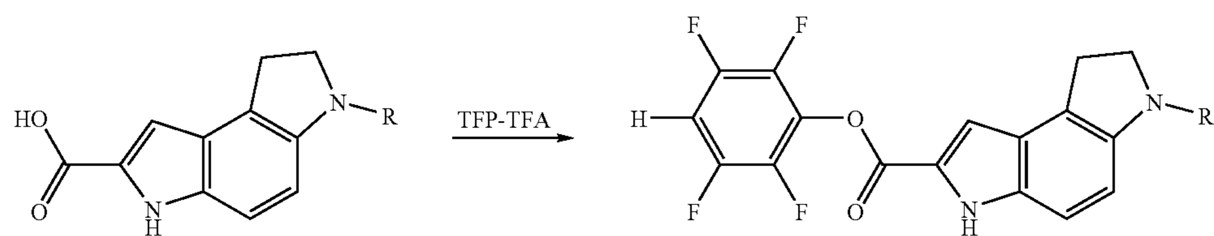
Reaction Scheme 1
