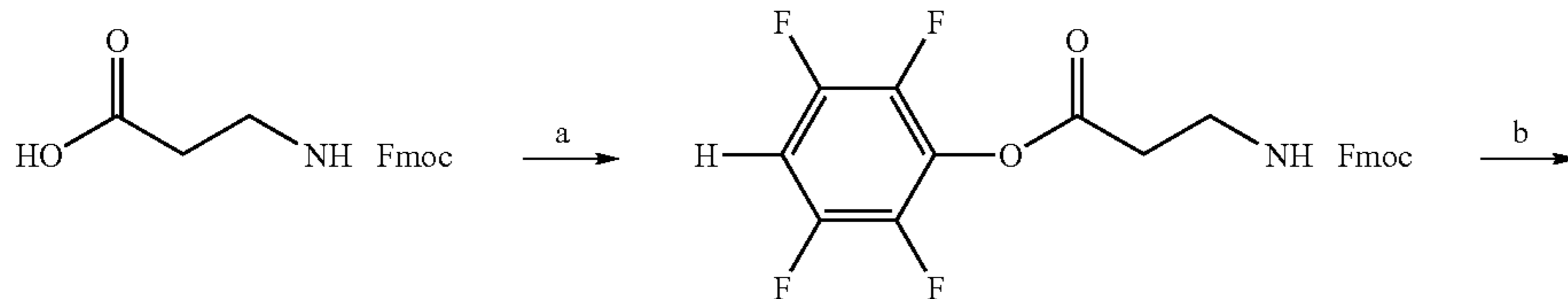
Reaction Scheme 5
