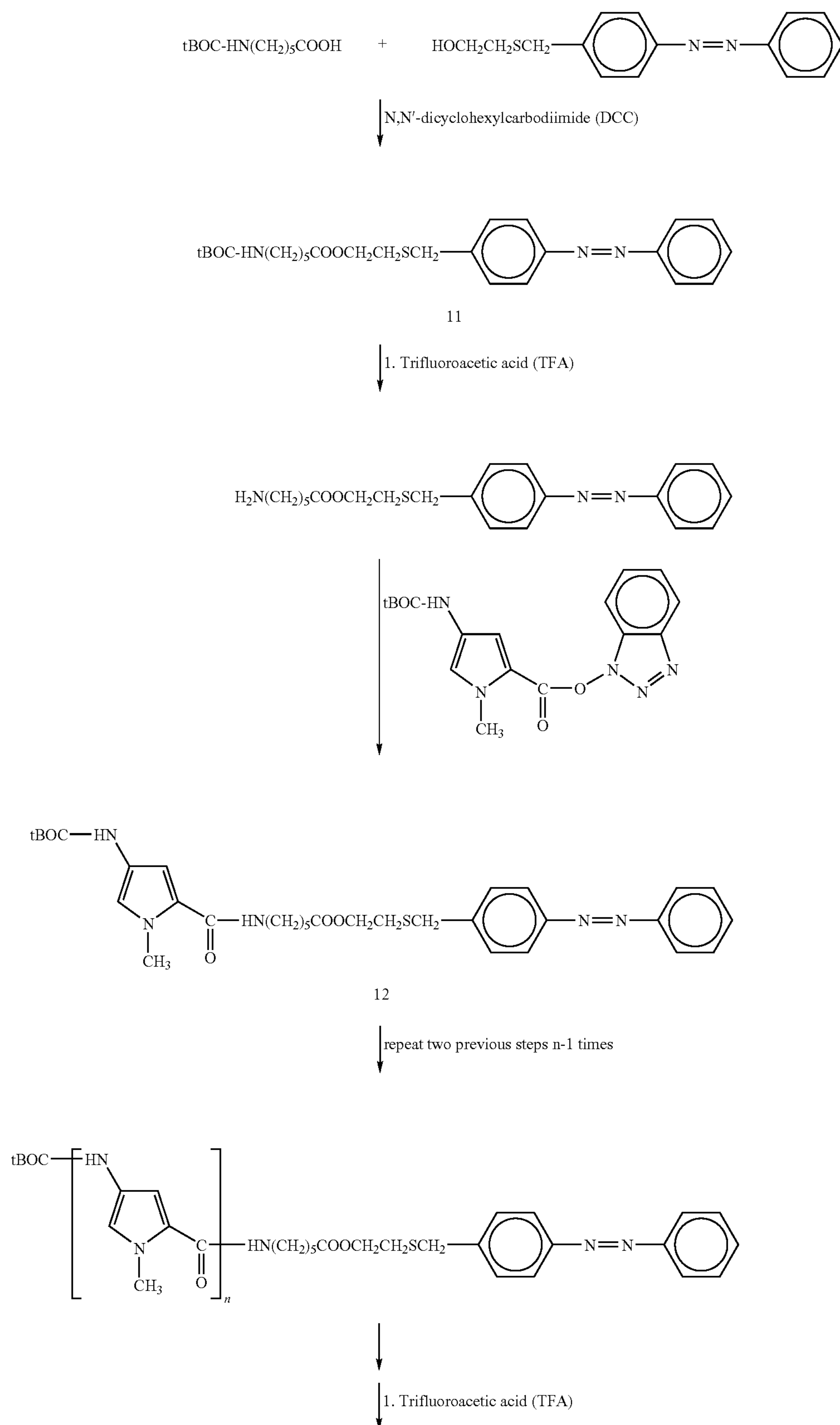
Reaction Scheme 2
