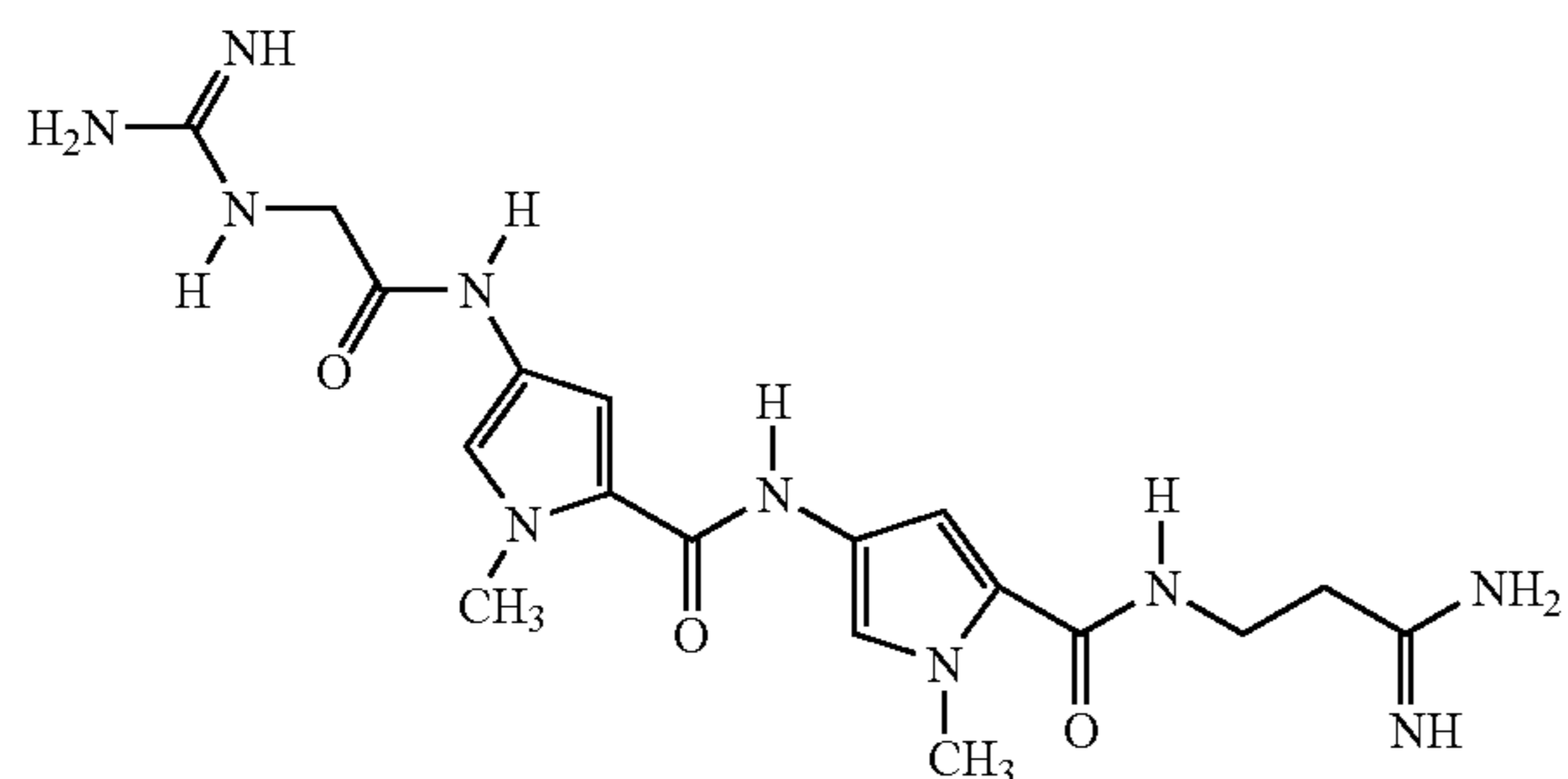
Netropsin
