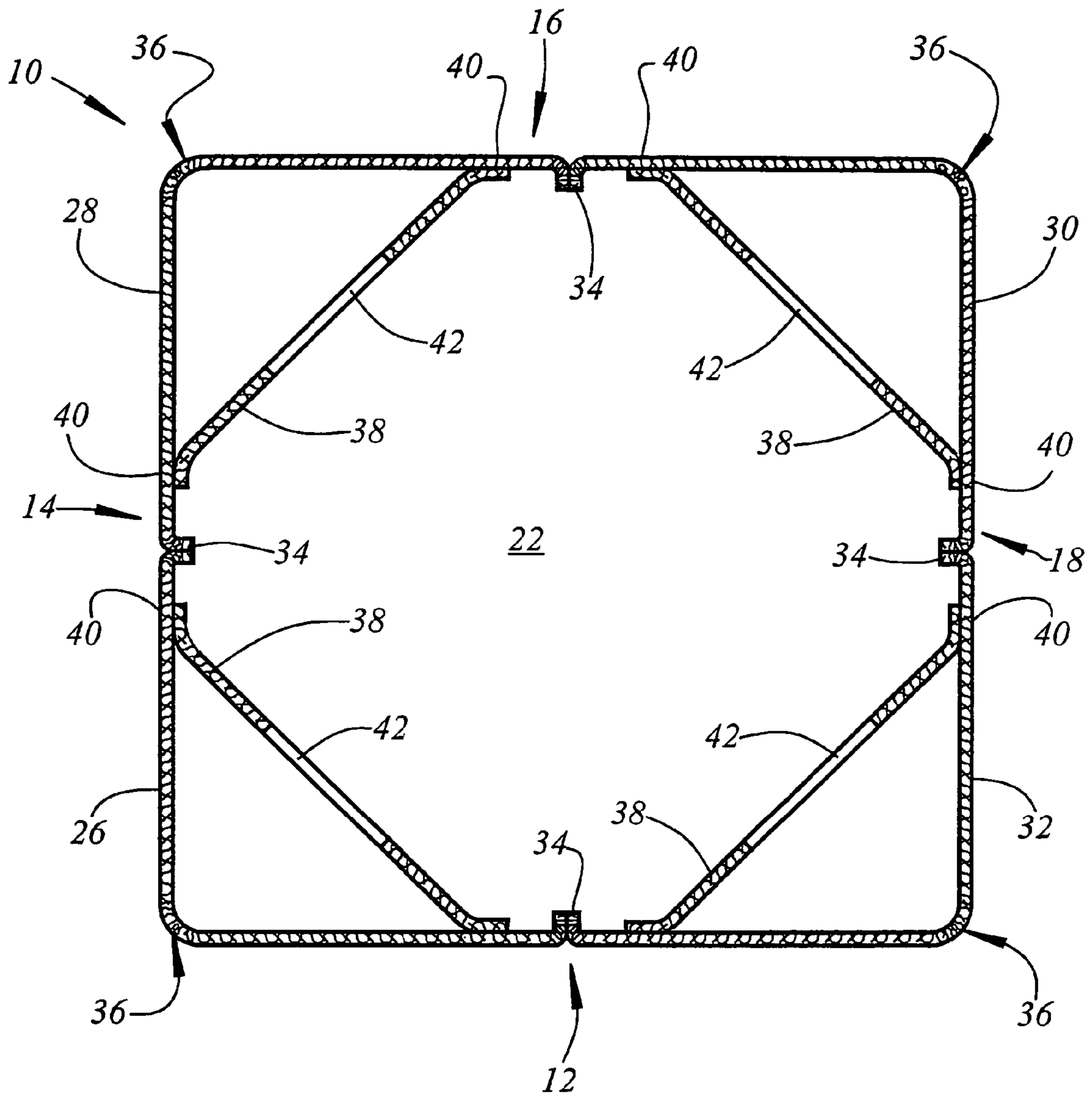
Fig. 2 Prior Art
