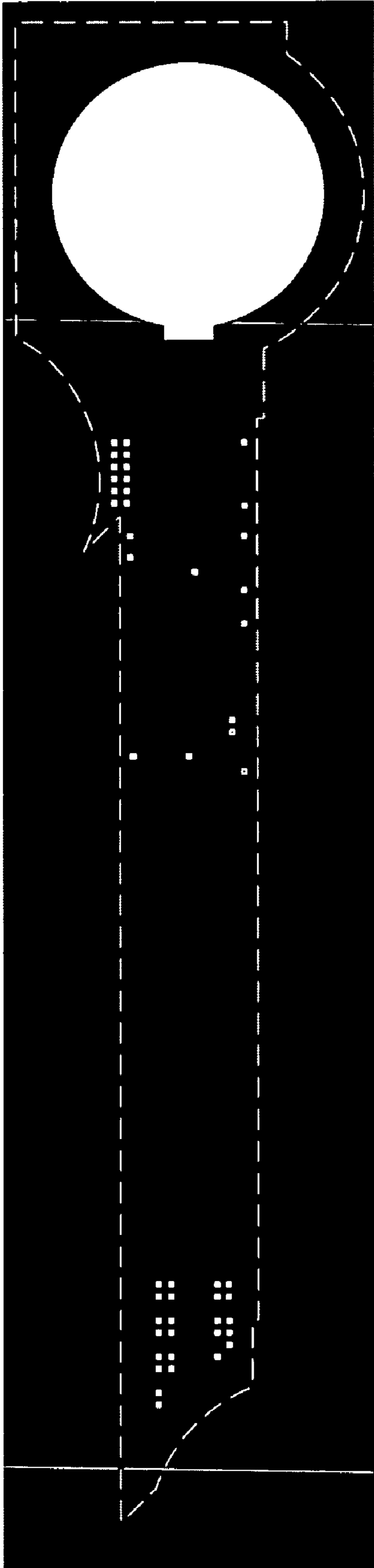
Via 1 mask
