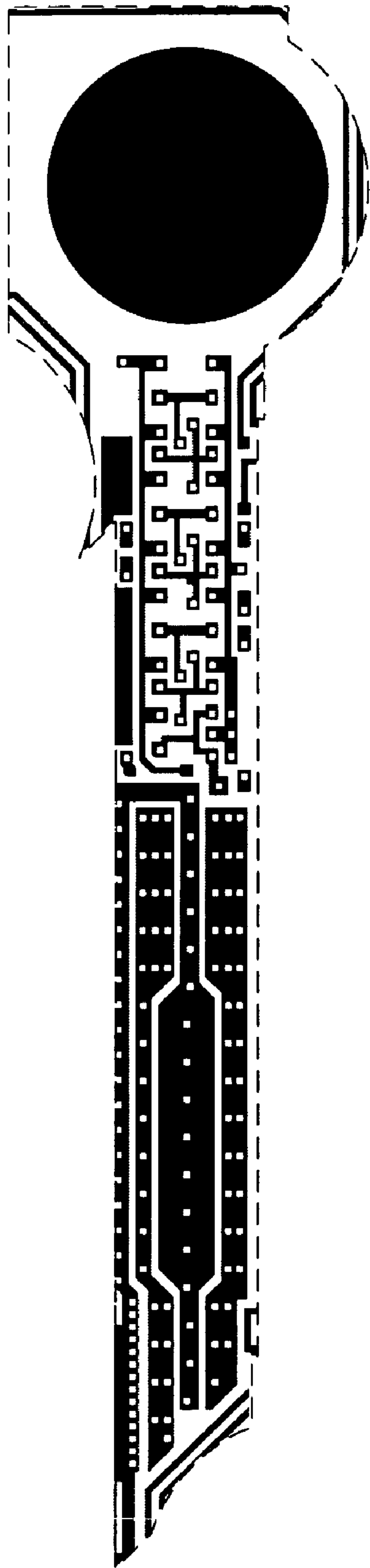
Metal 1 mask
