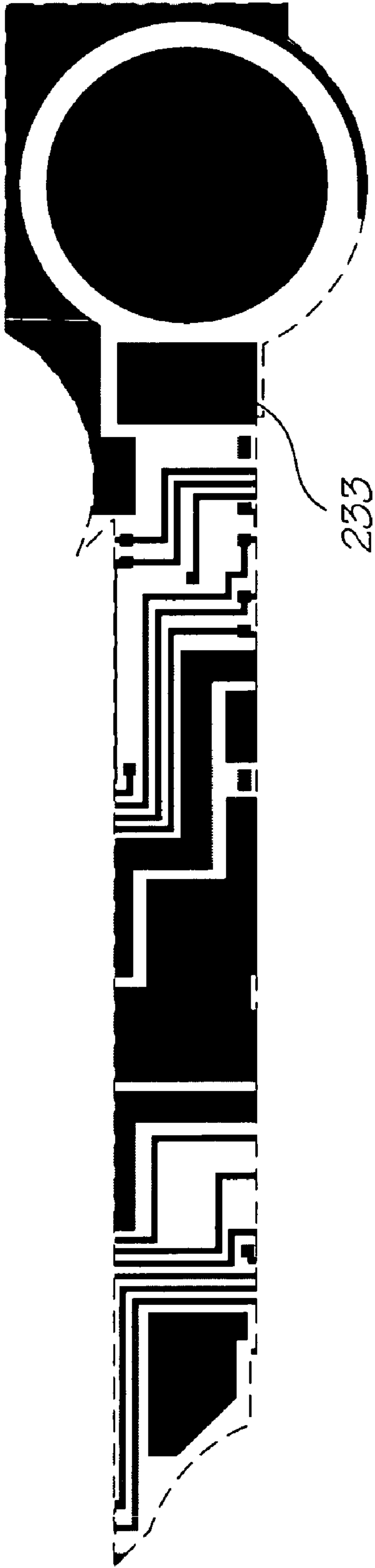
Metal 2 mask
