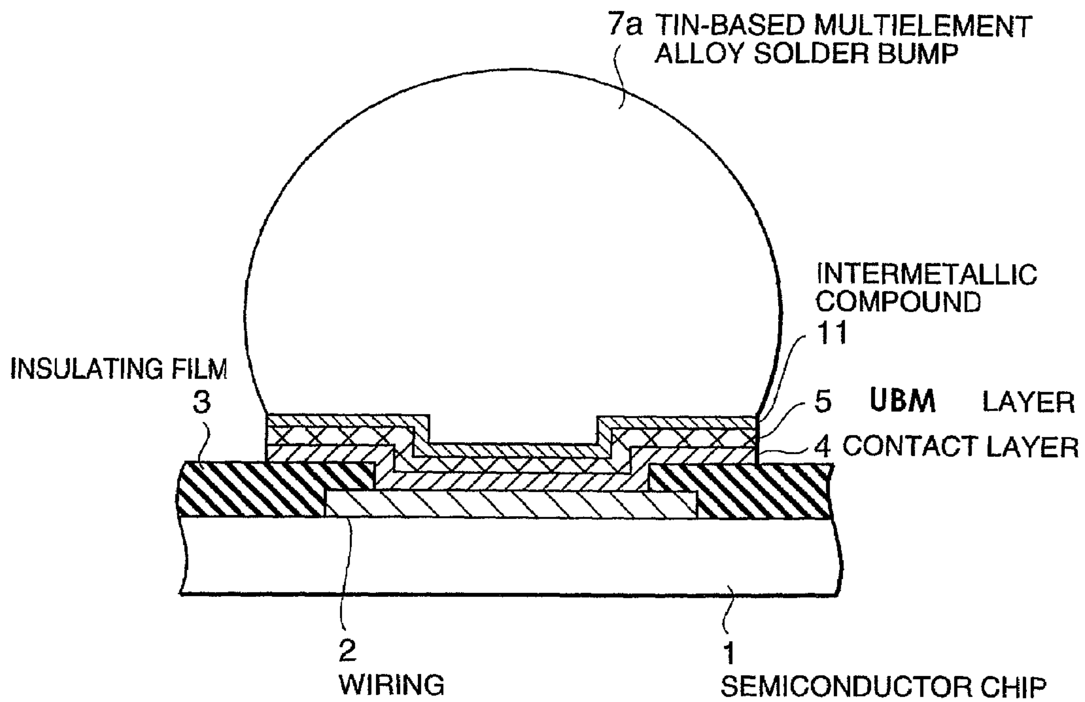
FIG.5 PRIOR ART
