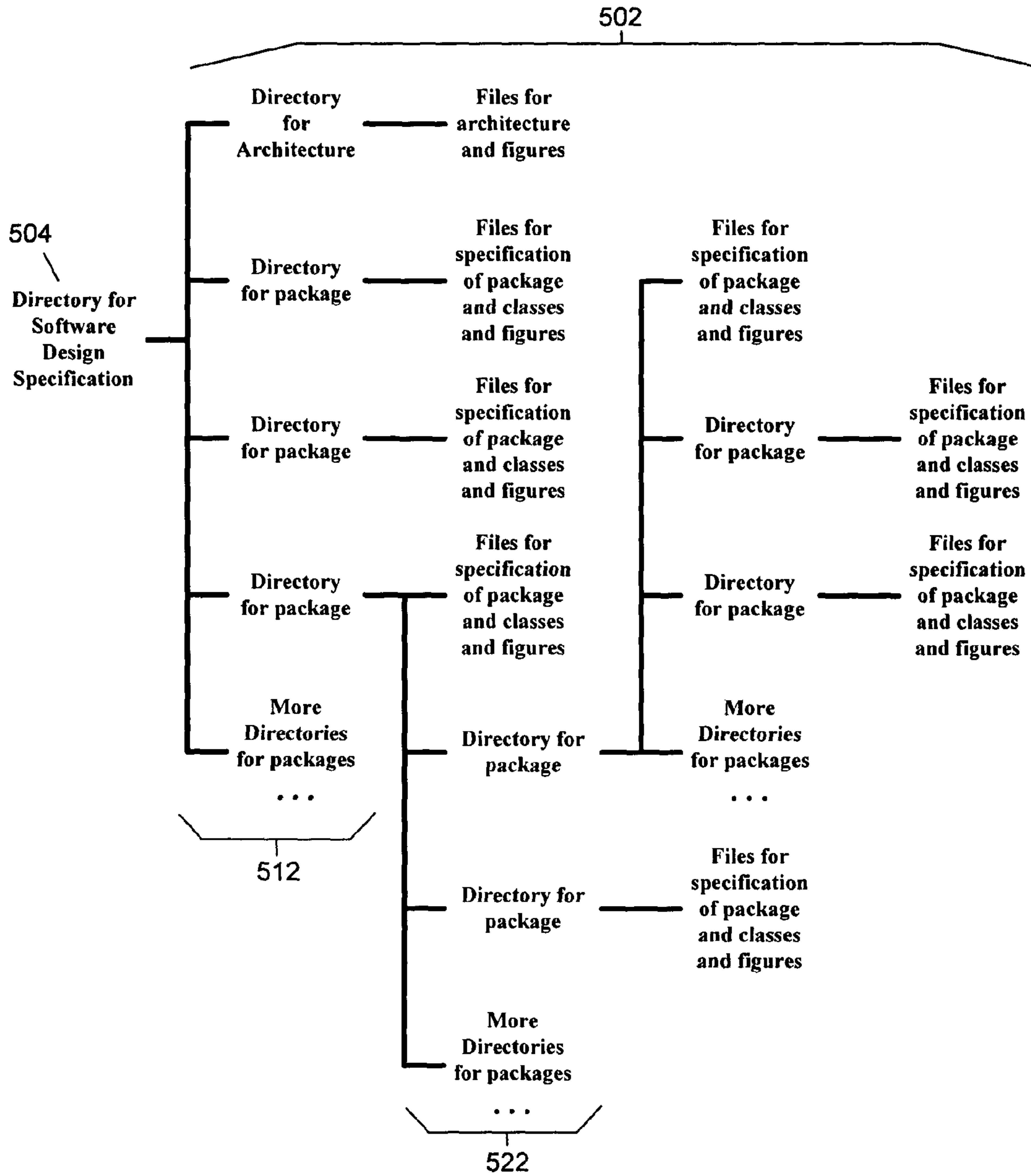
Organization of Software Design Specification Directory
