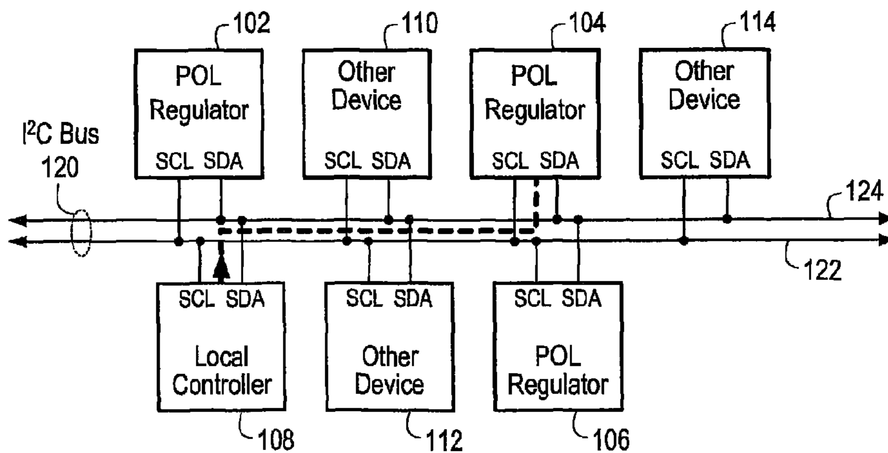
FIG. 3 (Prior Art)
