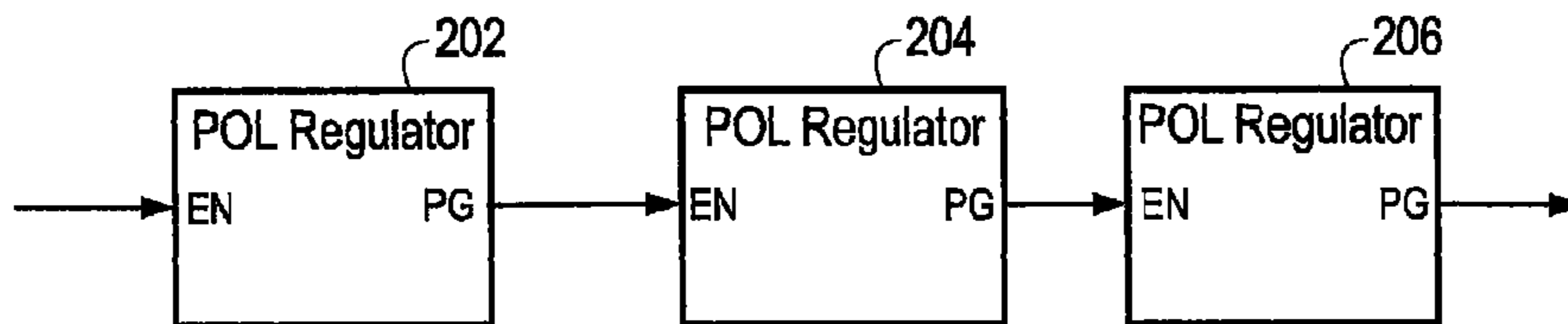
FIG. 5 (Prior Art)
