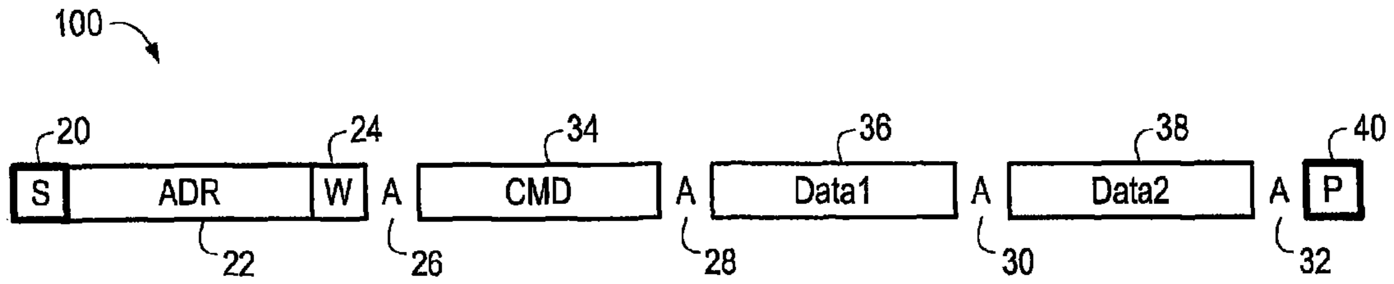
FIG. 1 (Prior Art)
