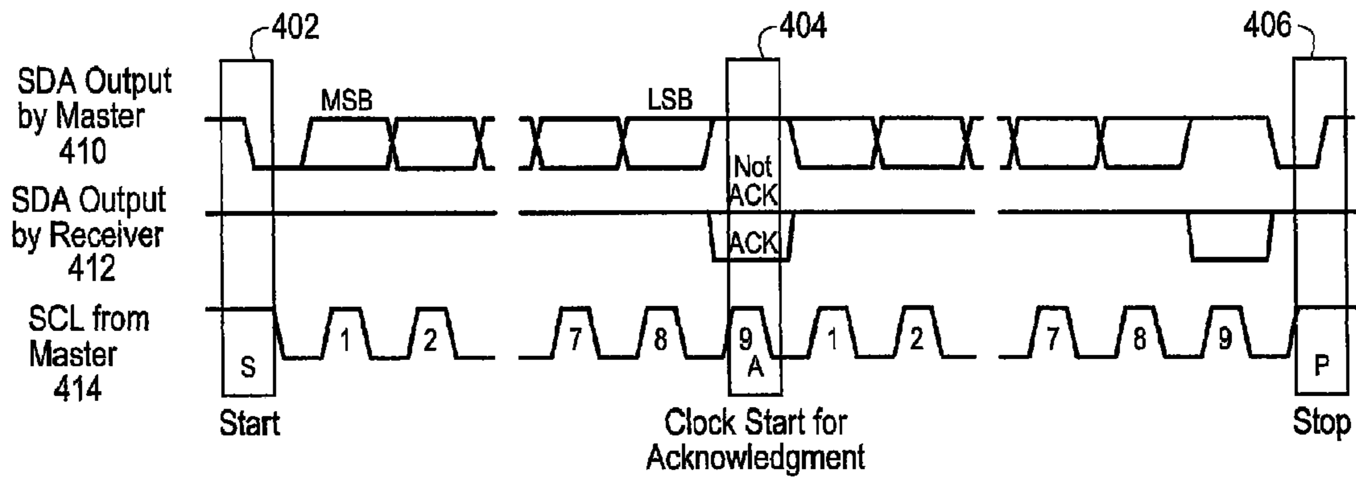
FIG. 4 (Prior Art)
