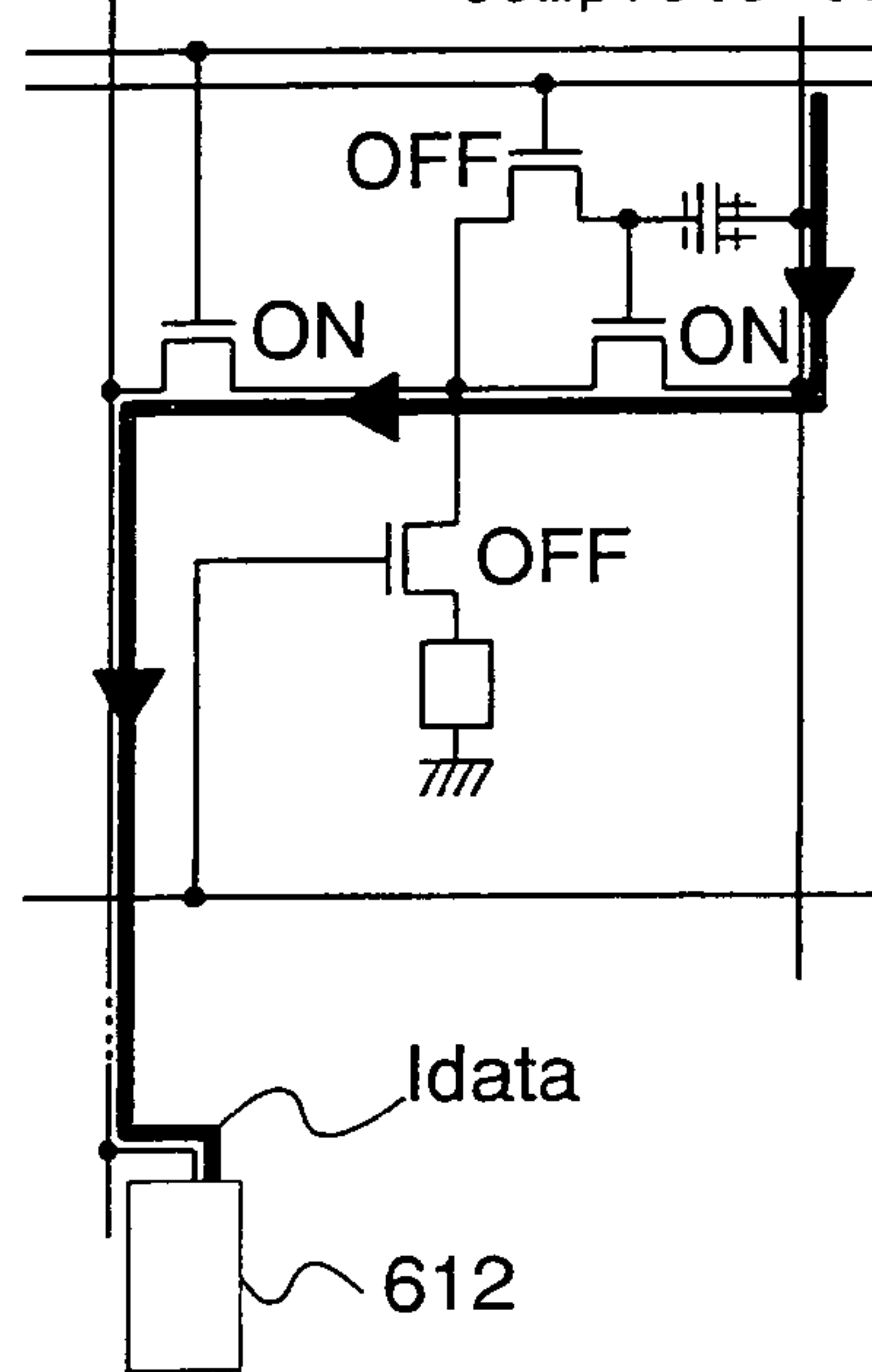
Fig. 17B signal input complete time
