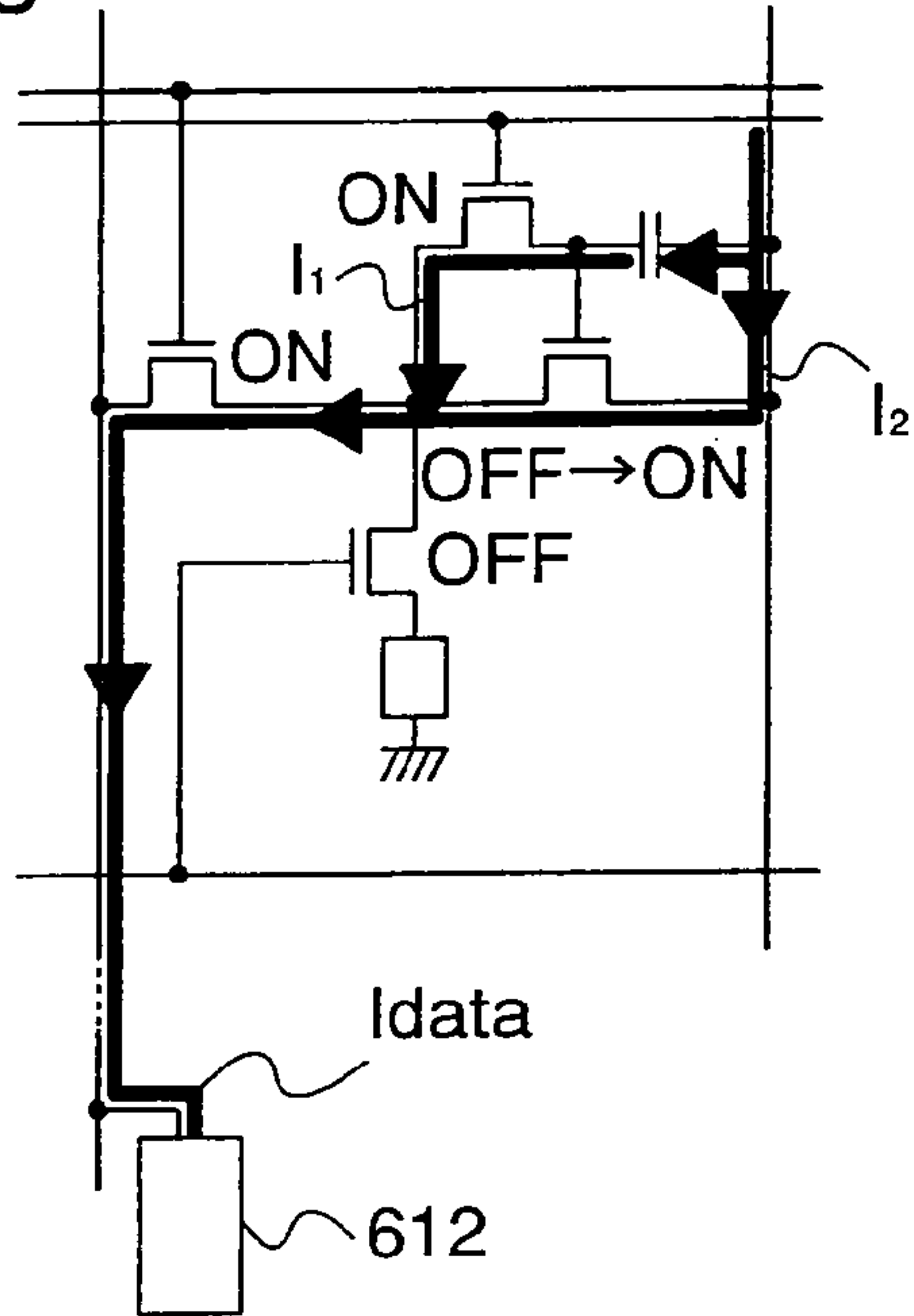
Fig. 17A signal input time
