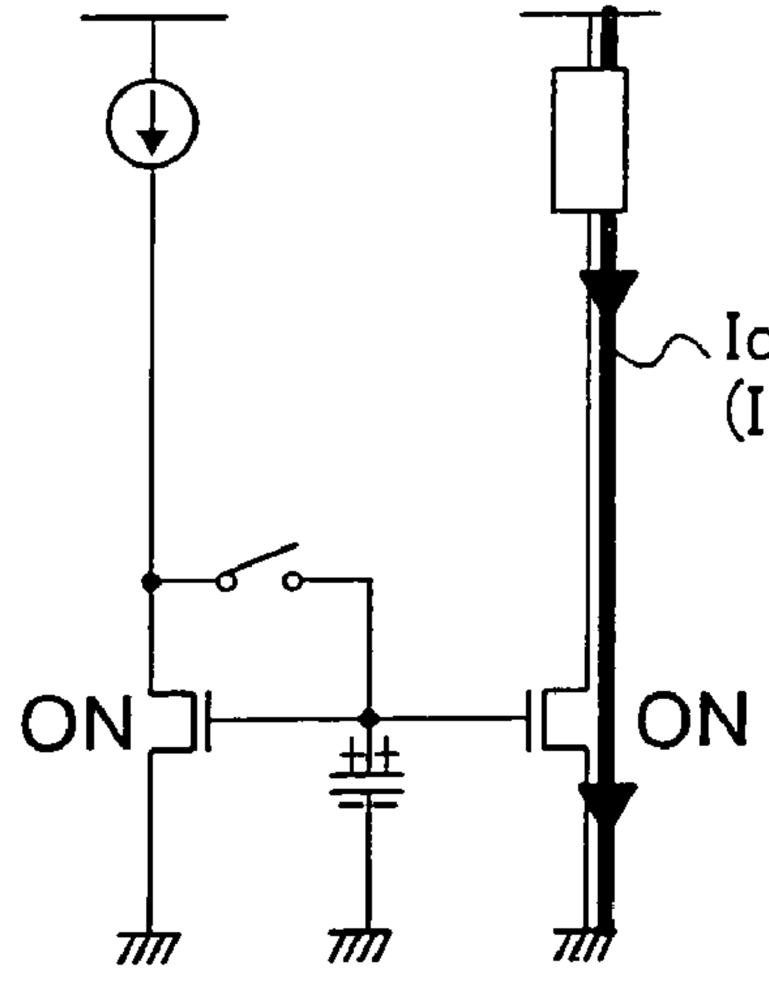
Fig. 20C signal input time to pixel
