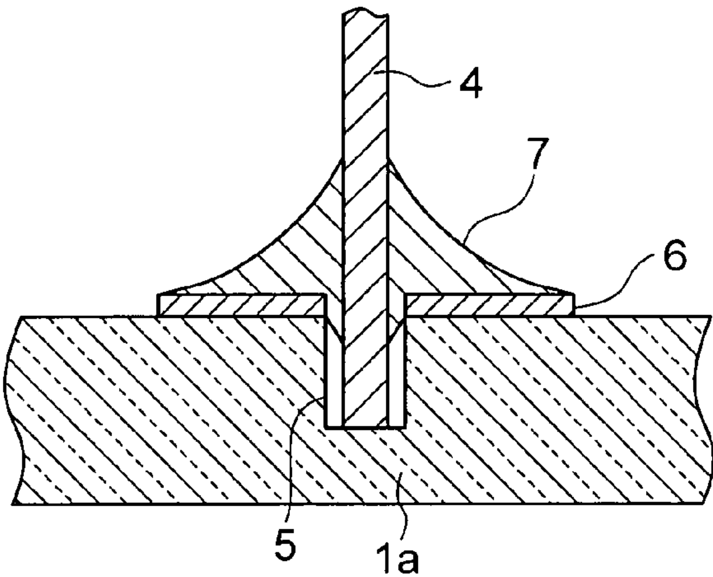
FIG. 3C PRIOR ART
