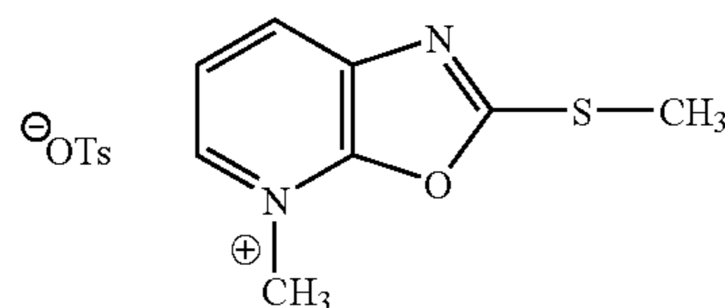
7-methyl-2-methylthioxazolo[5,4- b ]pyridinium tosylate
