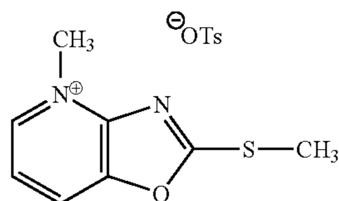
4-methyl-2-methylthioxazolo[4,5- b ]pyridinium tosylate
