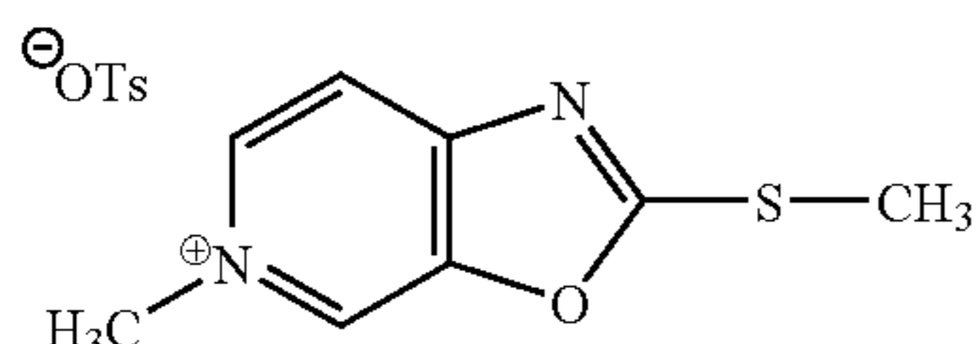
6-methyl-2-methylthioxazolo[5,4- c ]pyridinium tosylate
