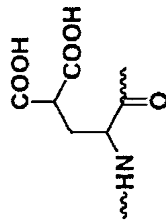
γ-carboxyglutamic acid (6)
