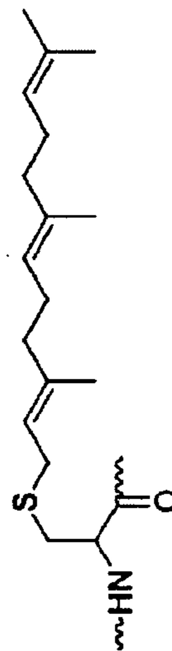
farnesylcysteine (4)
