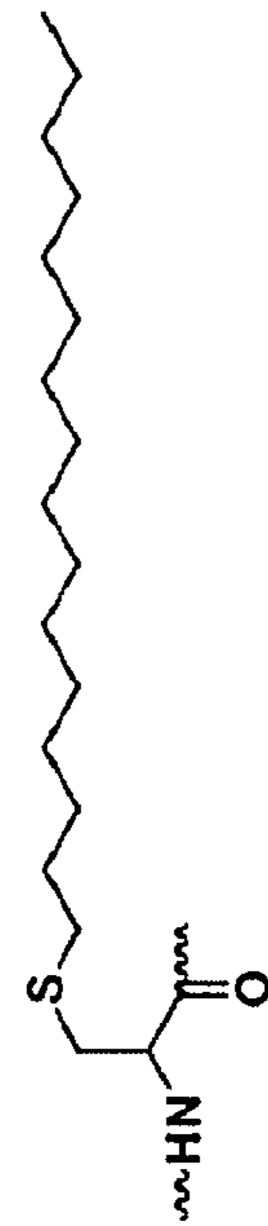
S-hexadecylcysteine (5)
