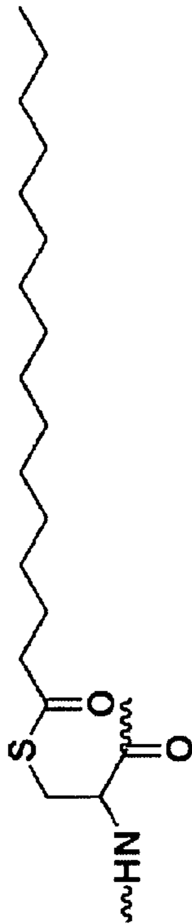
palmitoylcysteine (3)
