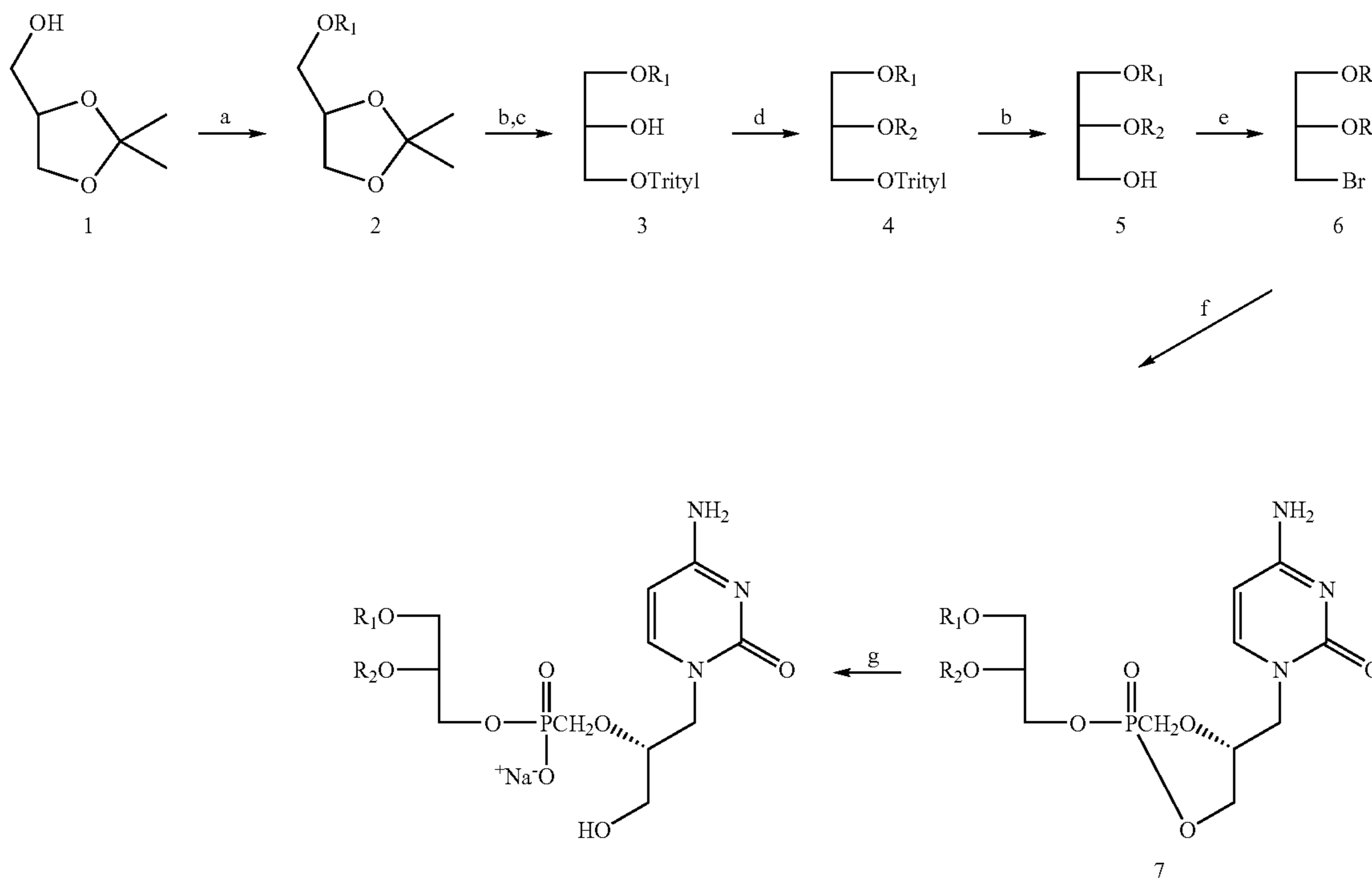
Scheme V
