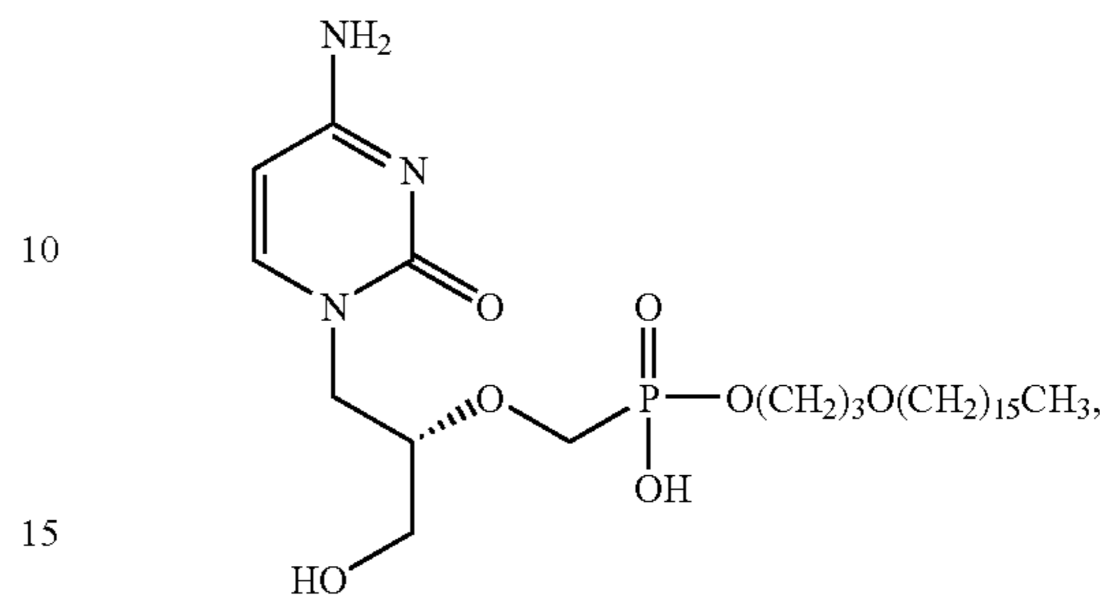
Formula II
