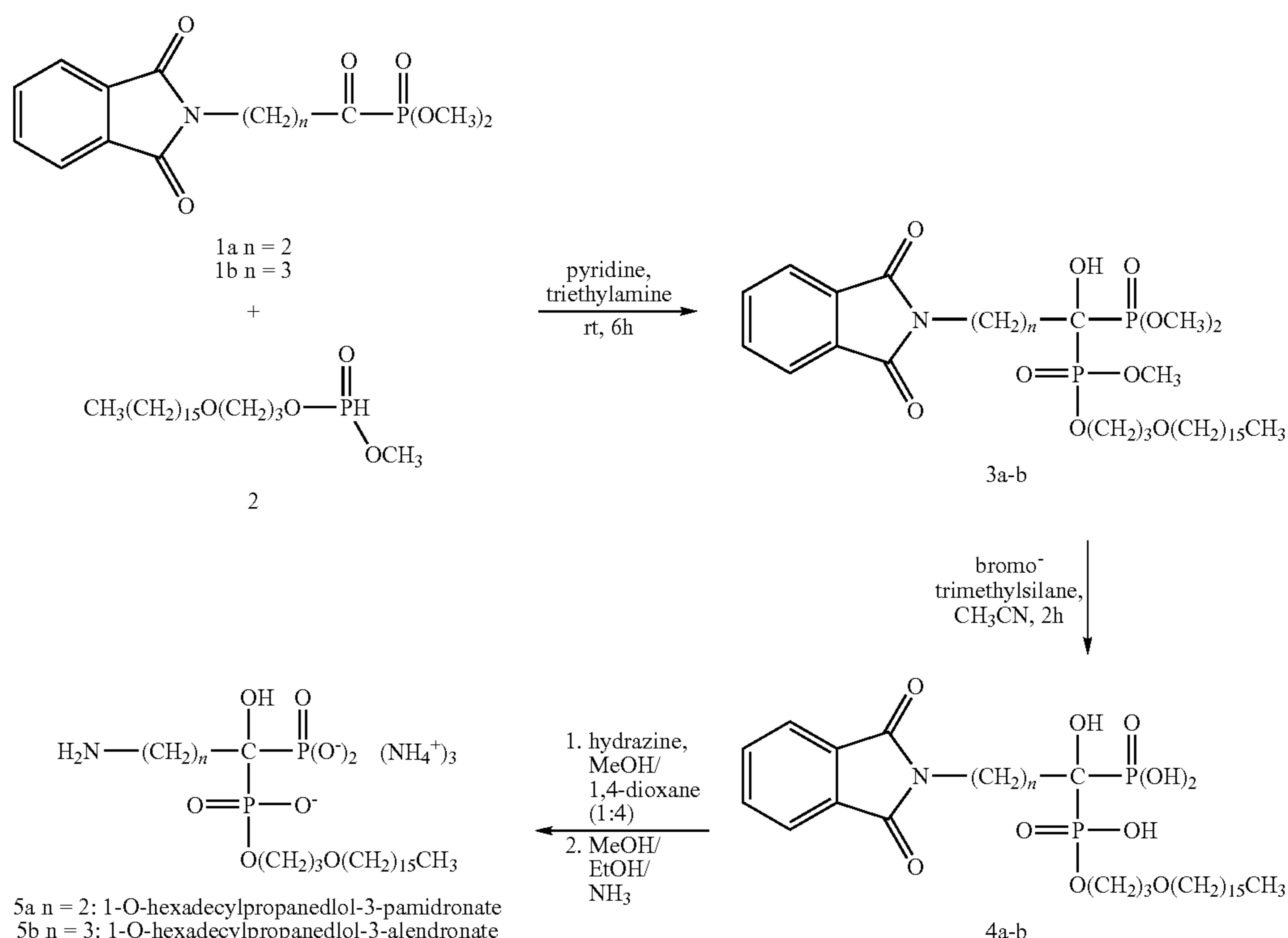
Scheme I
