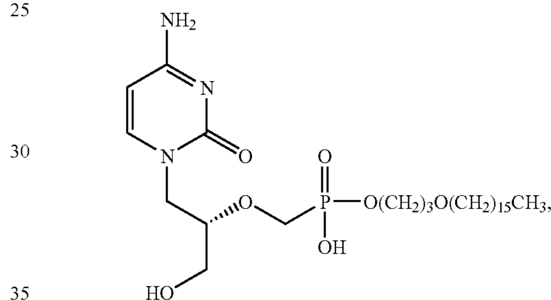
Formula A
