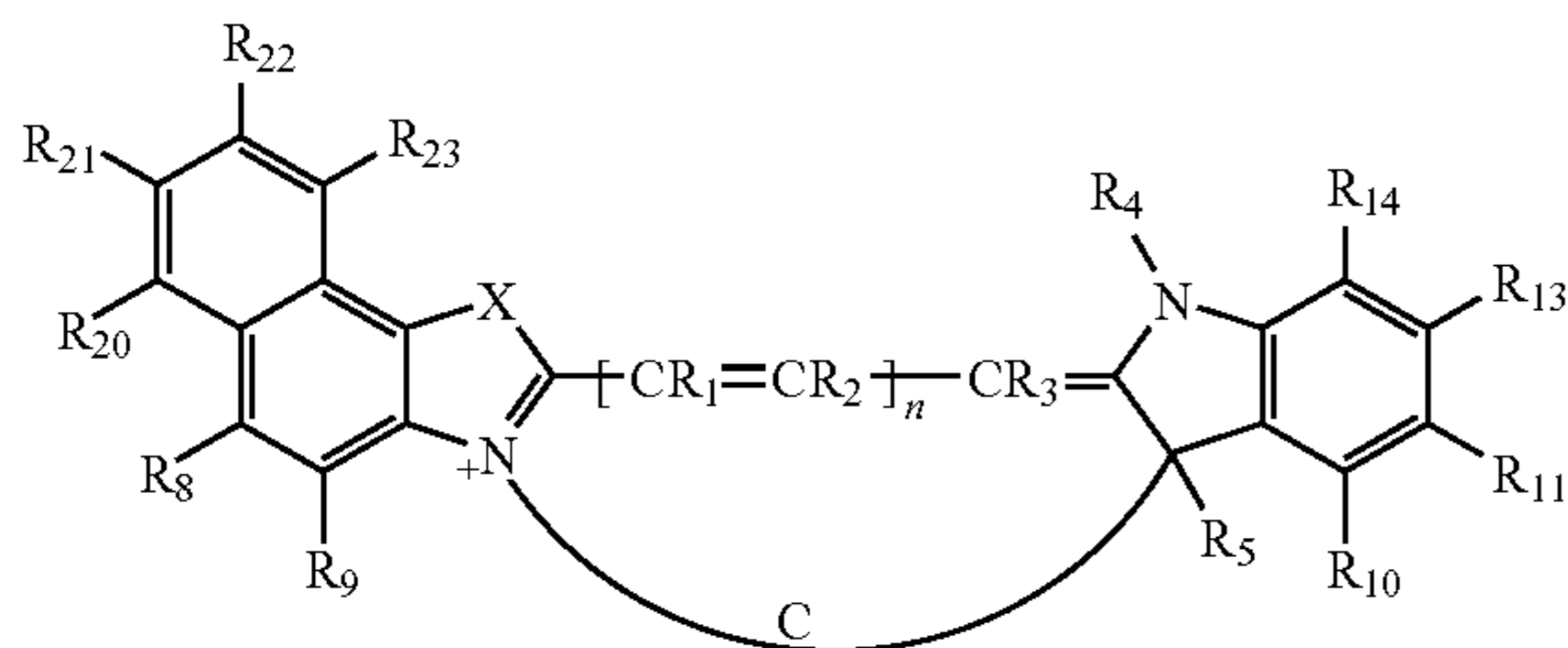
Formula VII
