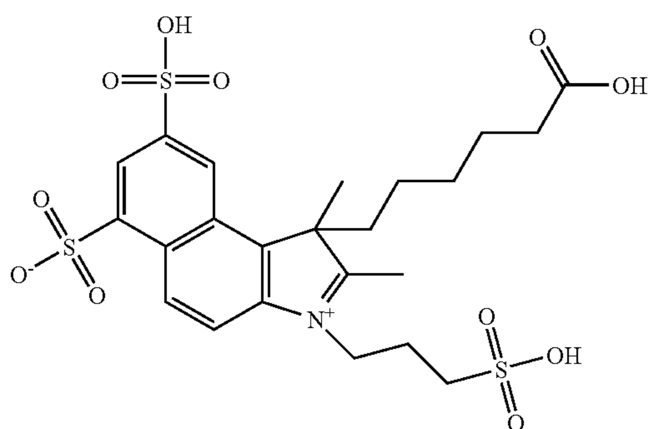
Compound 28
