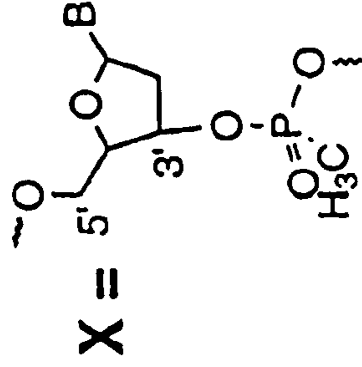
Methyl-phosphonate
