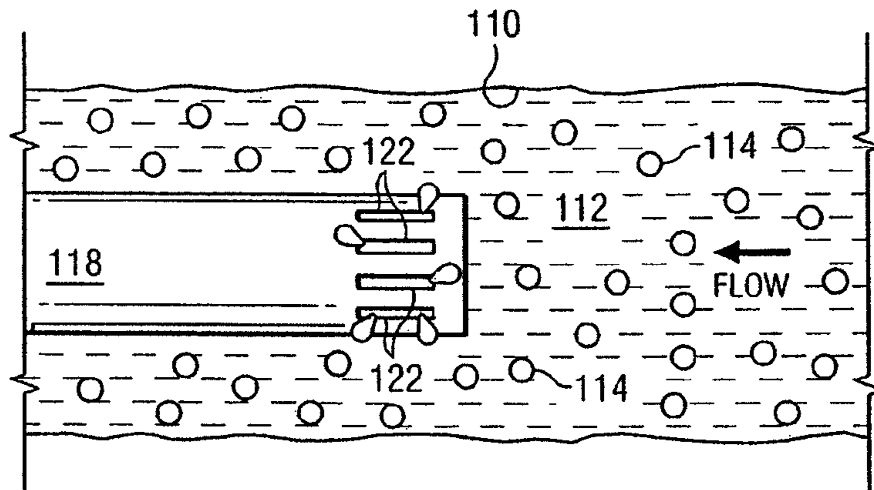
FIG. 1 PRIOR ART
