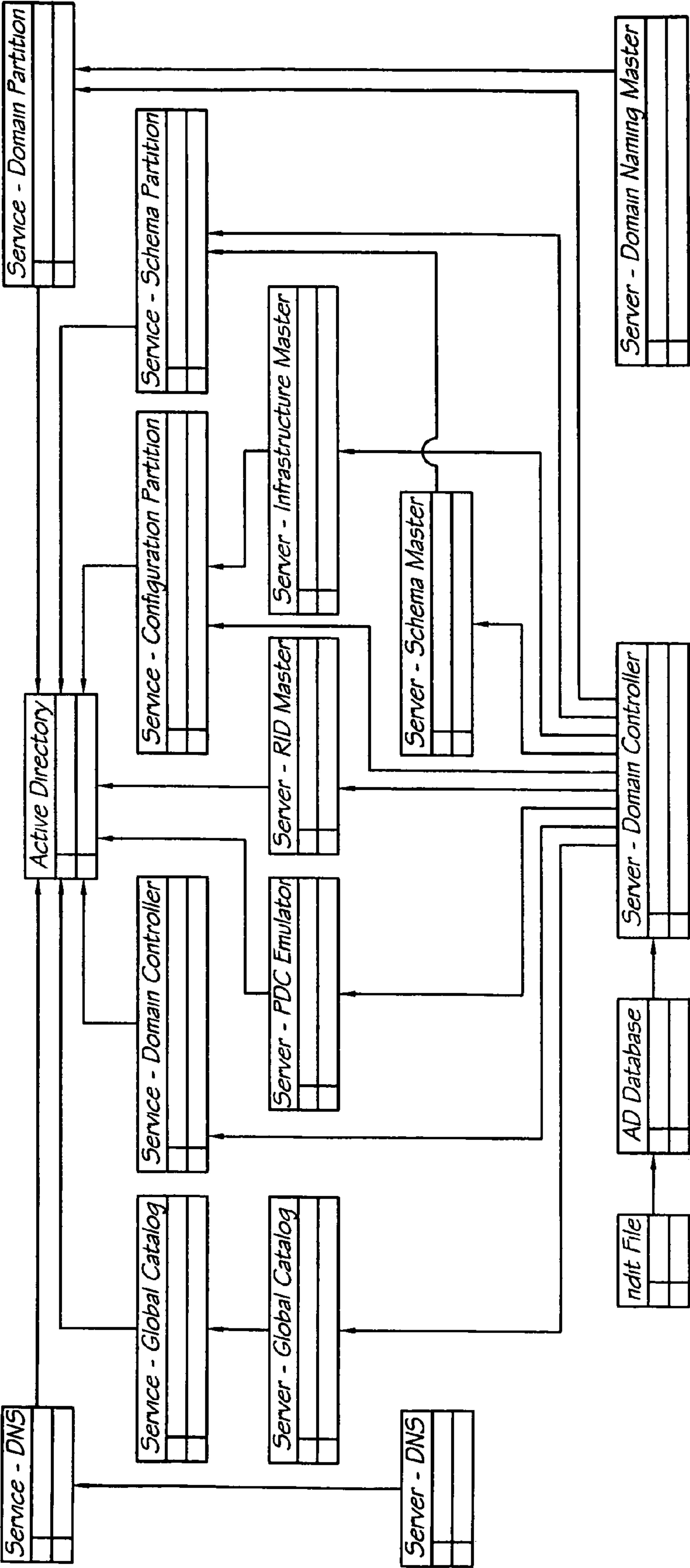
FIG. 30 Active Directory
