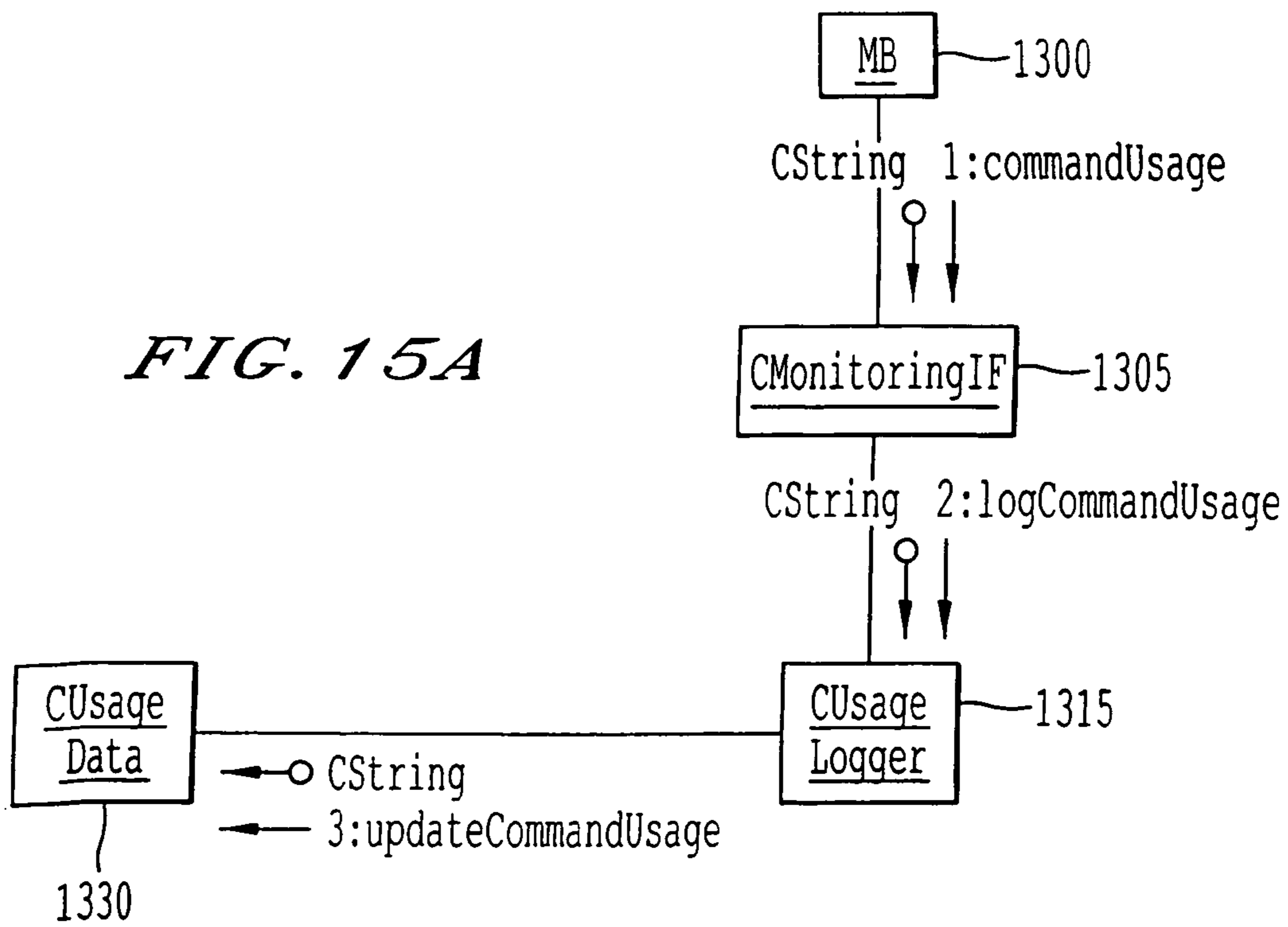
CommandUsage() Scenario
