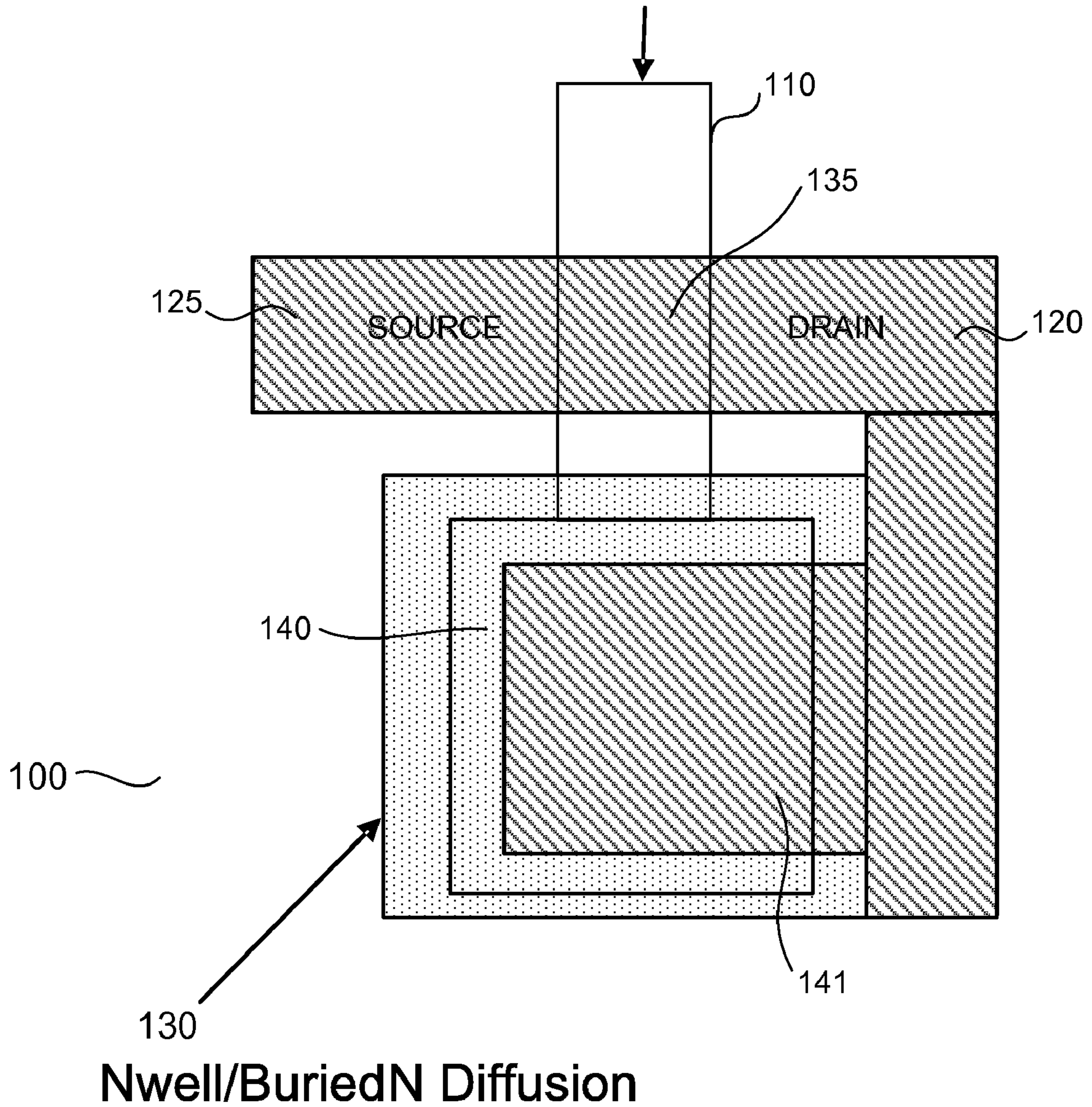
FIG. 1 Floating Gate
