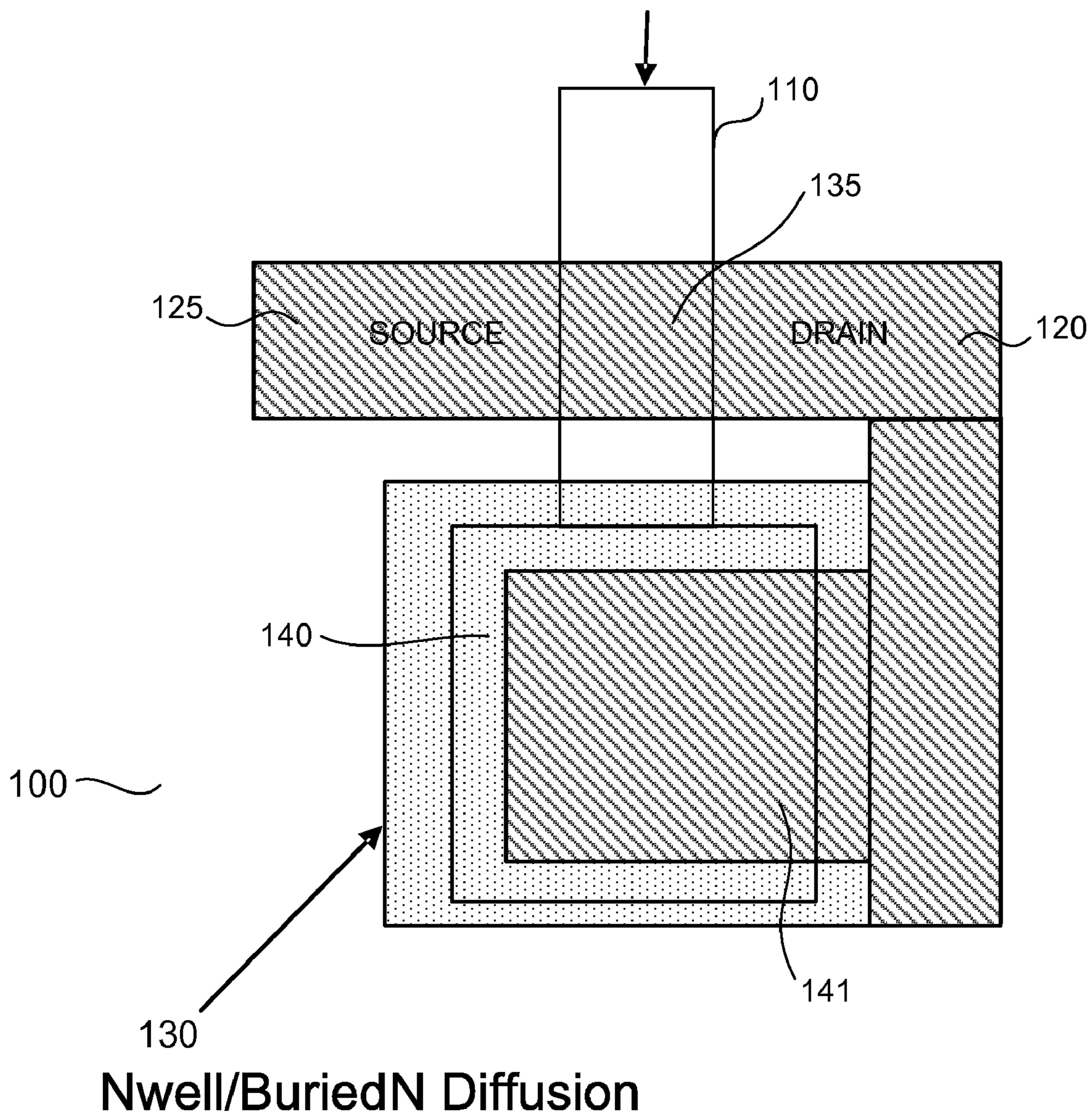
FIG. 1 Floating Gate
