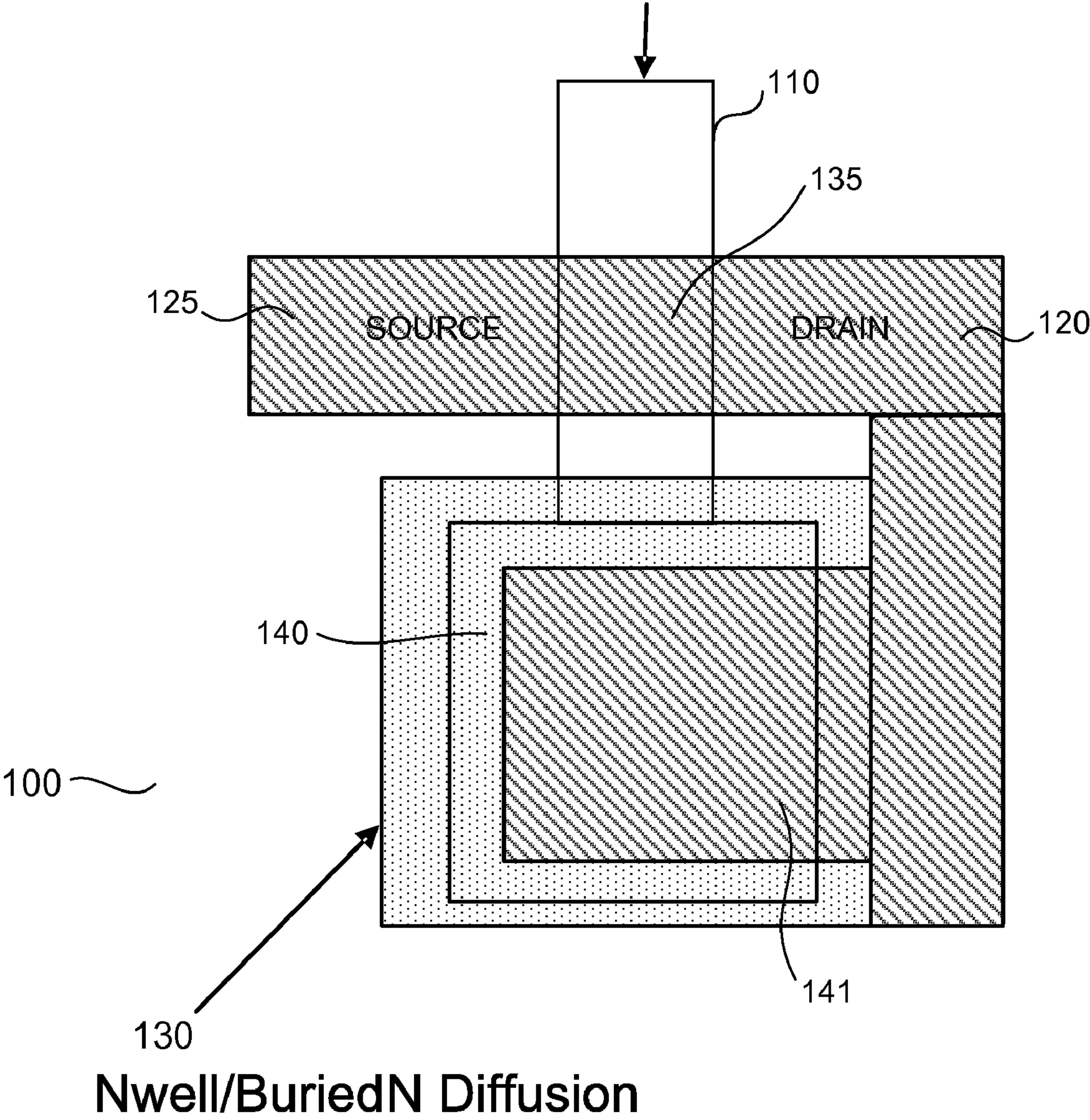
FIG. 1 Floating Gate
