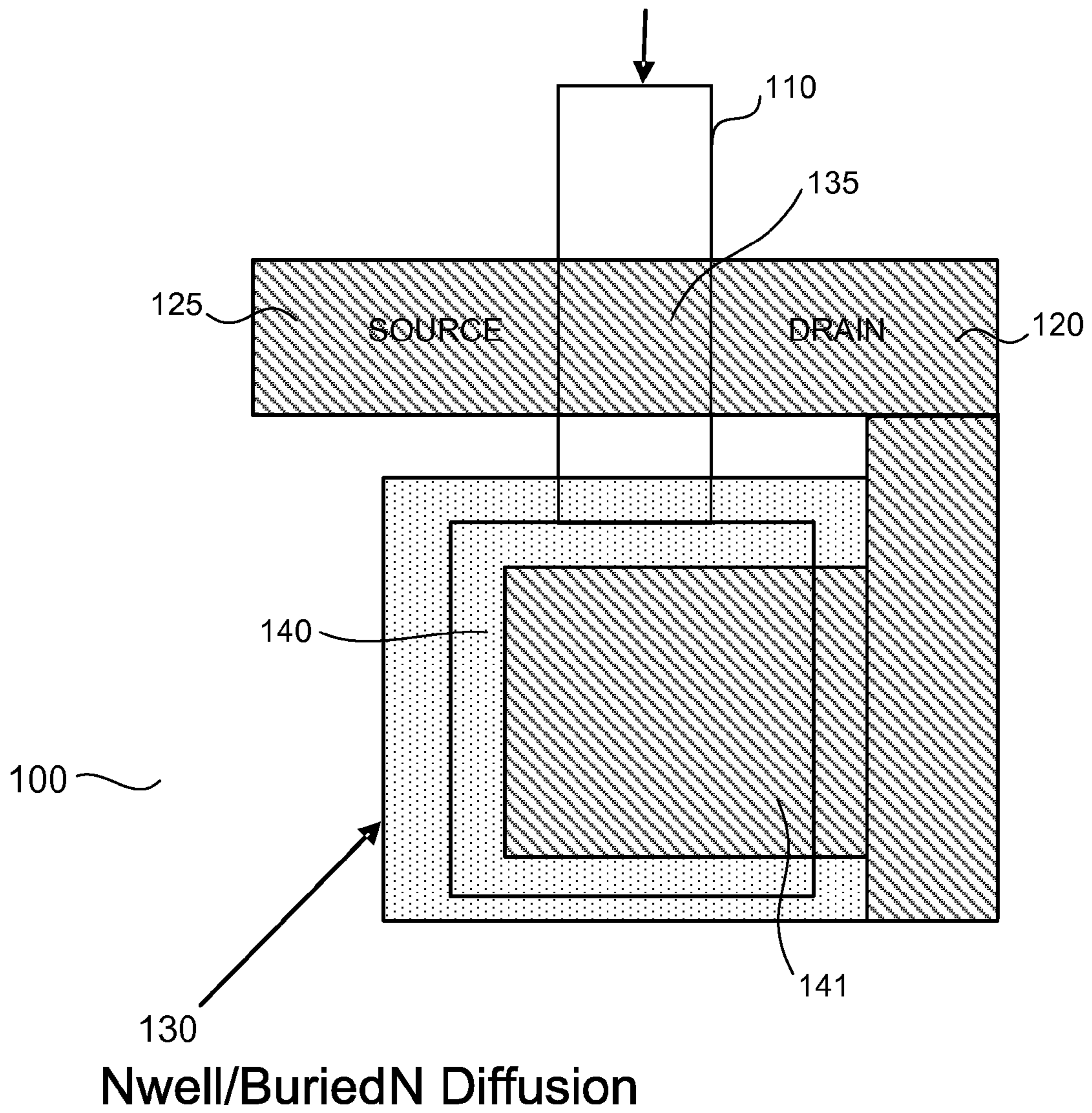
FIG. 1 Floating Gate
