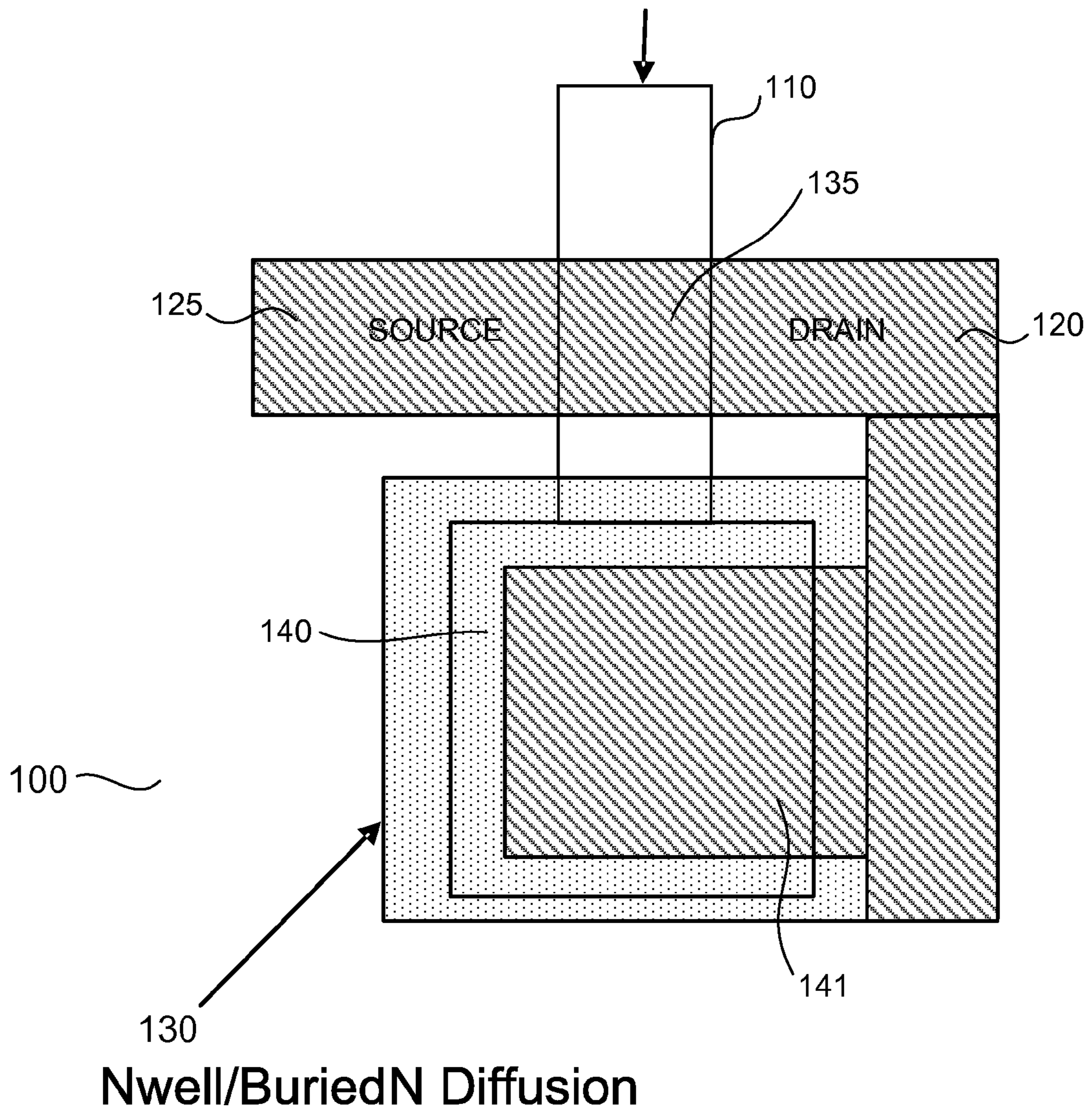
FIG. 1 Floating Gate
