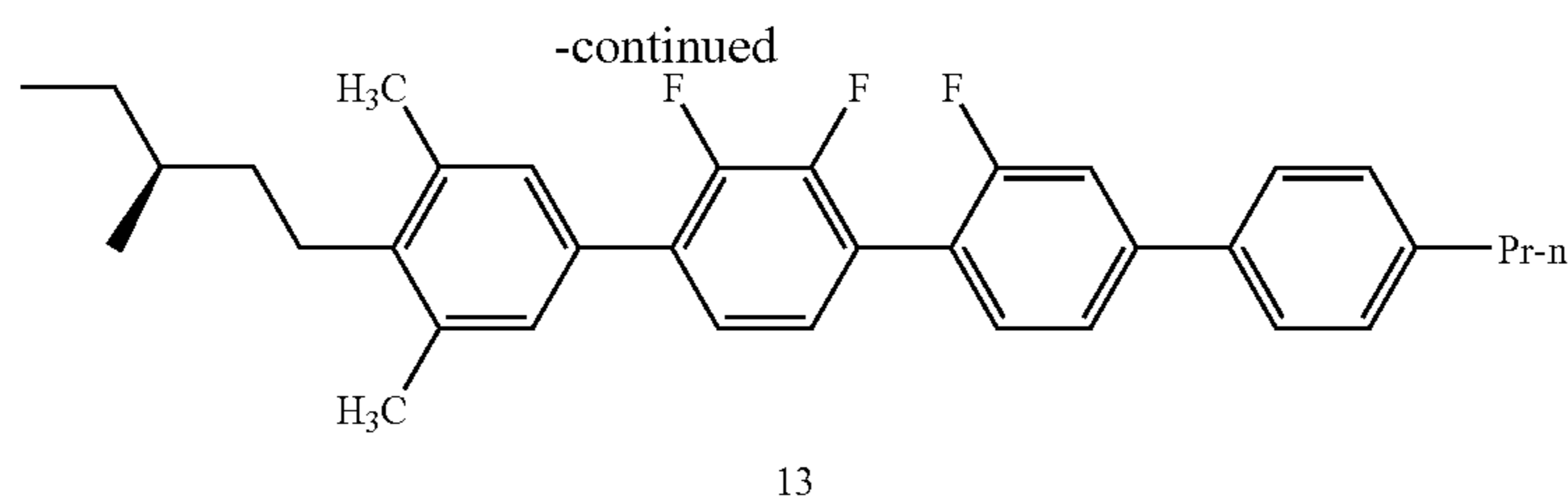
2',3',2''-Trifluoro-3,5-dimethyl-4-((S)-3-methylpentyl)-4'''-propyl-[1,4';1',1'';4'',1''']-quaterphenyl (13)
