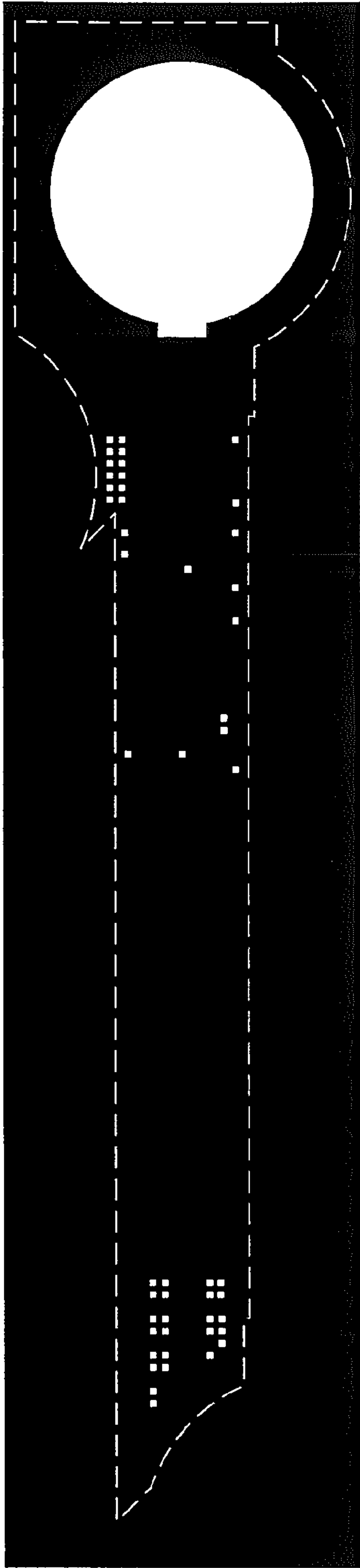
Via 1 mask
