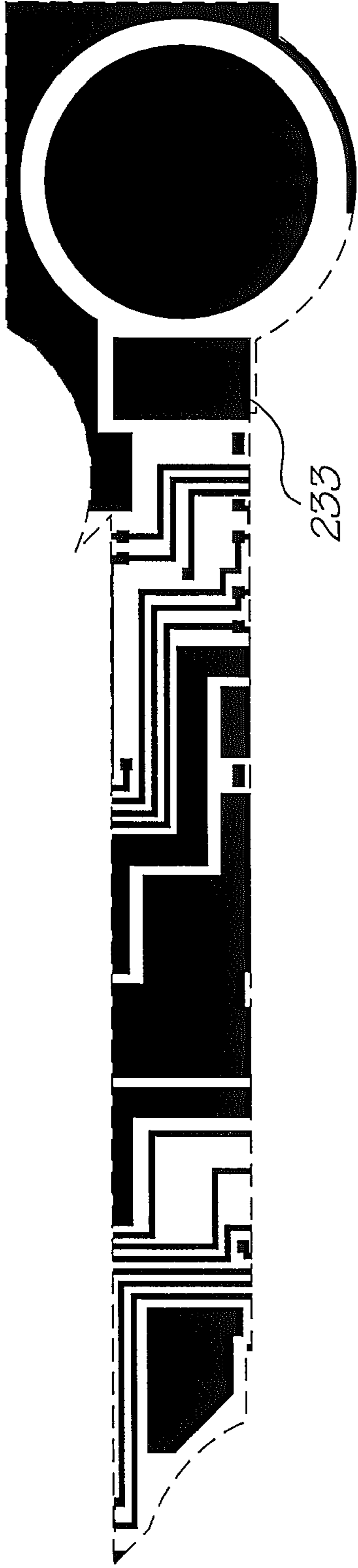
Metal 2 mask
