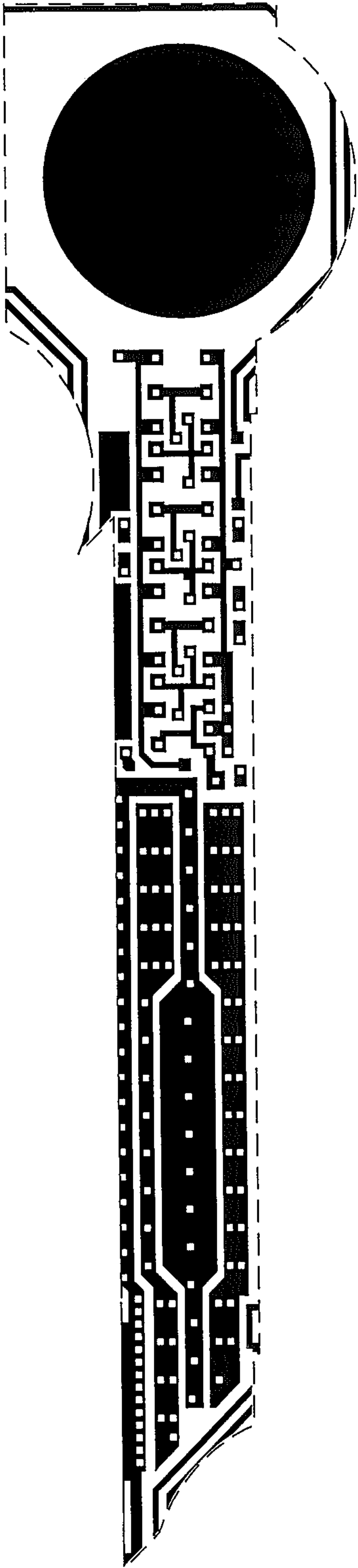
Metal 1 mask
