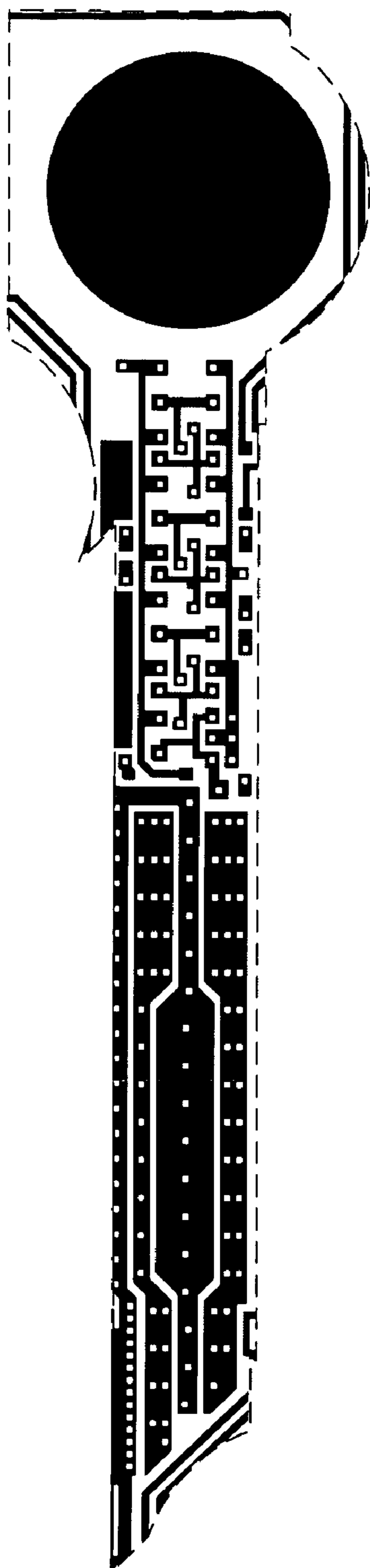
Metal 1 mask
