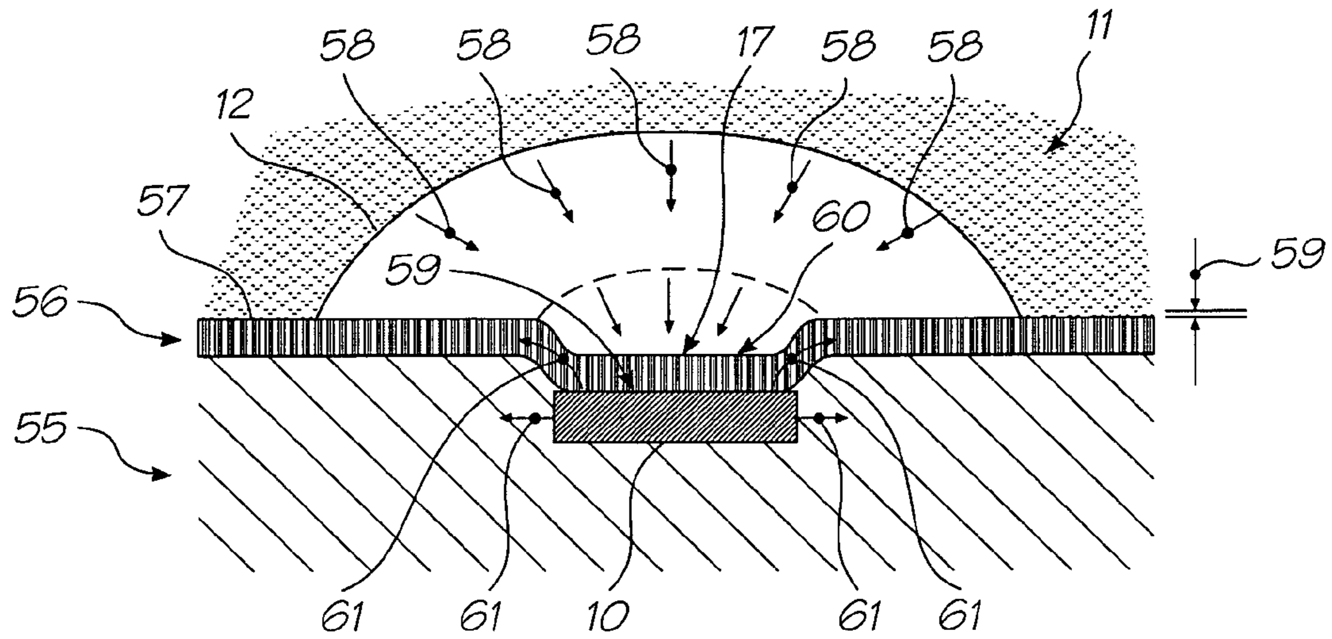
FIG. 47 (PRIOR ART)
