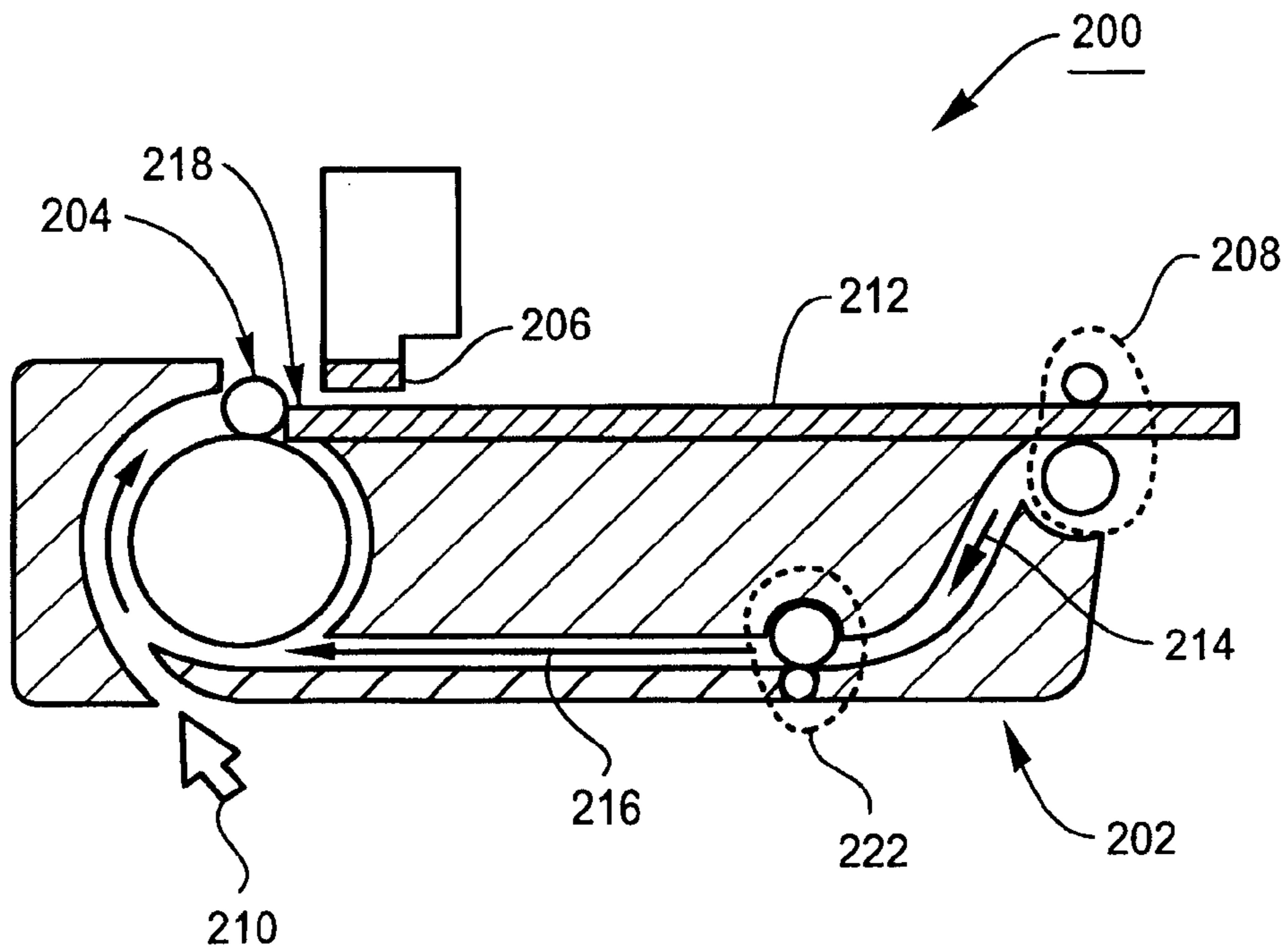
Figure 2 (Prior Art)
