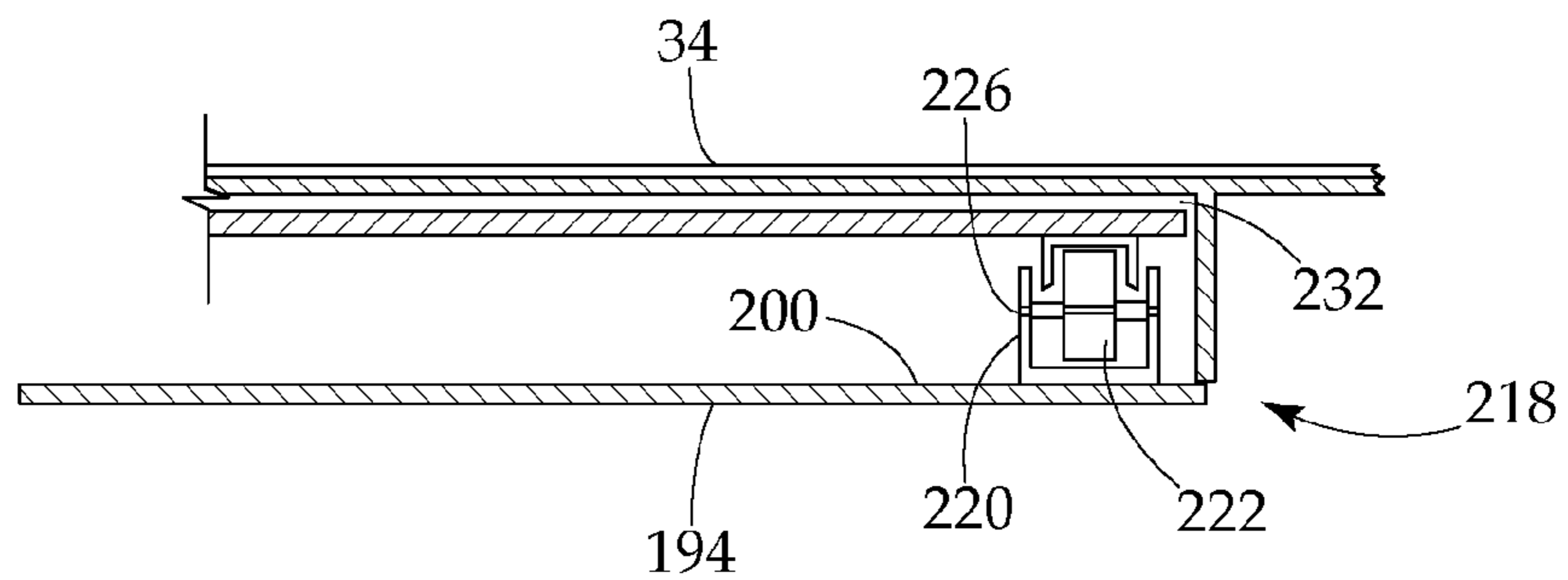
SECTION B-B
