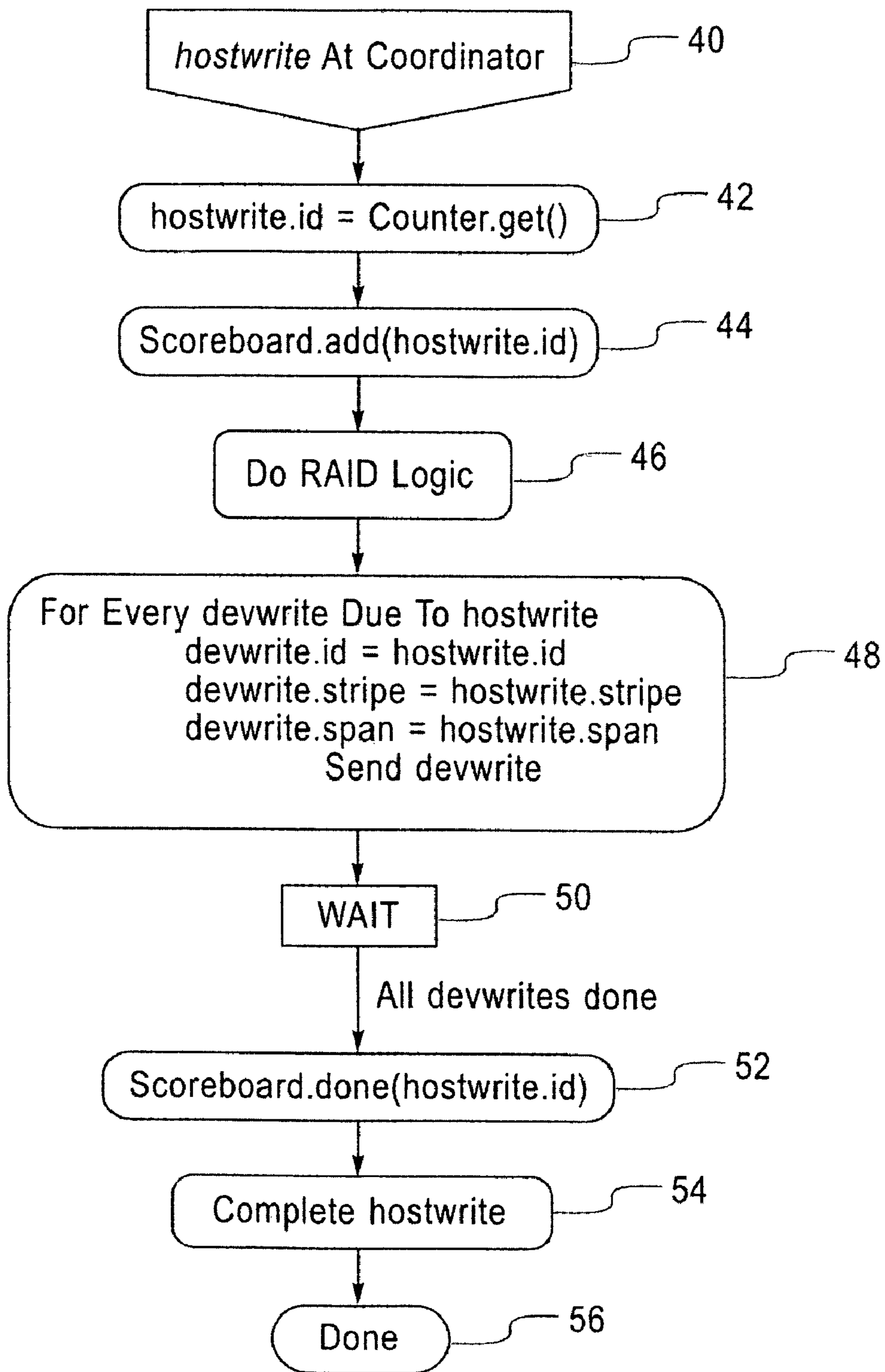
Host Write Logic FIG. 4
