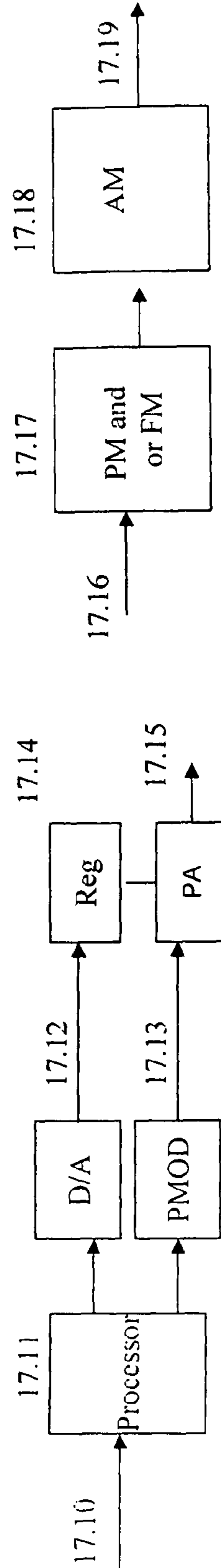
Fig. 17b A prior art Non Quadrature -Polar Modulator
