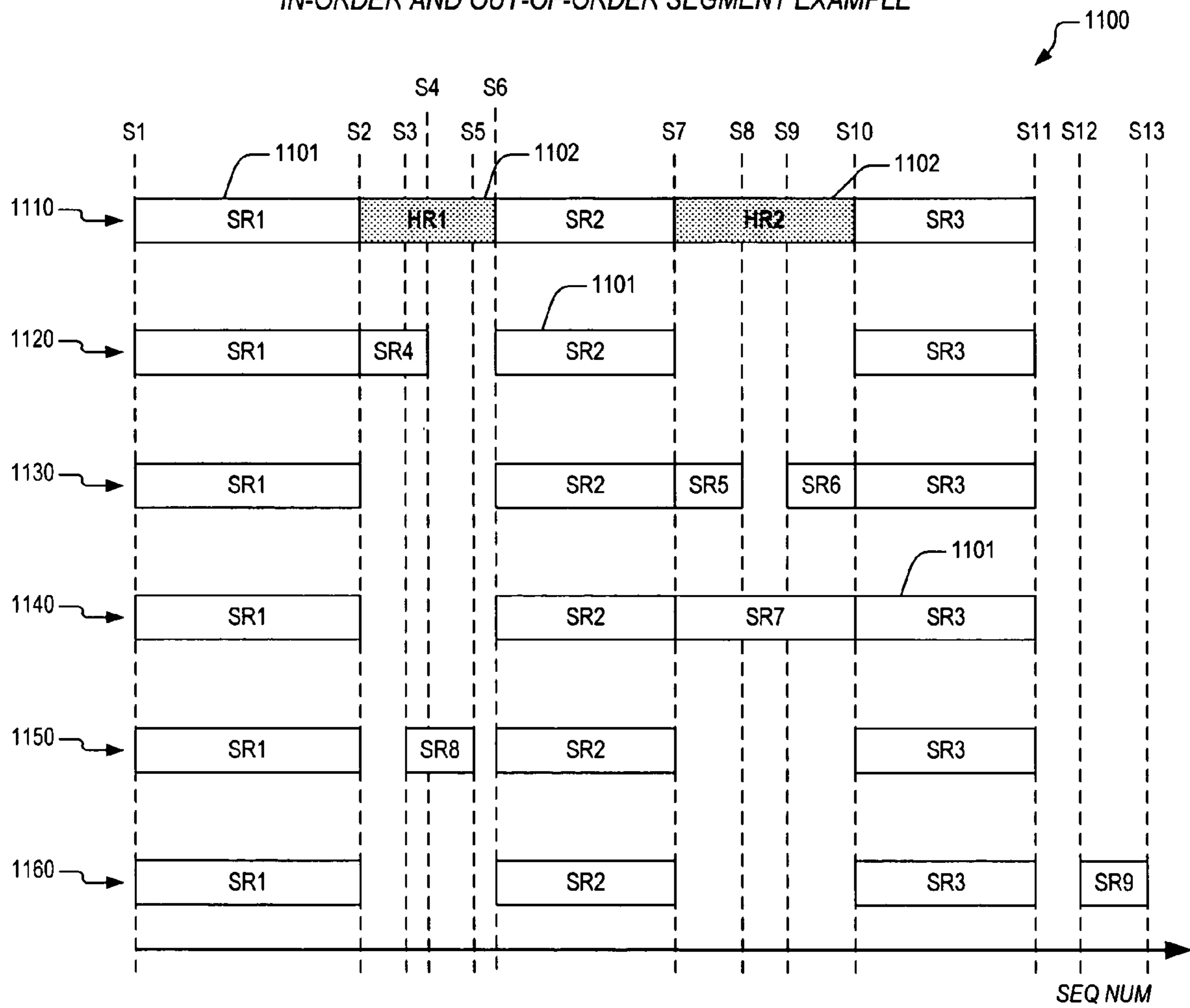
IN-ORDER AND OUT-OF-ORDER SEGMENT EXAMPLE
