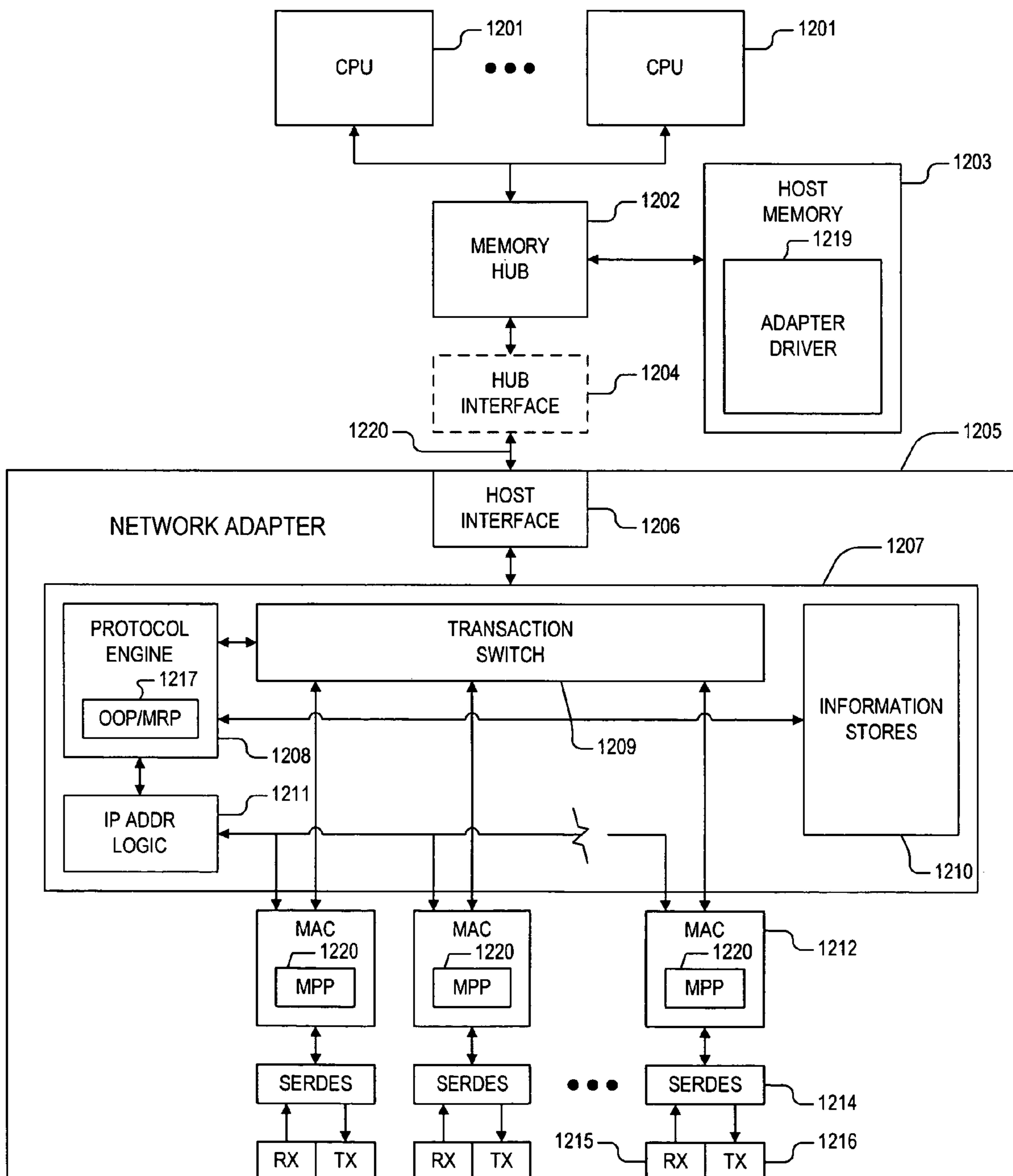
RDMA-ENABLED SERVER FEATURING SPECULATIVE MPA CRC CALCULATIONS 1200
