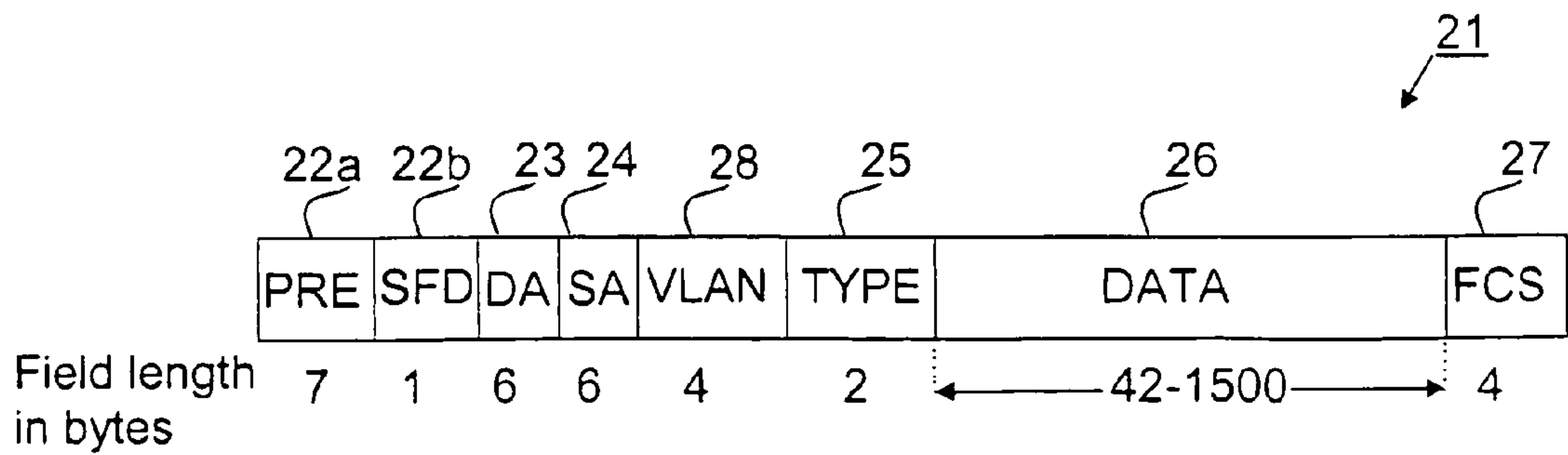
Fig. 2 (PRIOR ART)
