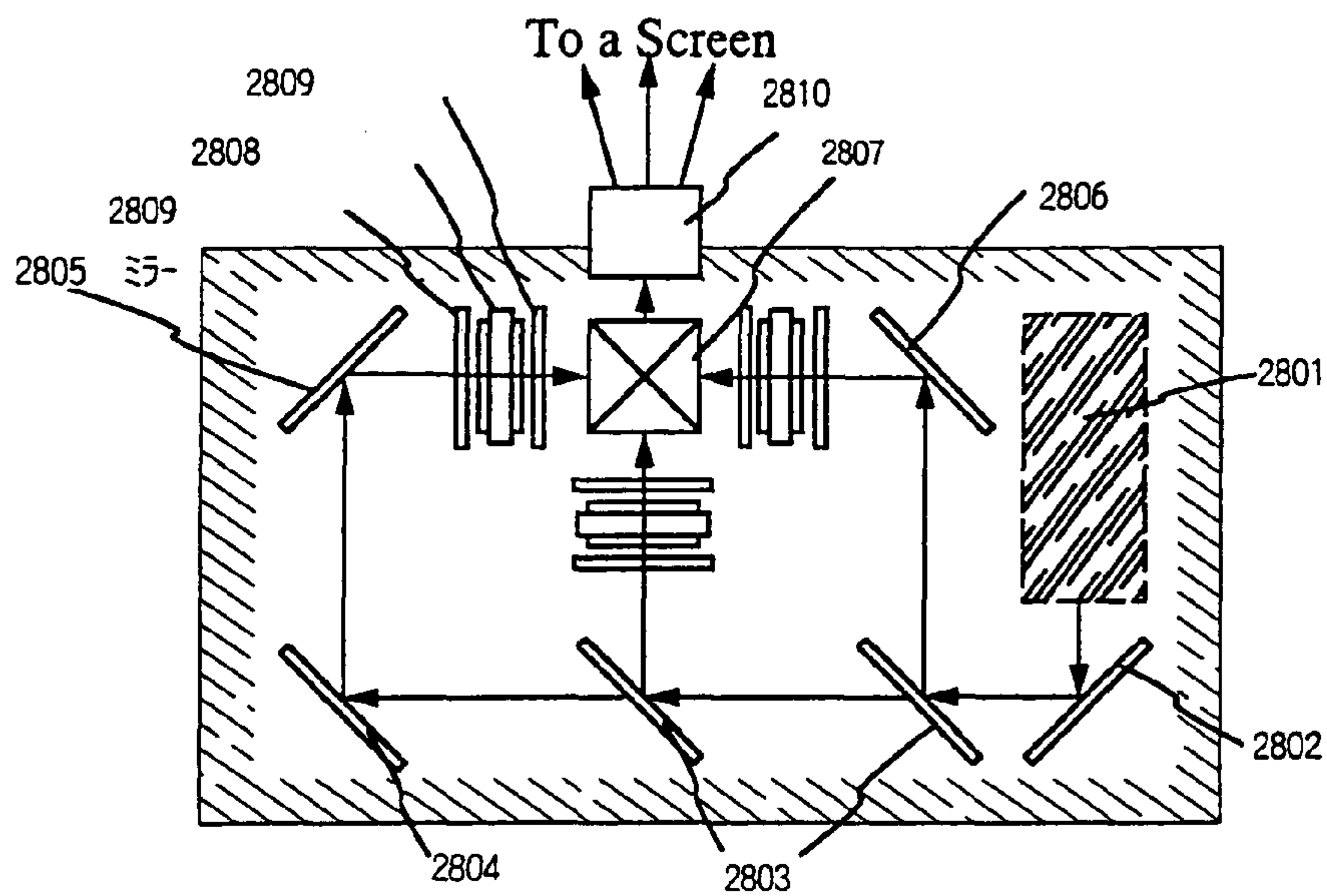
Fig. 18(C) Display Device(3 panel projector)
