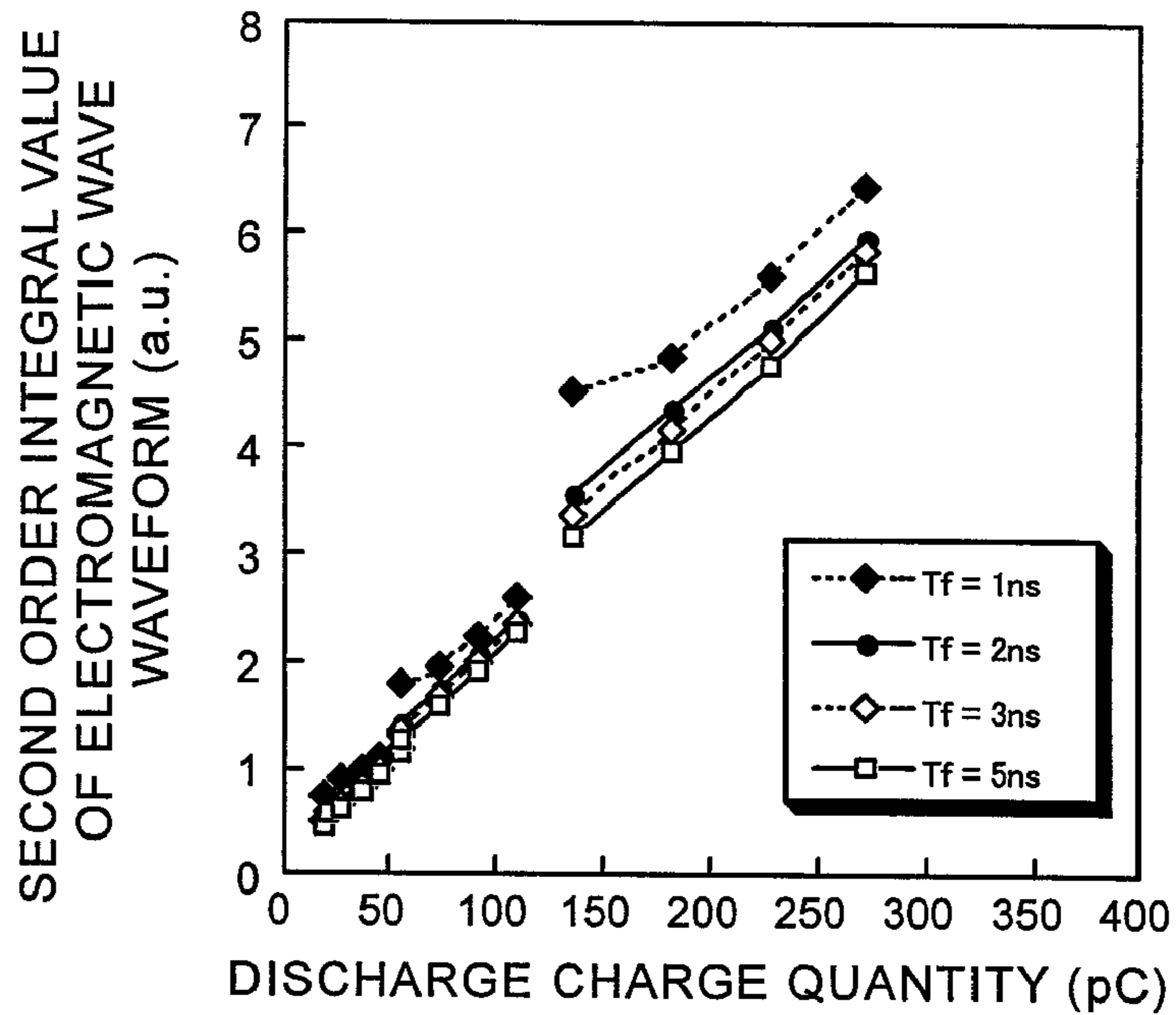
(a) SENSOR POSITION : 0°
