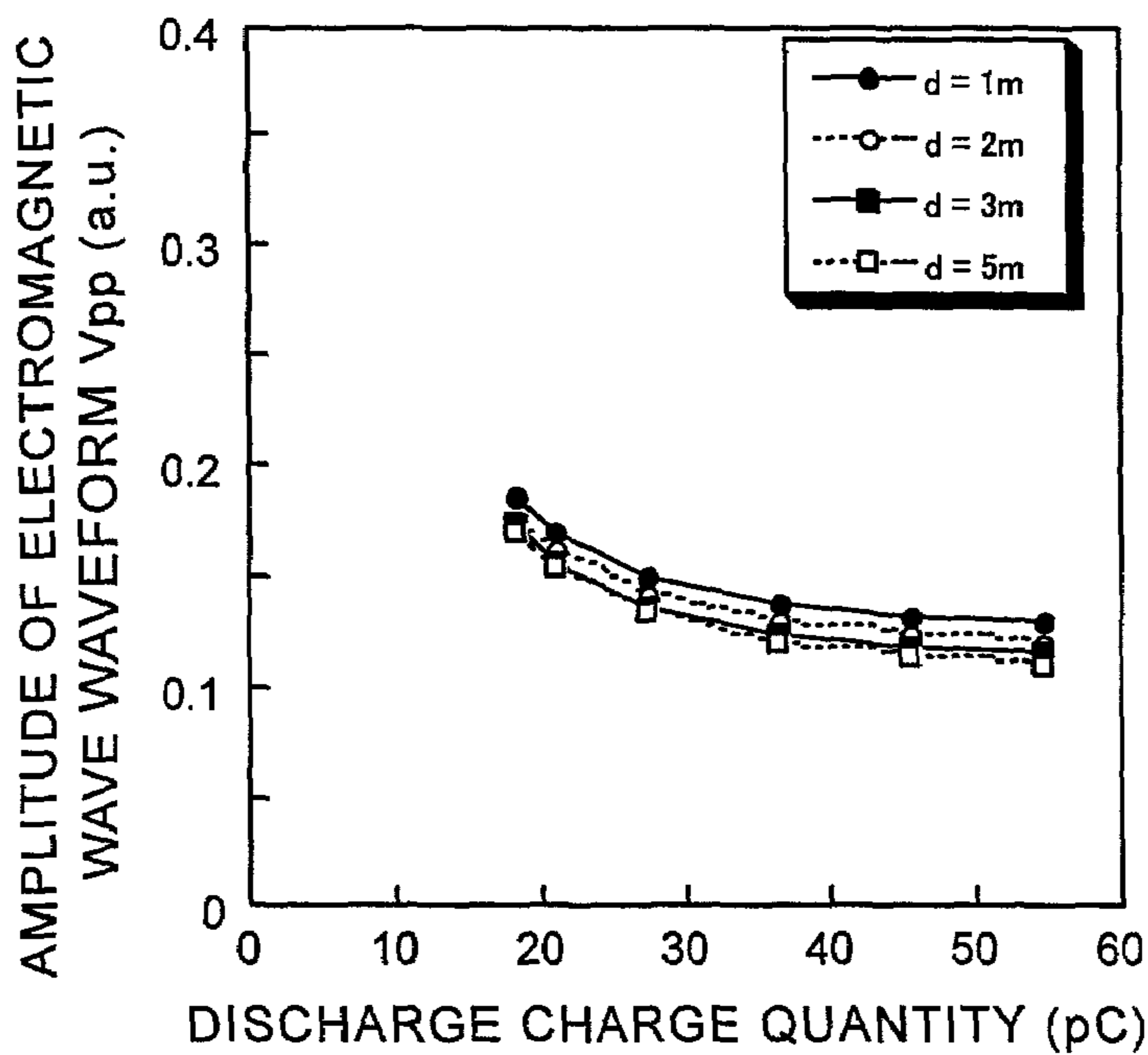
(b) SENSOR POSITION : 90^\circ
