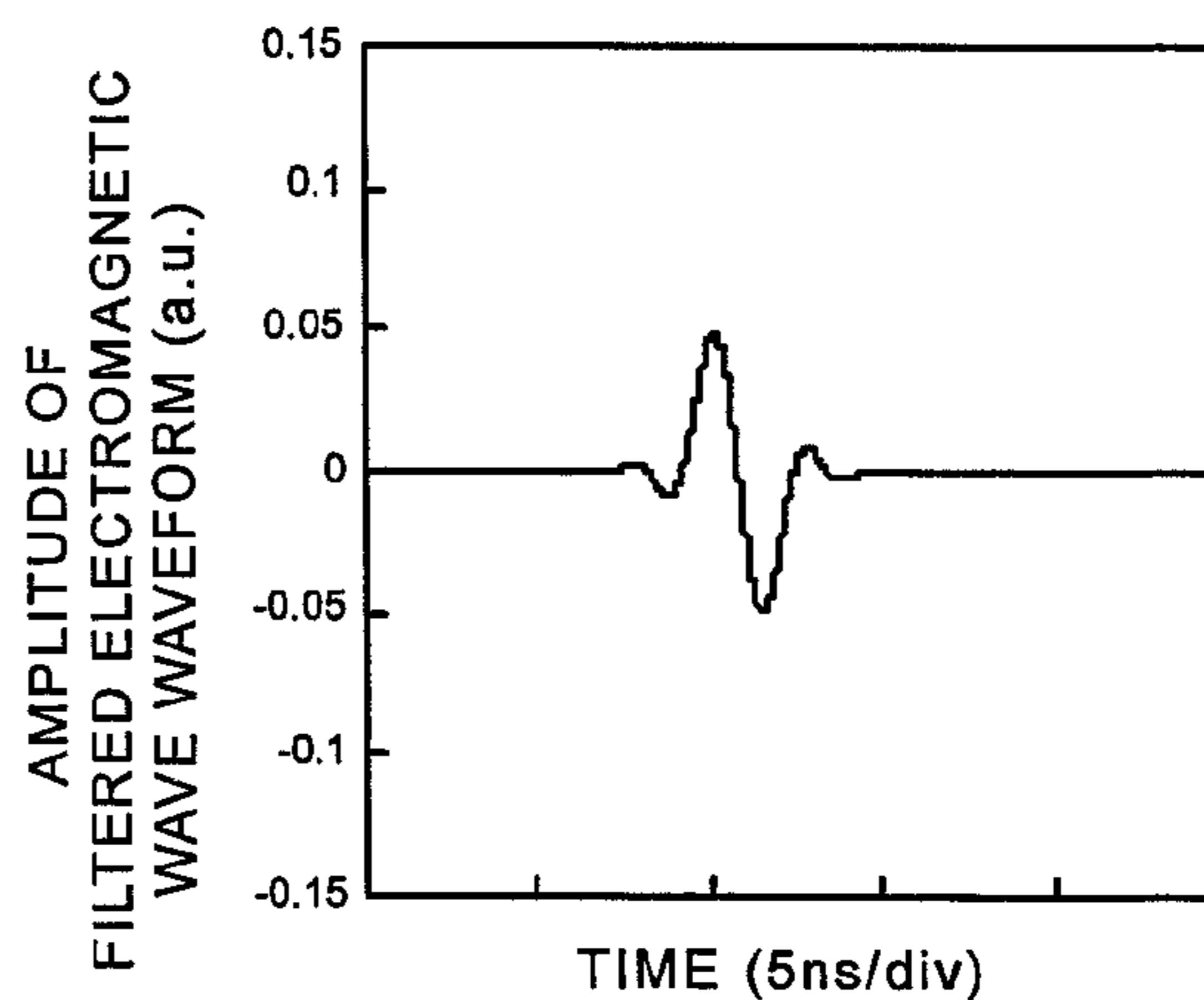
(b) EXTRACTION OF TEM MODE COMPONENT THROUGH FILTERING
