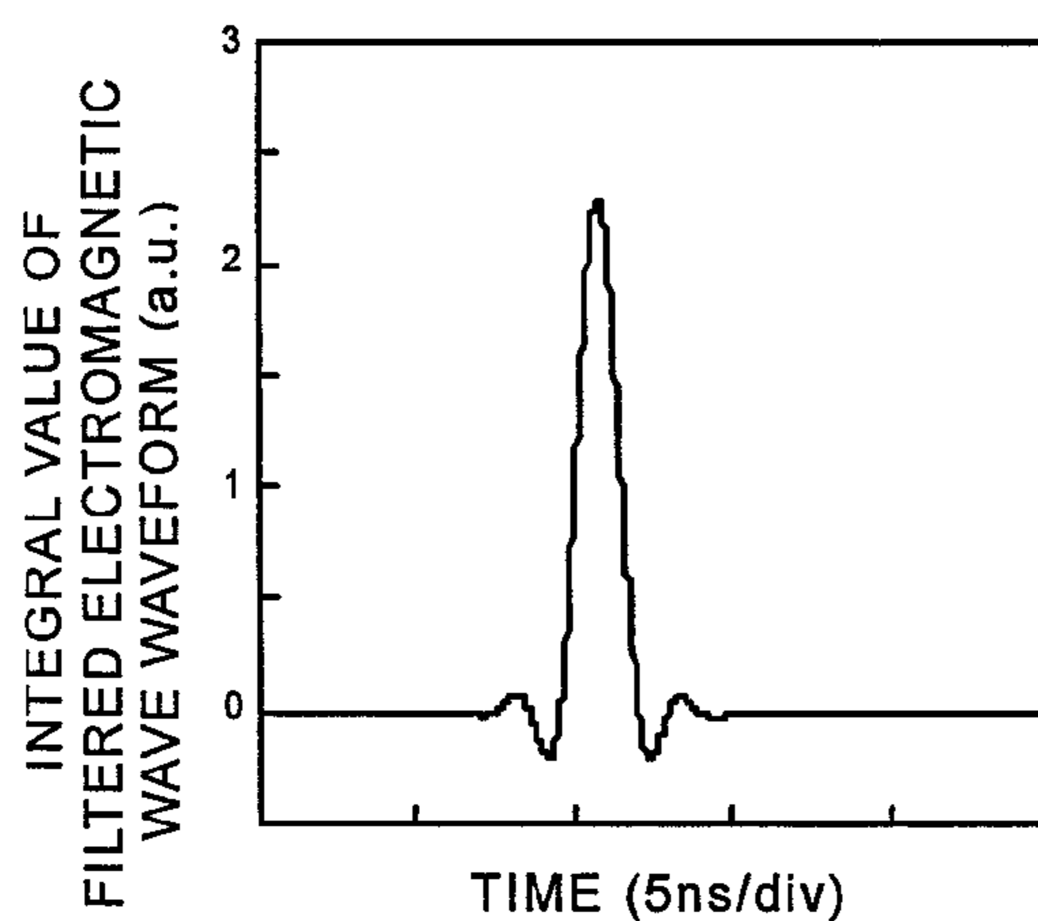
(c) FIRST ORDER INTEGRAL VALUE OF (b)
