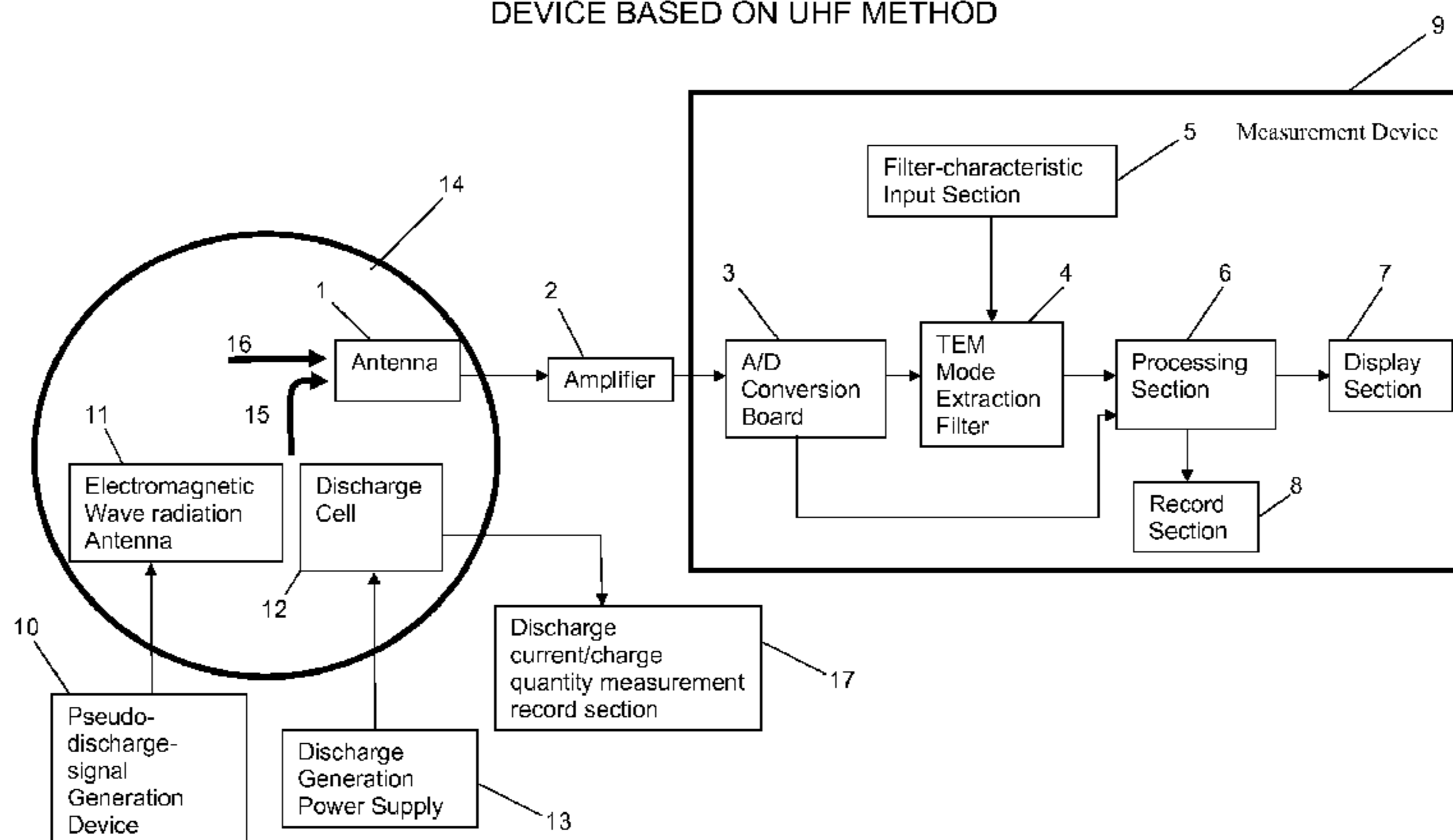
CHARGE QUANTITY MEASUREMENT DEVICE BASED ON UHF METHOD
