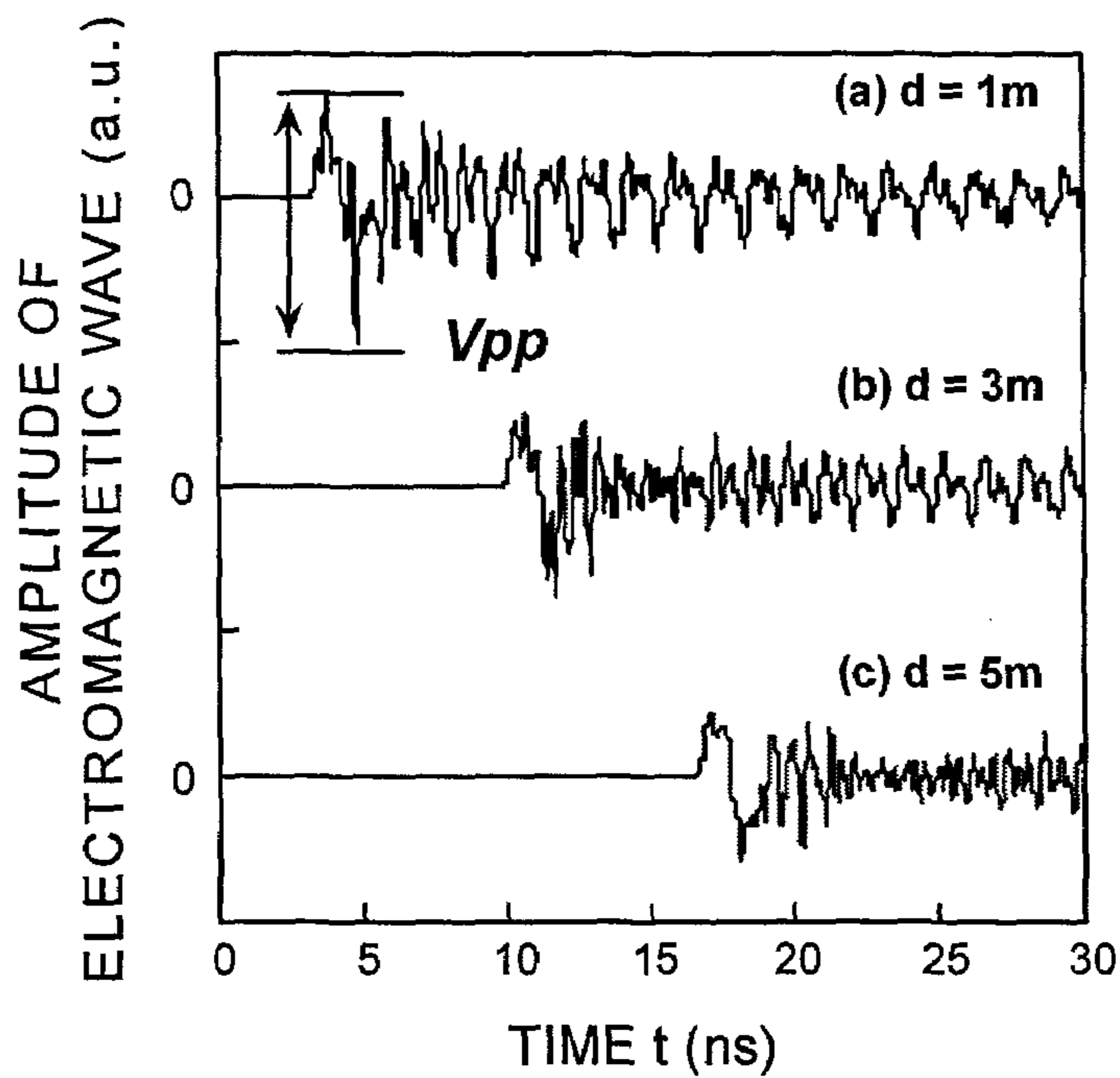
(a) 66 kV-CLASS MODEL GIS
