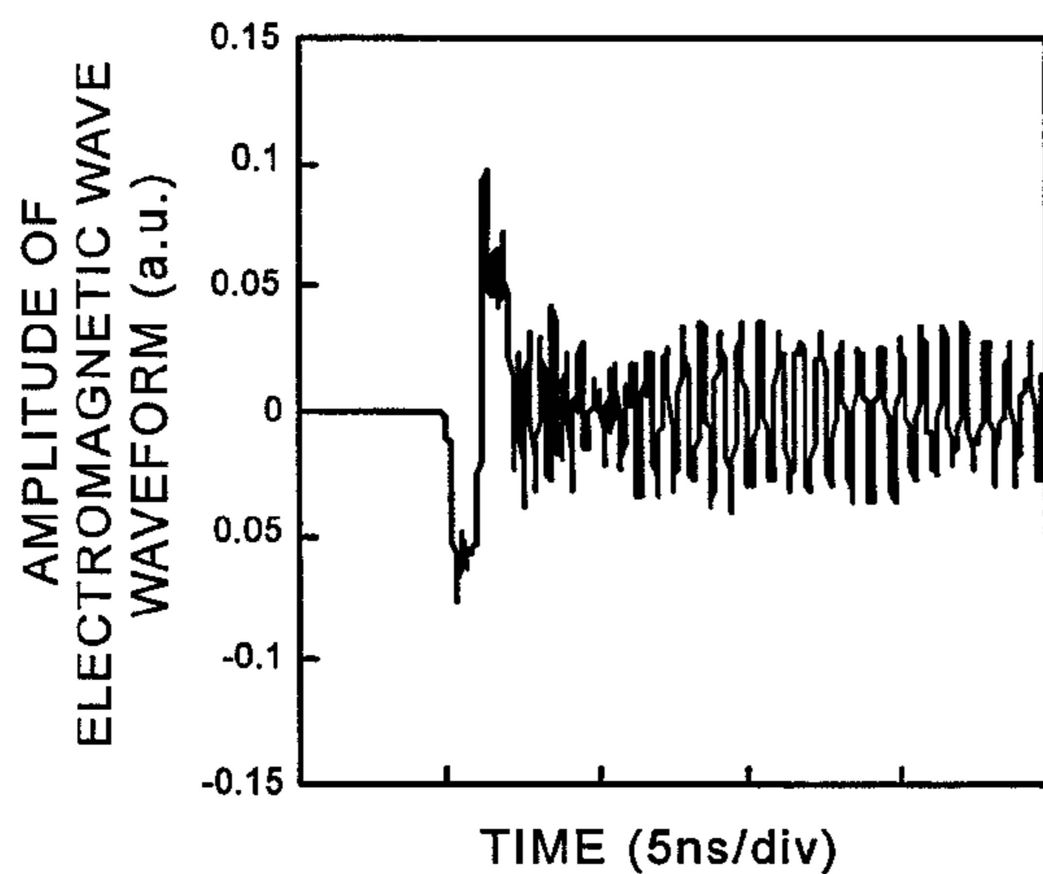
(a) RADIATED ELECTROMAGNETIC WAVE WAVEFORM
