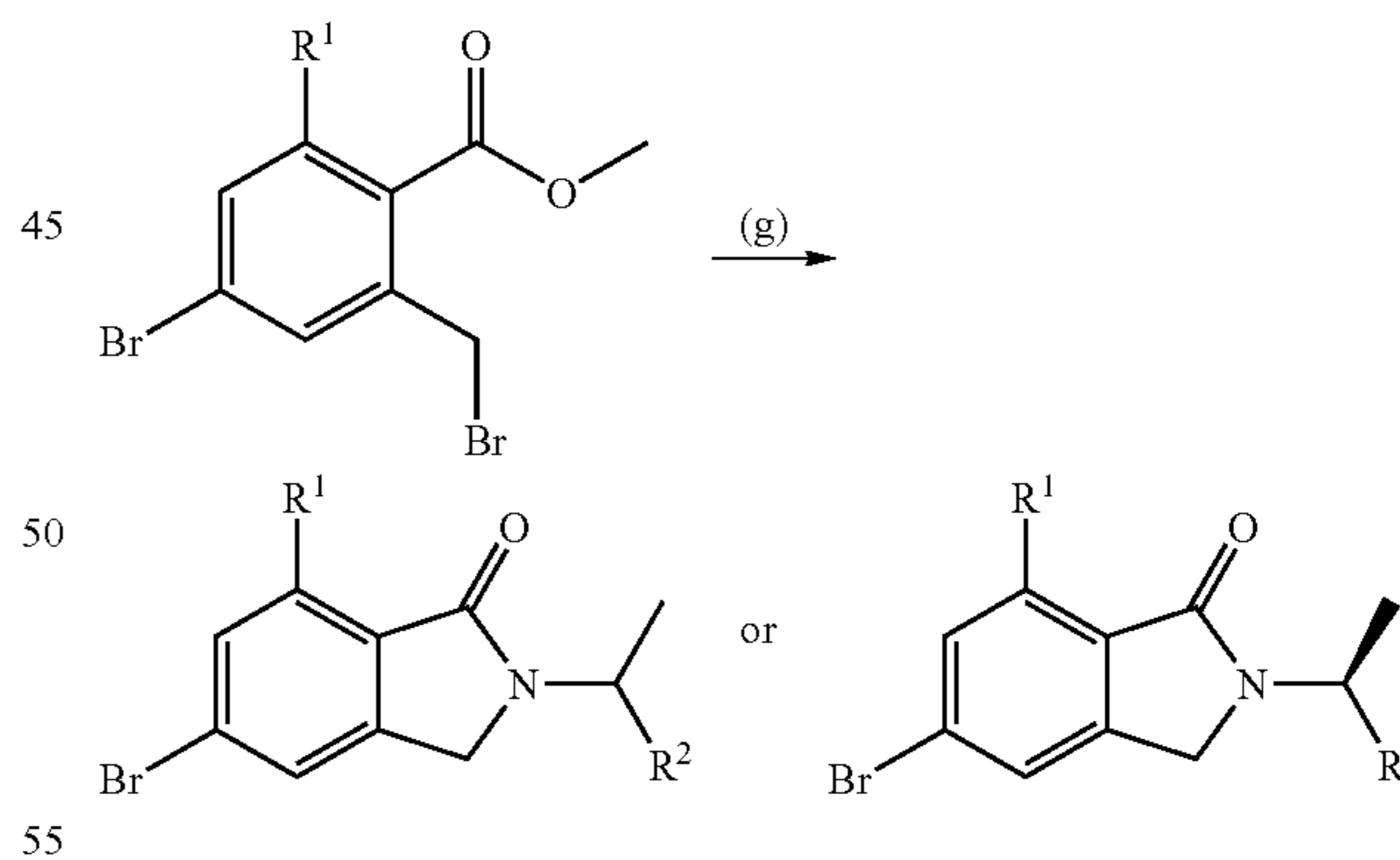
Scheme 2:
