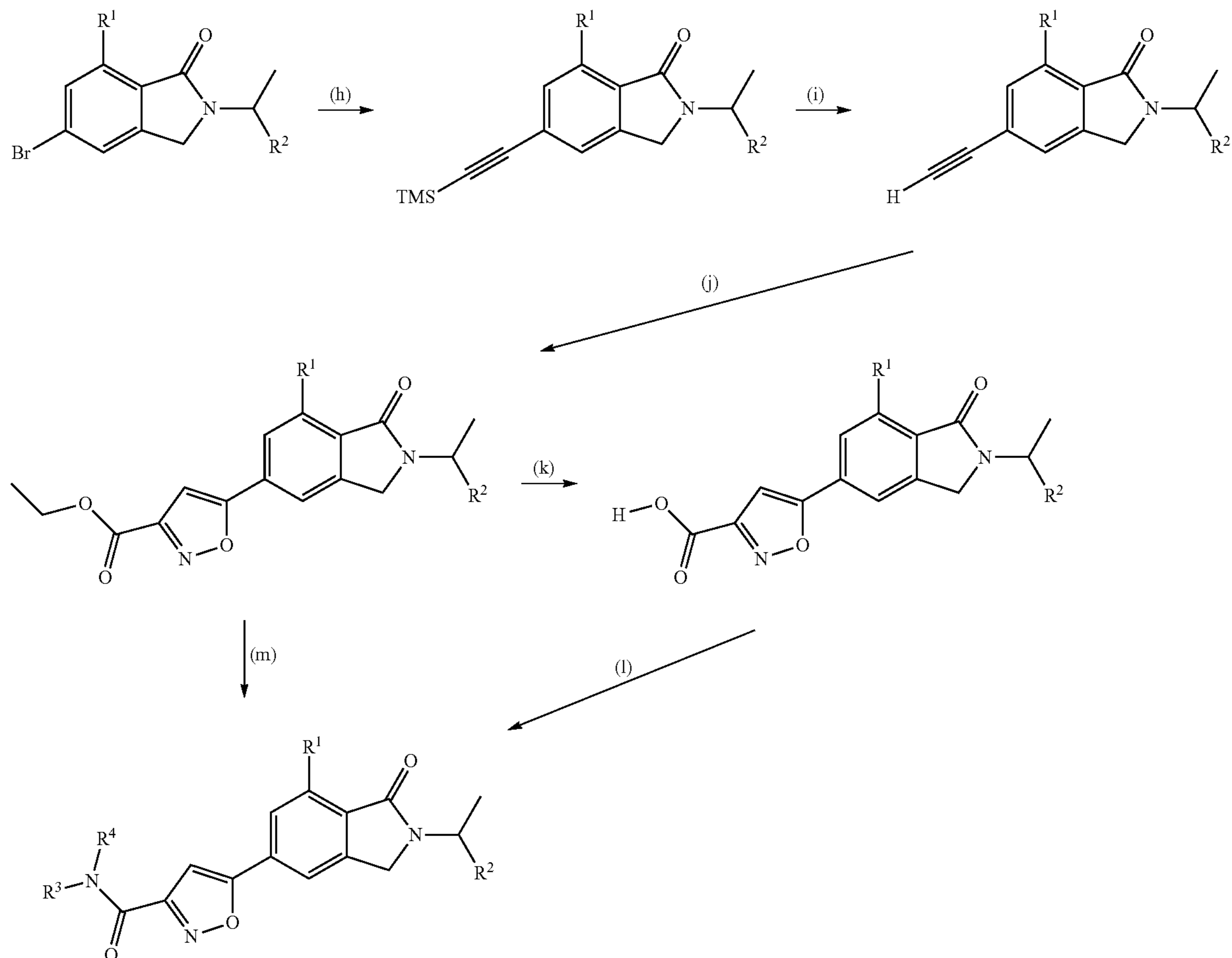
Scheme 3:
