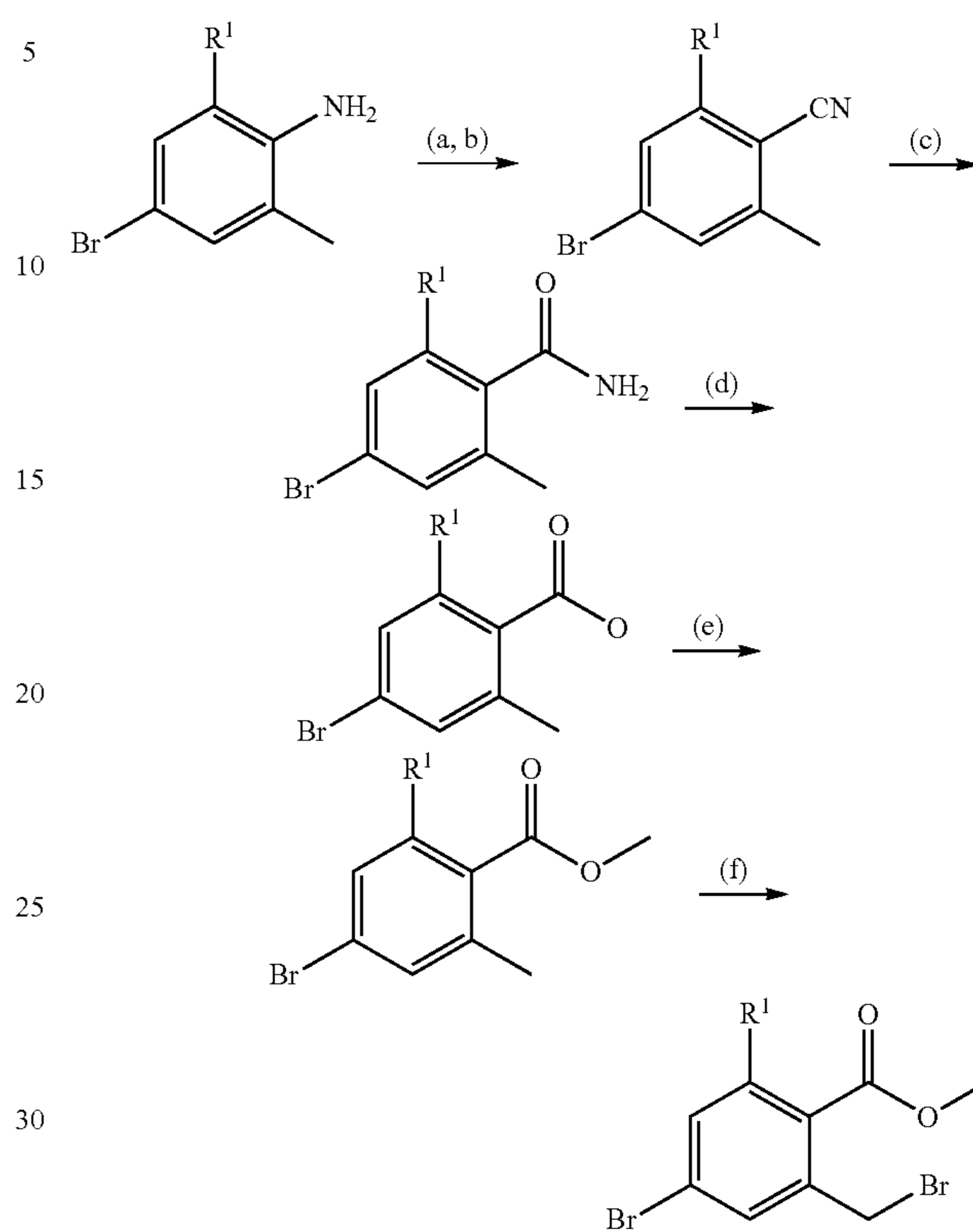
Scheme 1:
