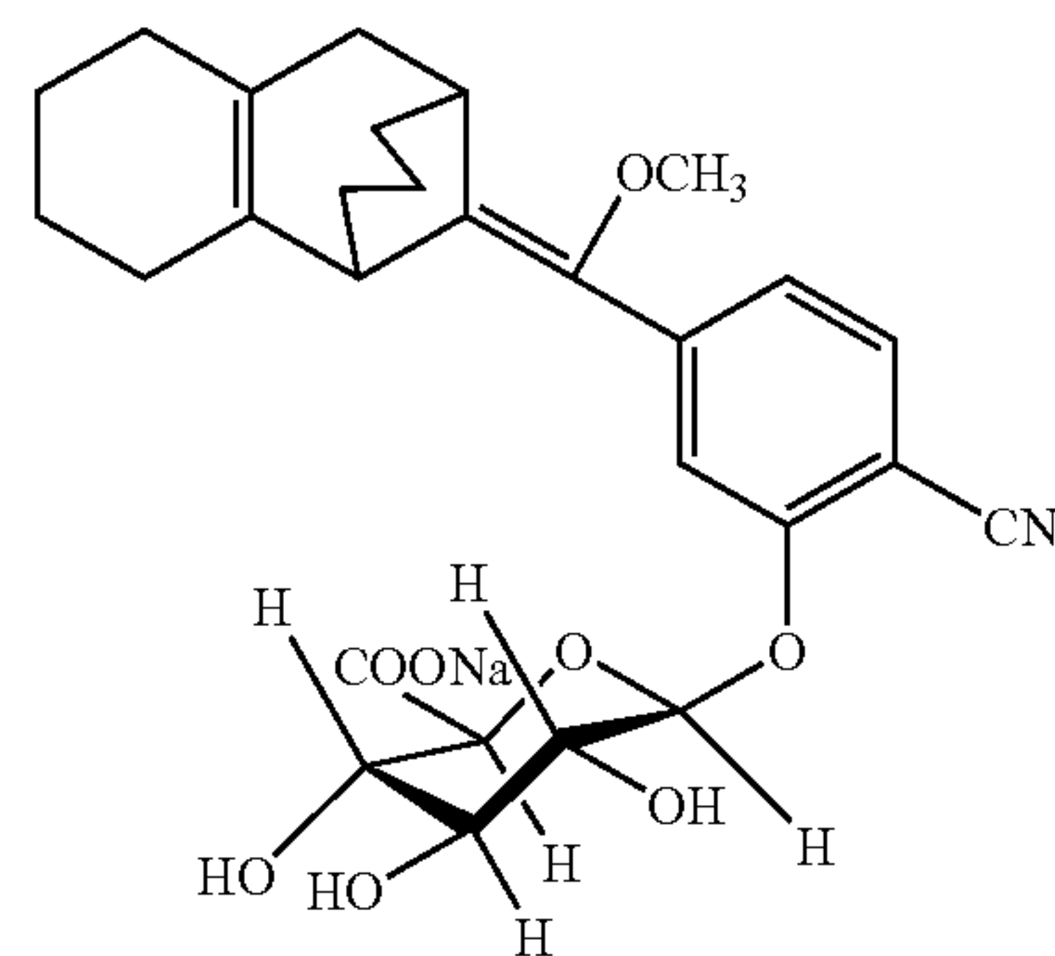
Synthesis of sodium [(4-methoxy-4(3-β-D-glucuronic acid-4-cyanophenyl)]spiro[1,2-dioxetane-3-1,3-tricyclo[7.3.1.0 2,7 ]tridec-2,7-ene
