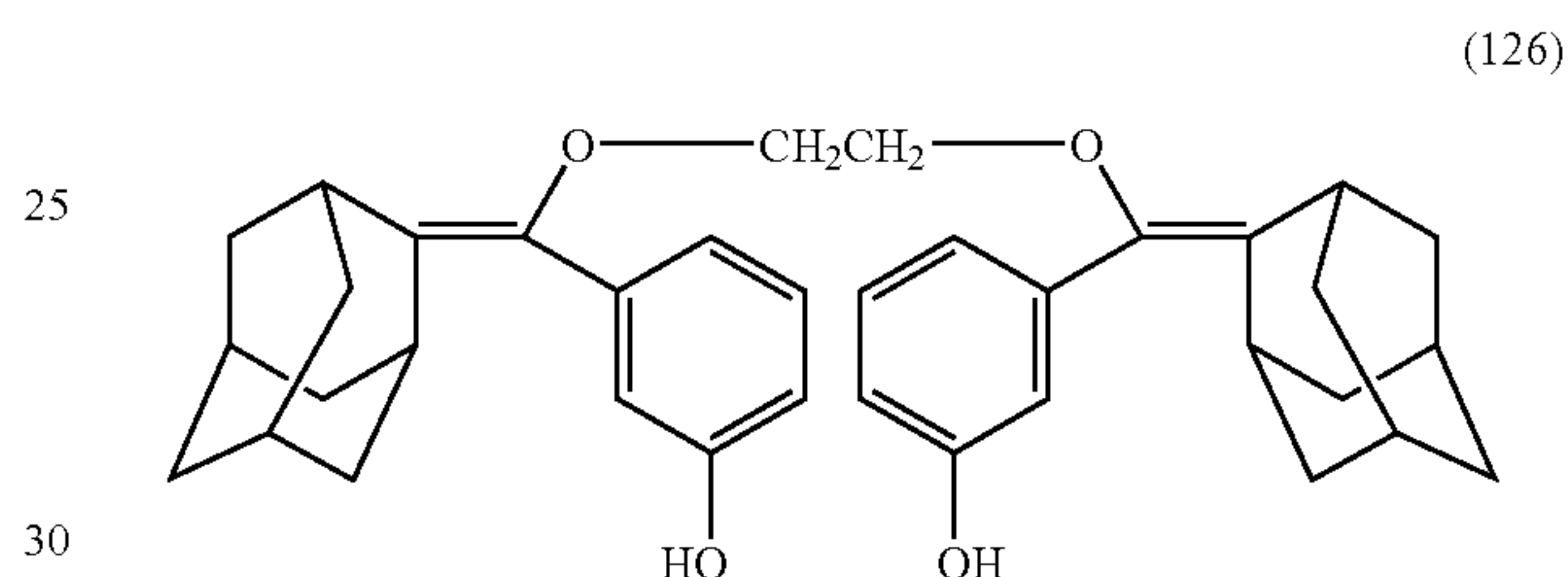
(g). Synthesis of bis[(3-phosphoryloxyphenyl)methylenoxymethylene adamantane, disodium salt]
