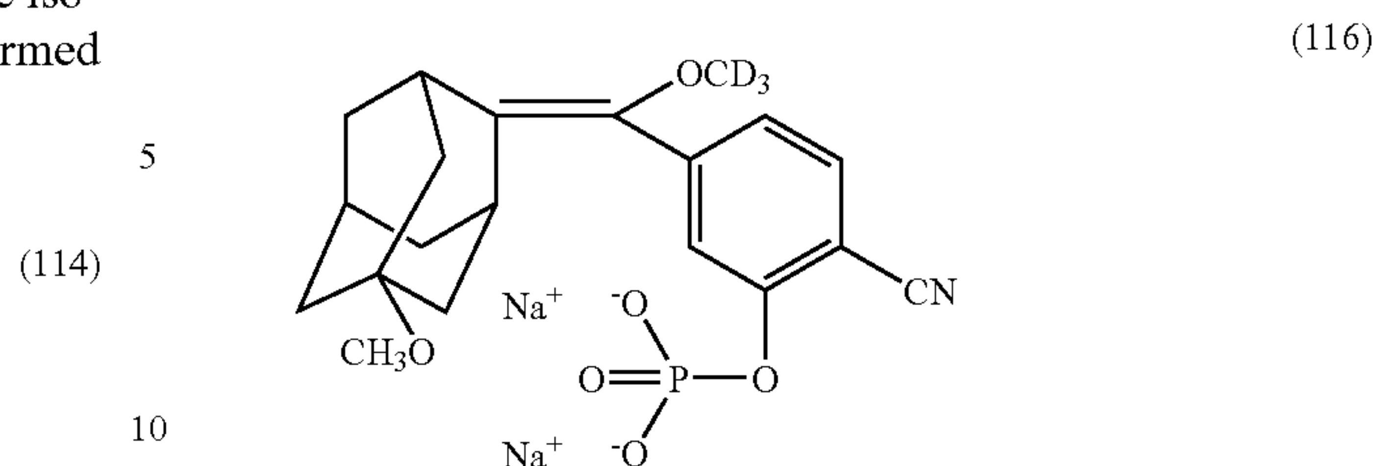
(c). Synthesis of [(4-methoxy (D 3 )-4-(3-phosphoryloxy-4-cyanophenyl)]spiro[1,2-dioxetane-3, 2'-5-methoxyadamantane], disodium salt
