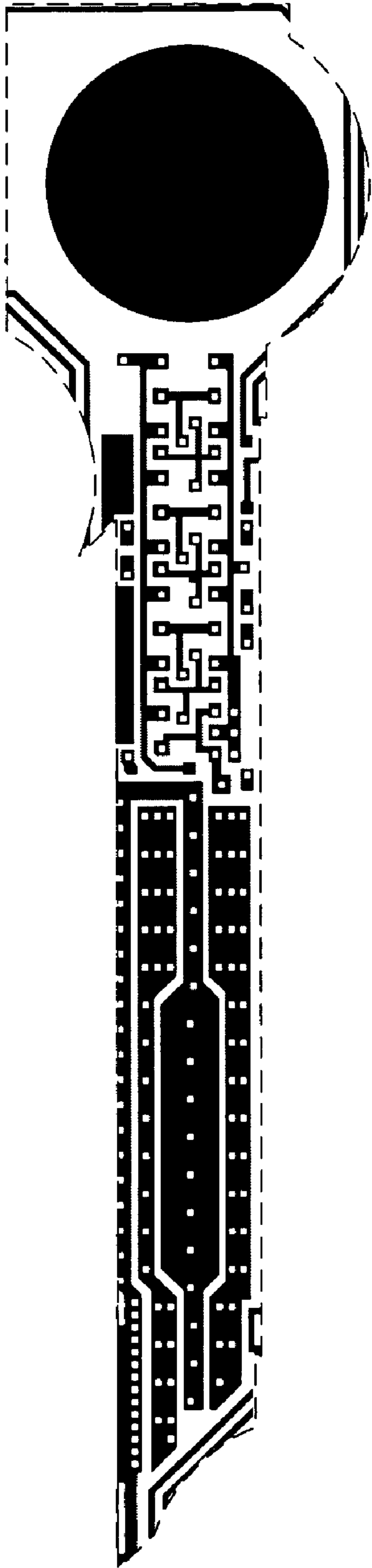
Metal 1 mask
