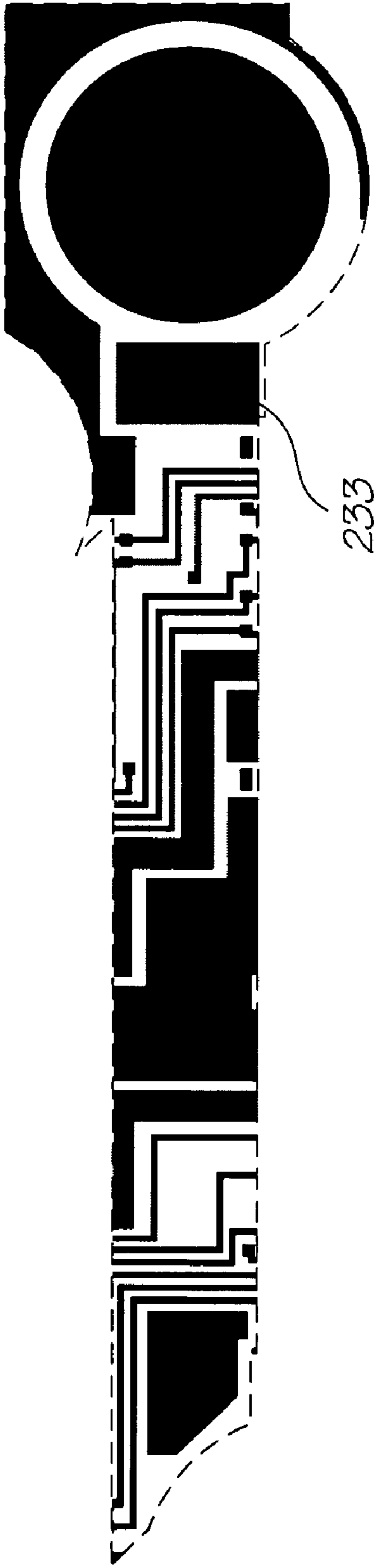
Metal 2 mask
