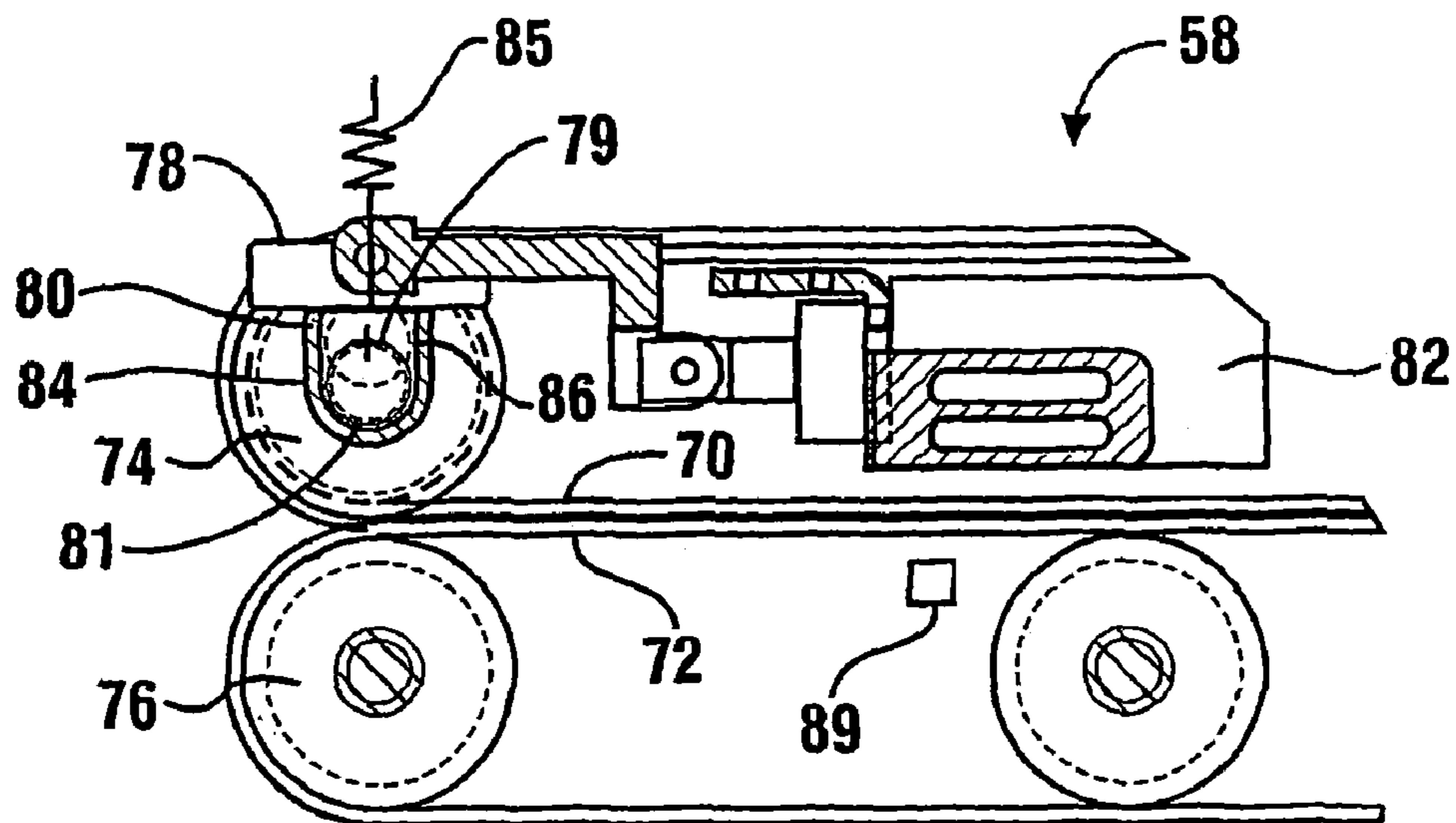
Low Drive Position FIG. 9
