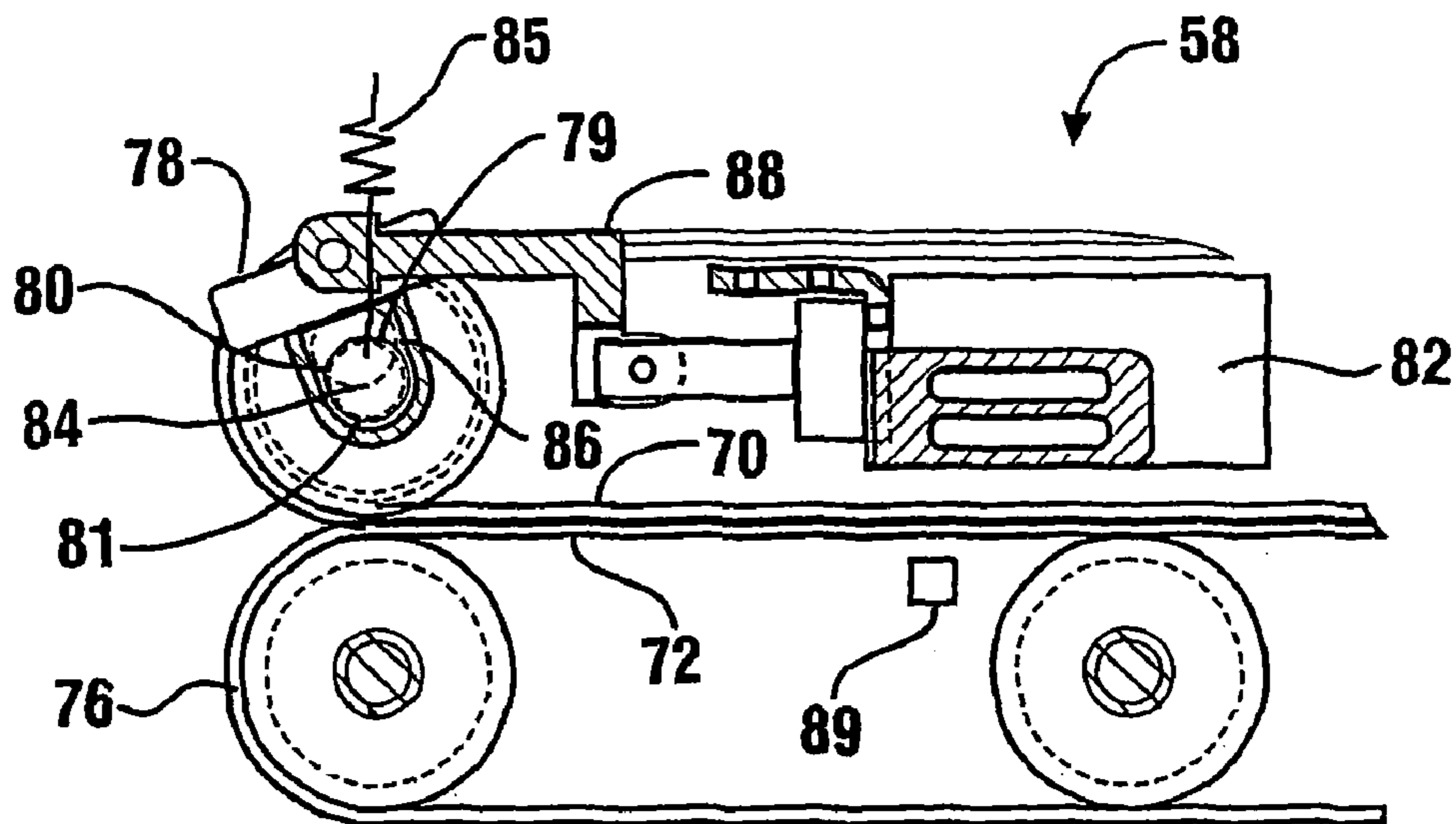
High Drive Position FIG. 10
