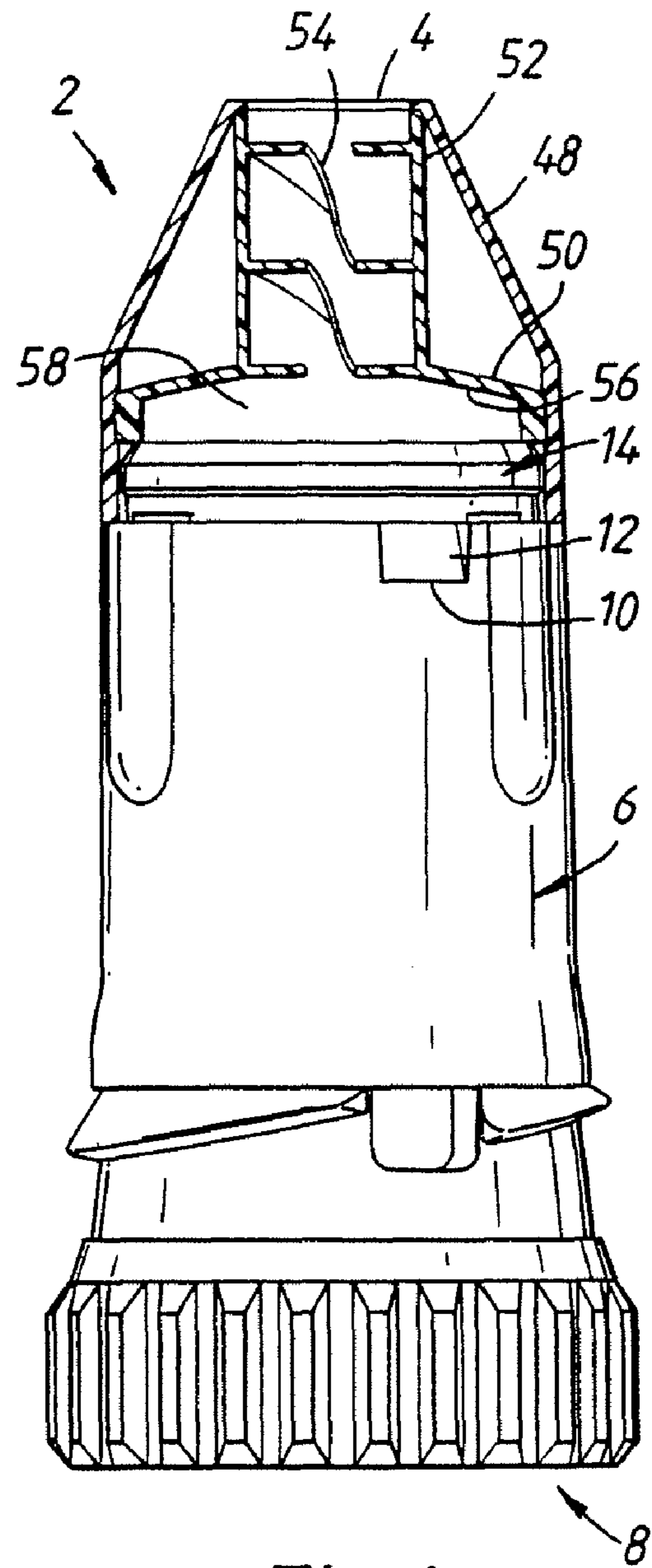
Fig. 4 PRIOR ART
