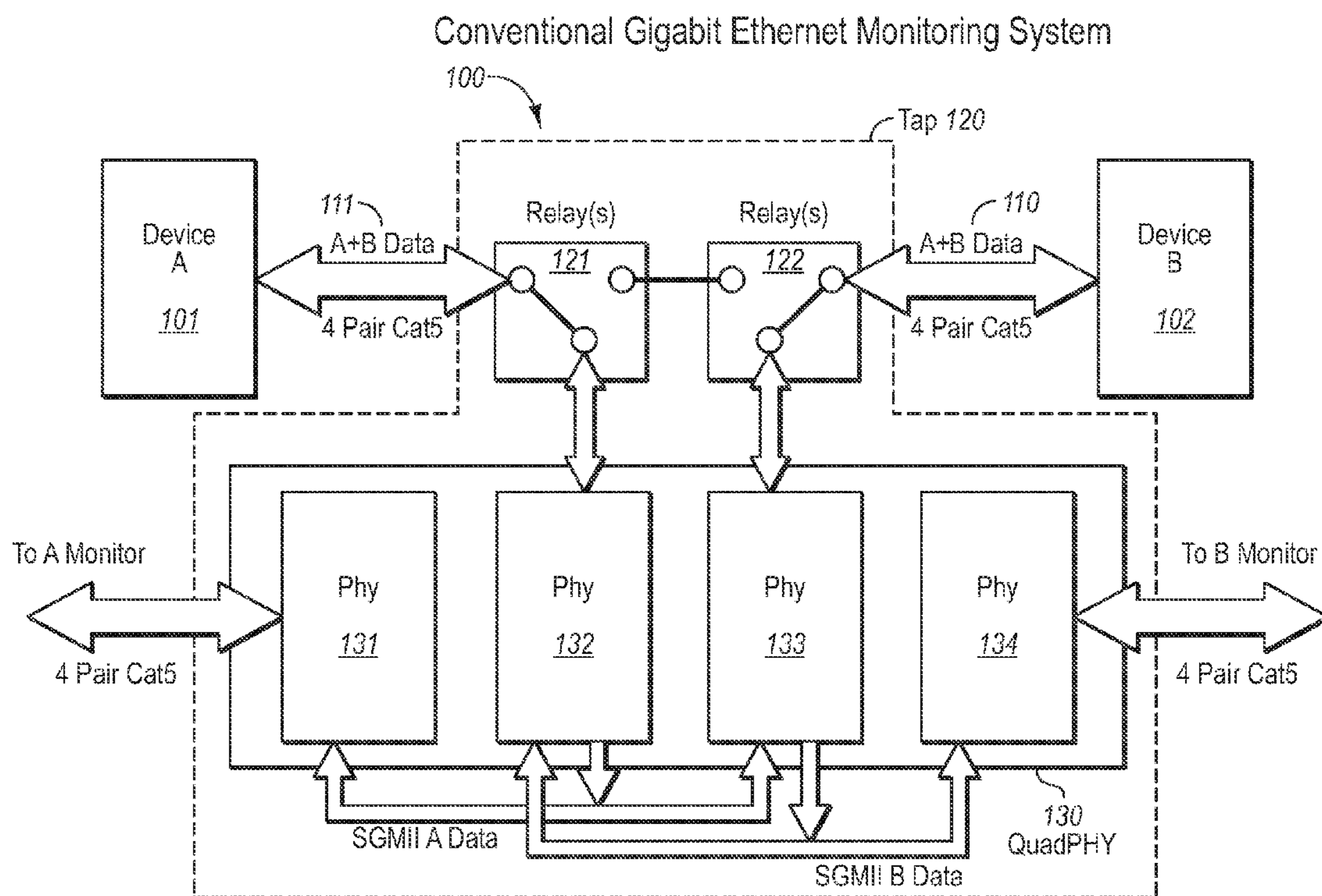
Fig. 1 (Prior Art)
